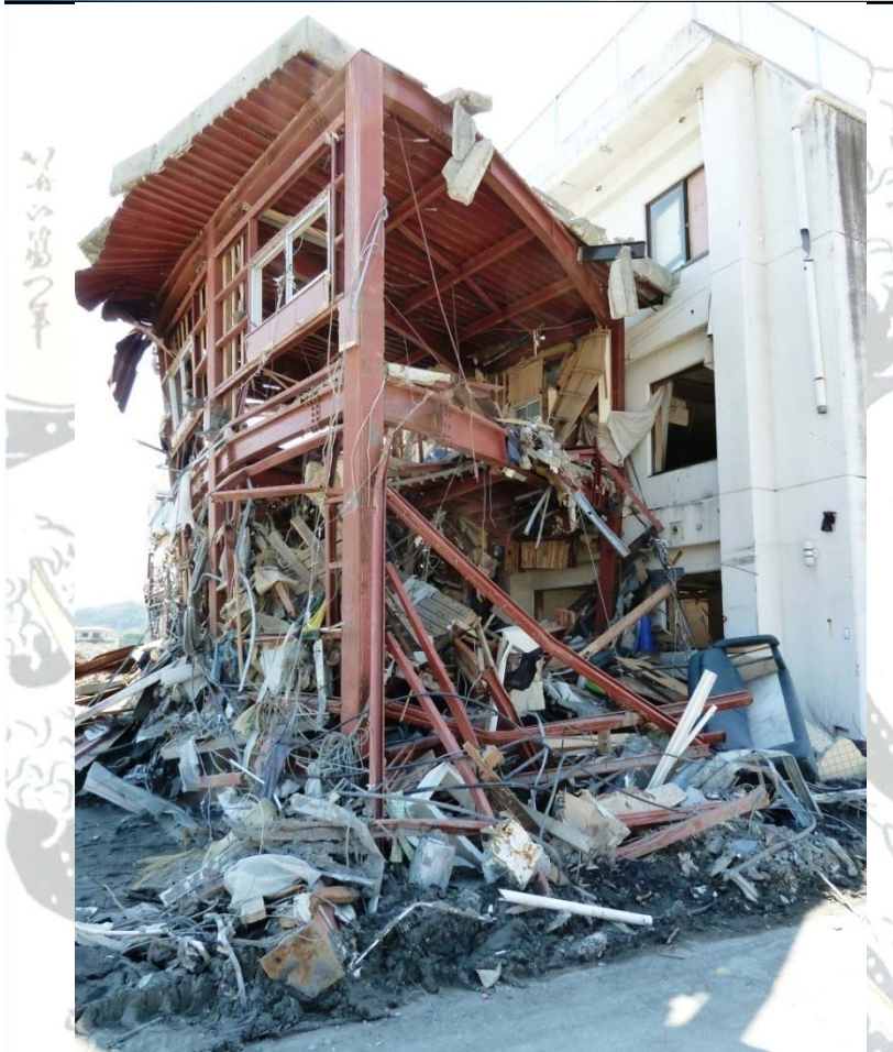
Three-Story SMRF collapsed and pushed into concrete building
