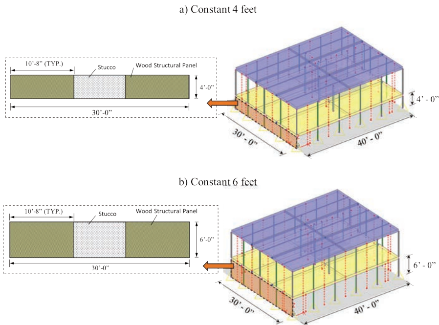
Figure 9-4 Illustration of the two control archetypes on constant height cripple walls used for comparison in the transition study: (a) four-foot cripple wall height; (b) six foot cripple wall height. Wood structural panels assume 8d common nails at 4 inches on center.
