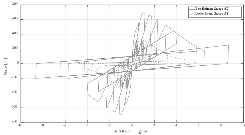
Figure 11-12 Assumed hysteretic behavior for best estimate stucco (solid line) and lower bound stucco (dashed line).
