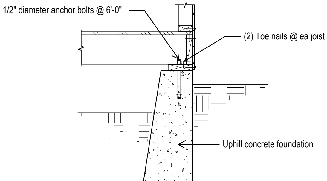
Figure 13A-7 Existing uphill foundation section
