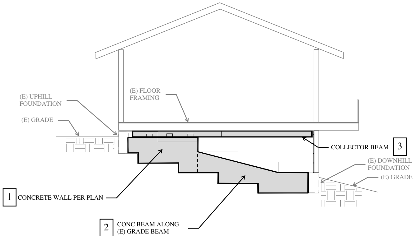
Fig 13A-17 Example dwelling elevation showing primary members
