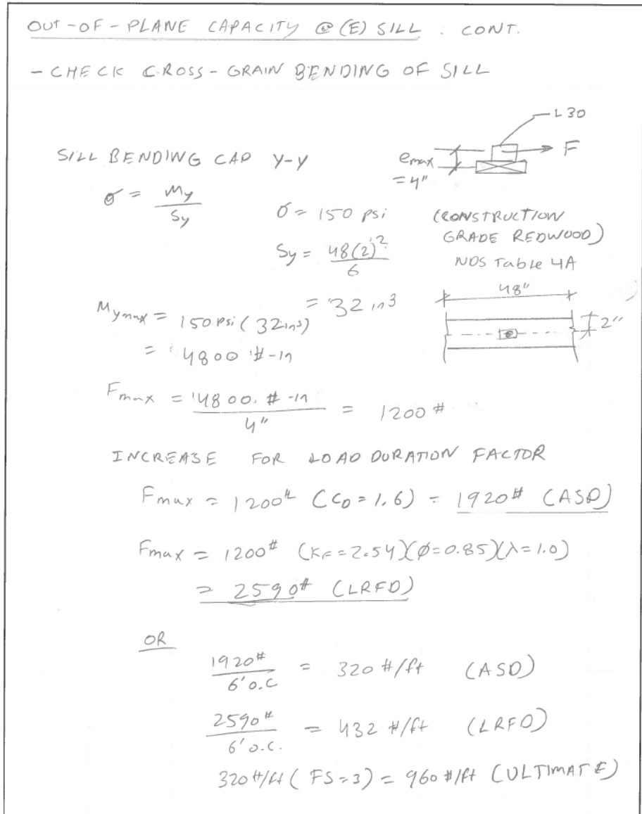
Figure 9-19 Page two of calculations for out-of-plane resistance at uphill wall line: check for cross grain bending of sill.
