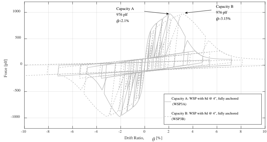
Figure 11-18 Comparison of wood structural panel displacement capacity based on cripple wall height: Capacity A (solid line) for cripple walls taller than 5 feet; Capacity B (dashed line) for cripple walls with a height of 5 feet or less.
