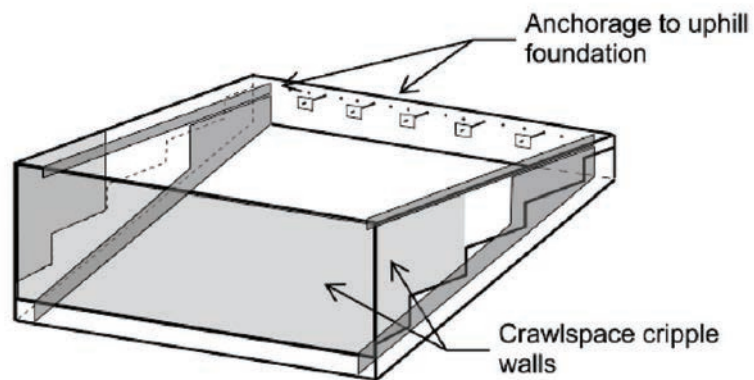
Figure 13-2 Hillside dwelling schematic illustration of the underfloor area enclosed with sheathed side walls.
