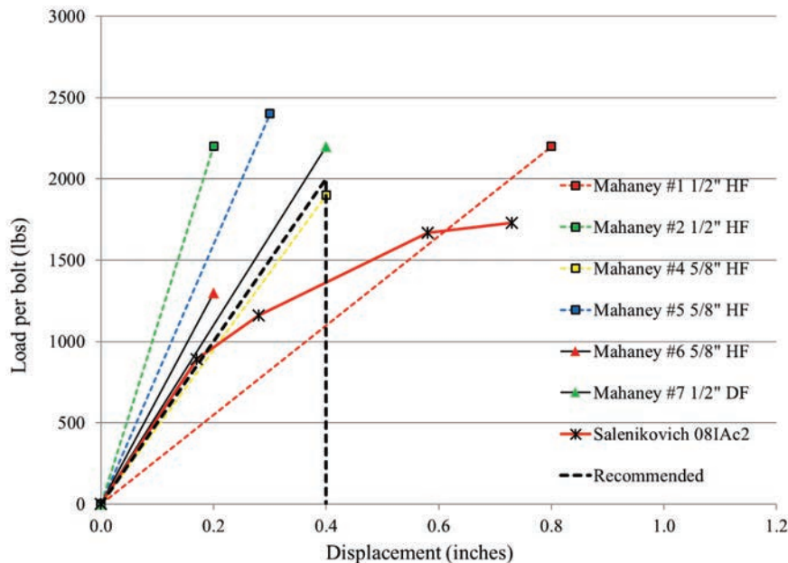
Figure 4-13 Plot of applicable test data and load-deflection behavior for anchorage out-of-plane.
