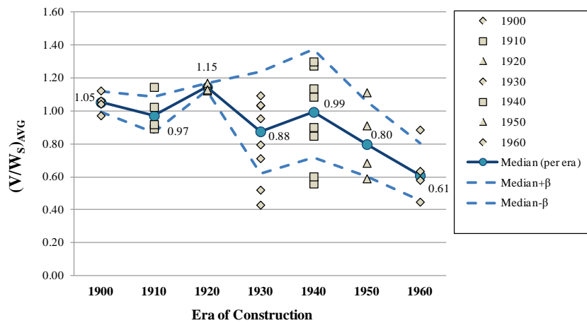
Figure 6-27 Strength-to-seismic weight ratios for the bottom story of two-story configurations.
