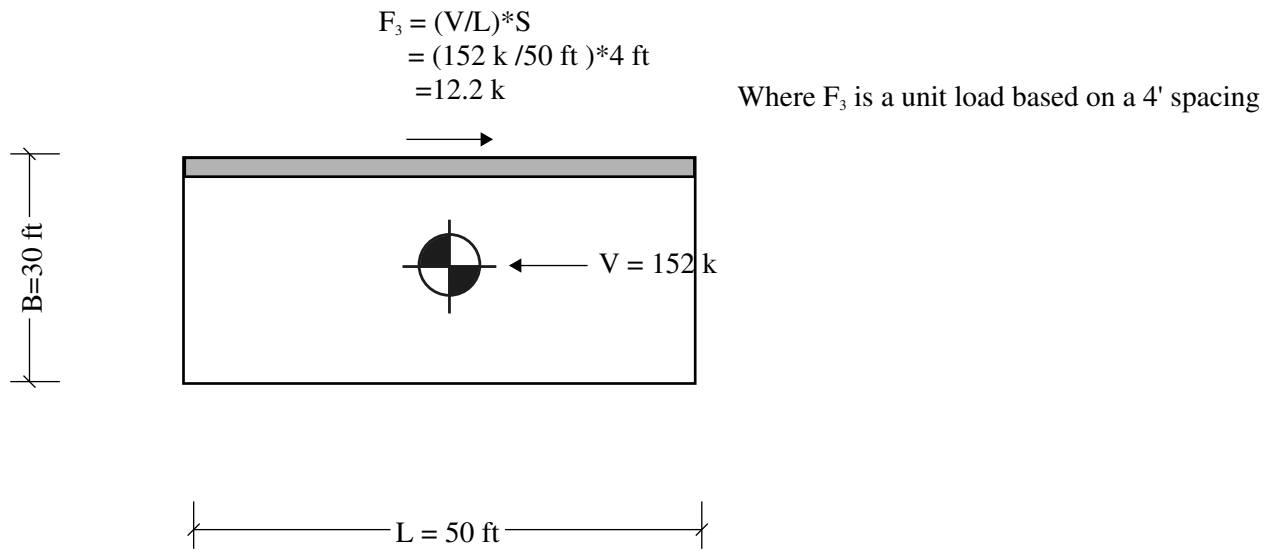
Figure 13A-14 Shear anchor configuration
