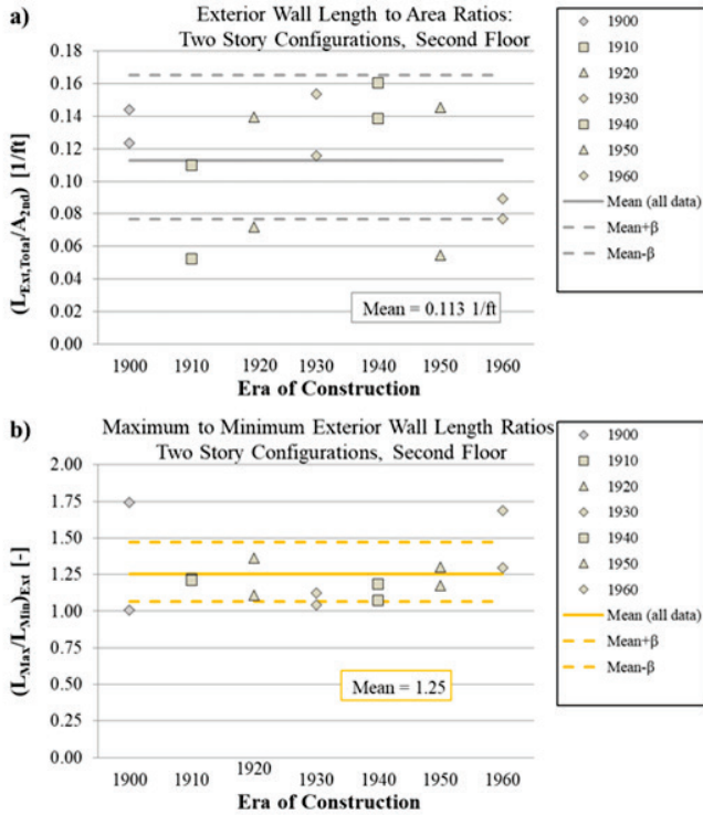
Figure 6-11 Exterior criteria for the second floor of two-story configurations: (a) Exterior wall density, (b) Maximum-to-minimum length ratio.
