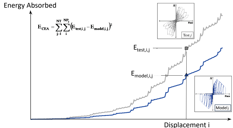
Figure 4-20 Illustration of procedure to extract CUREE hysteretic parameters based on equal cumulative energy absorbed.
