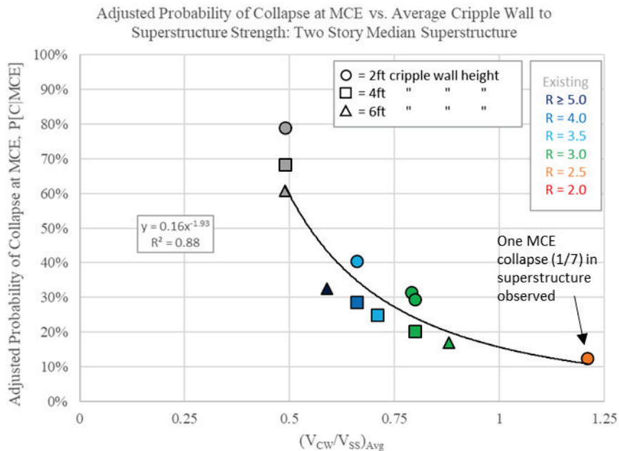
Figure 11-25 Trends of probability of collapse at the MCE intensity level versus the average cripple wall to superstructure strength ratio: Two-story median pre-1950 superstructure.
