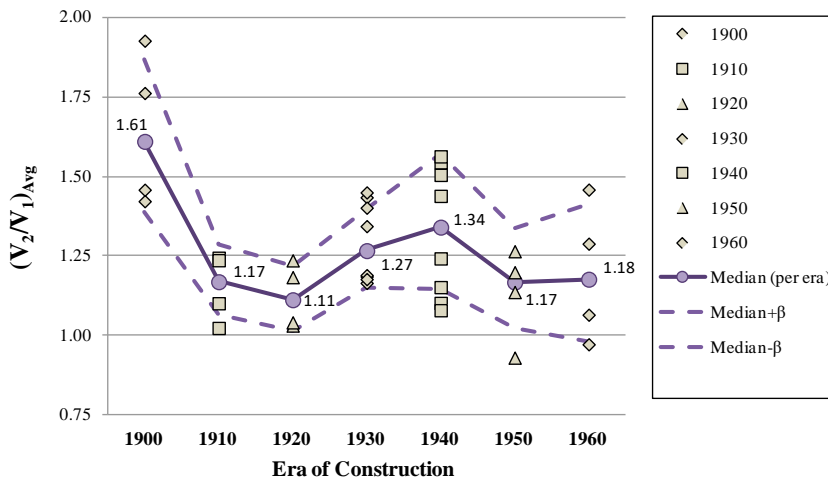
Figure 6-26 First-to-second-story strength ratios for two-story configurations.
