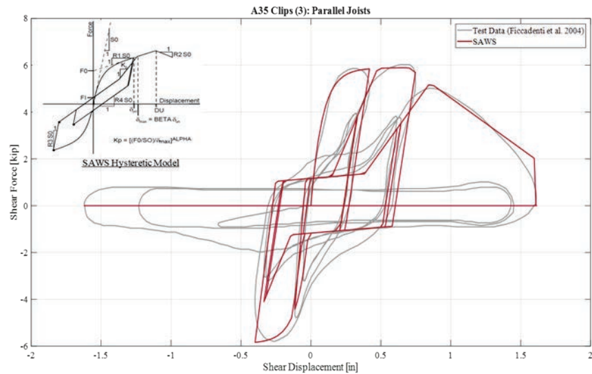
Figure 4-35 Fitting of SAWS hysteretic model to A35 clip testing conducted by Ficcadenti et al. (2004). NOTE: The test shown is for three clips in parallel.
