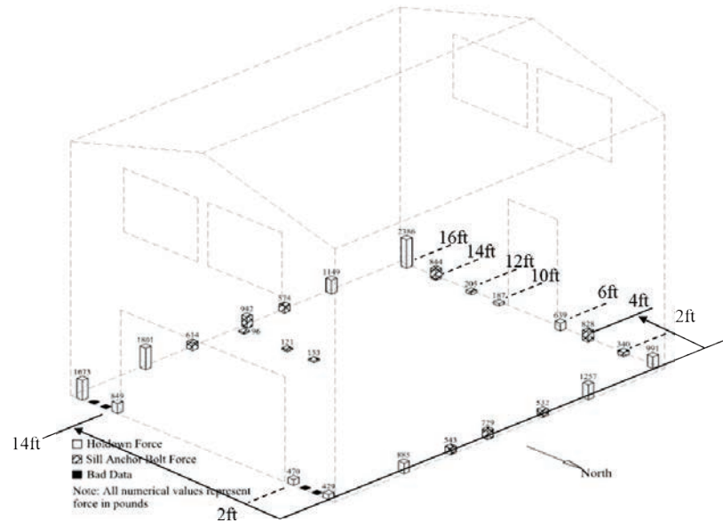
Figure 8-4 Assumed locations of anchor bolts and hold-downs for calculation of overturning moments from shake table testing by Fisher et al. (2001; 2002) (Locations for phases 9 and 10 shown).
