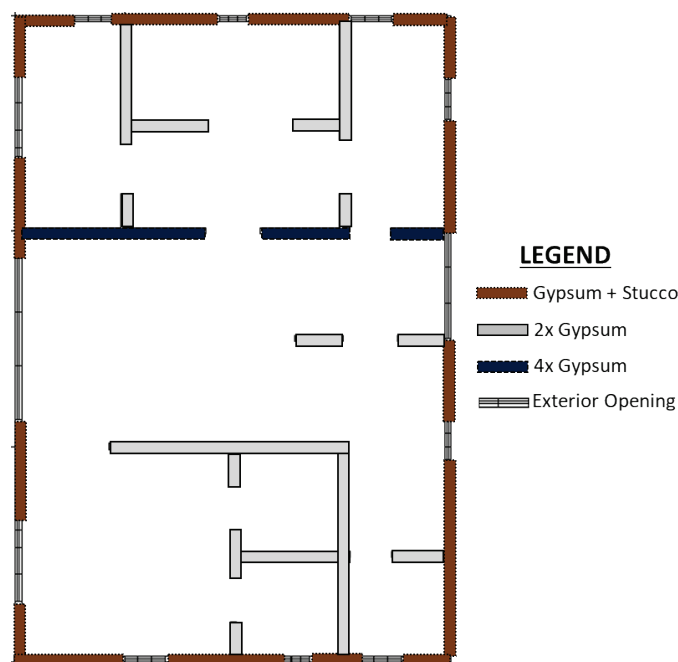
Figure 13-20 Simplified floor plan for modeling purposes. Used for all models except Model 6-1H016-M-R=M1R.
