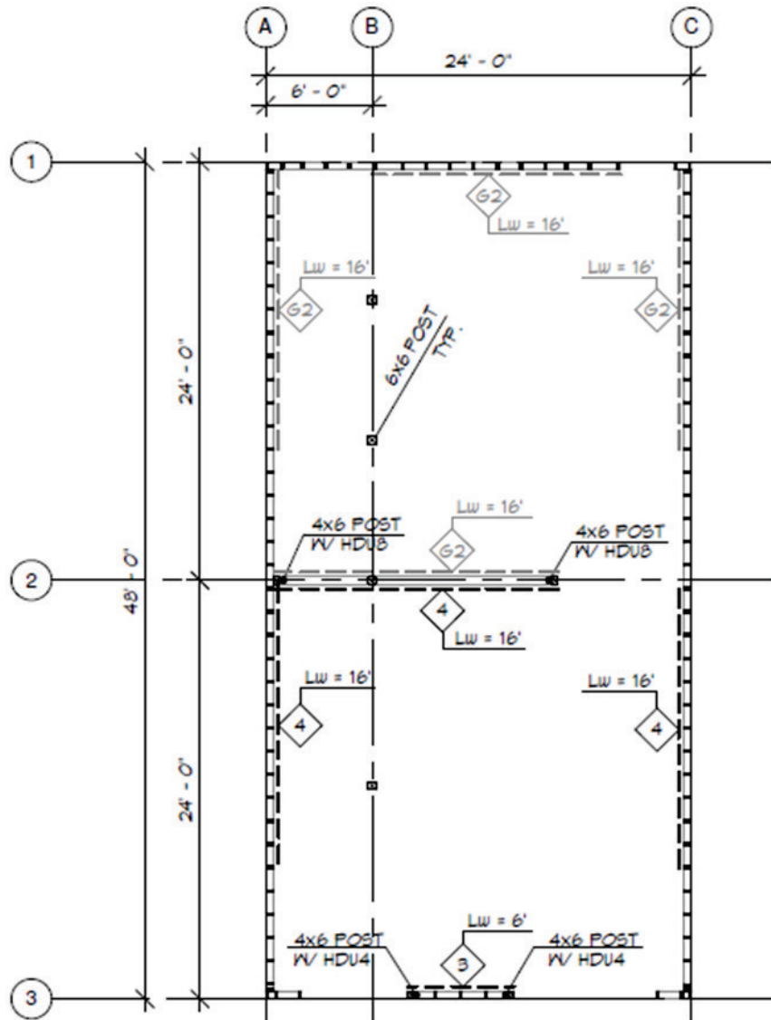
Figure 12-5 First floor plan view of house-over-garage with living space at the ground floor.
