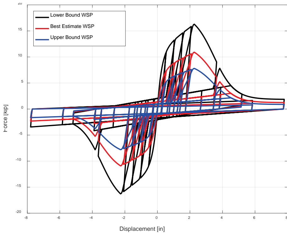
Figure 12-16 Hysteretic parameters for wood structural panels (WSP1, WSP2, and WSP3).
