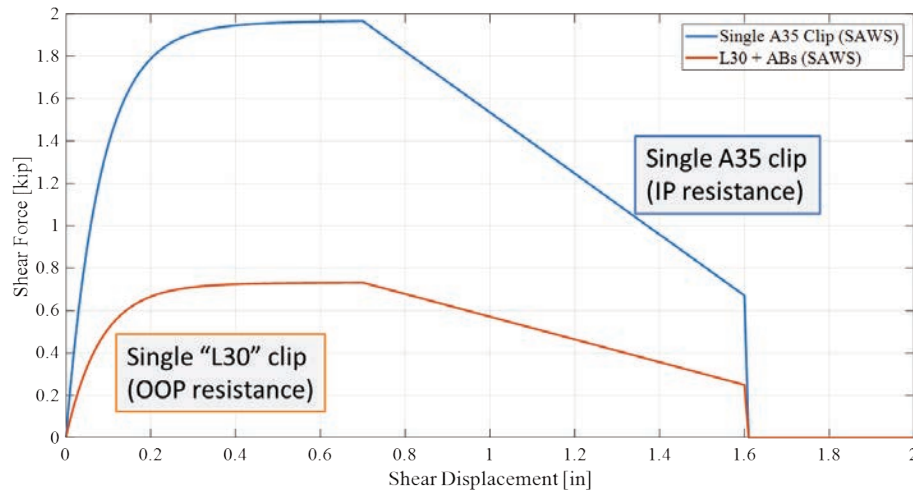
Figure 9-8 Assumed material backbones for in-plane (IP) and out-of-plane (OOP) resistance at the retrofit joist-to-sill connection at the uphill wall line of sloped cripple wall with a zero-height condition.
