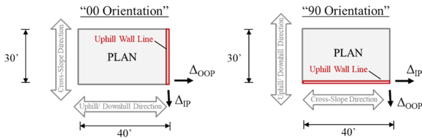
Figure 9-5 Illustration of the two orientations of the uphill wall line considered for transition study archetypes. In-plane (IP) and out-of-plane (OOP) displacements are annotated with respect to the uphill wall line.
