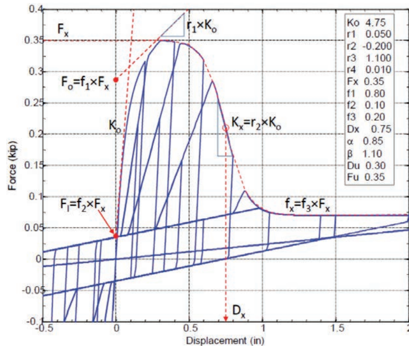
Figure 1-2 Modification of CUREE hysteretic rule for modeling residual strength.
