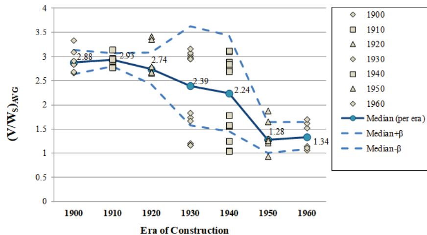
Figure 6-14 Sample of configuration data collected across different eras of construction showing the average superstructure strength to seismic weight ratios for all one-story configurations.
