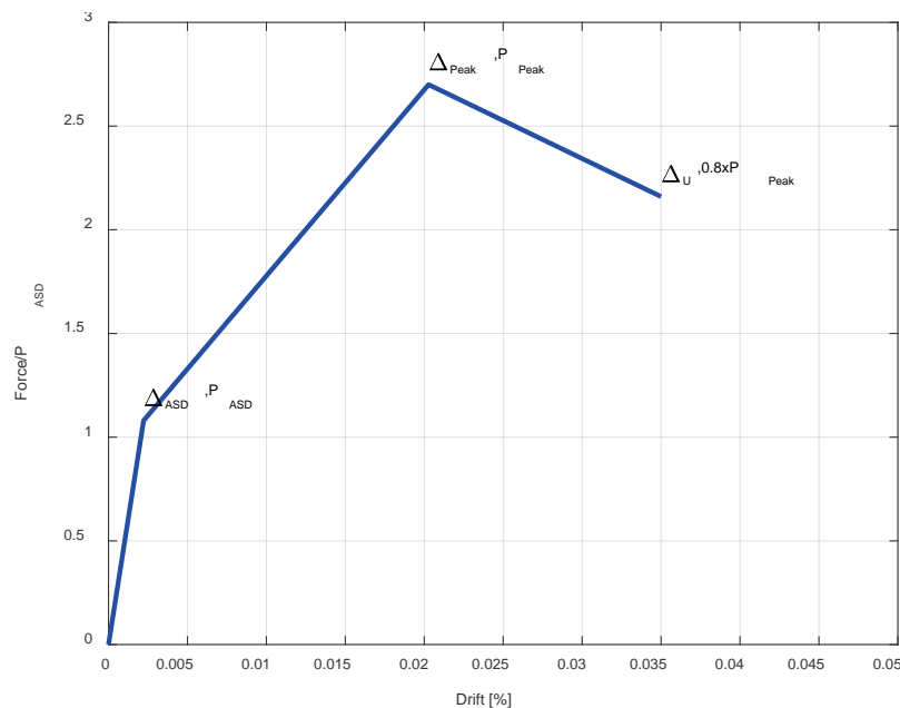
Figure 12-22 Points used for backbone of proprietary wall systems based on ICC acceptance criteria.
