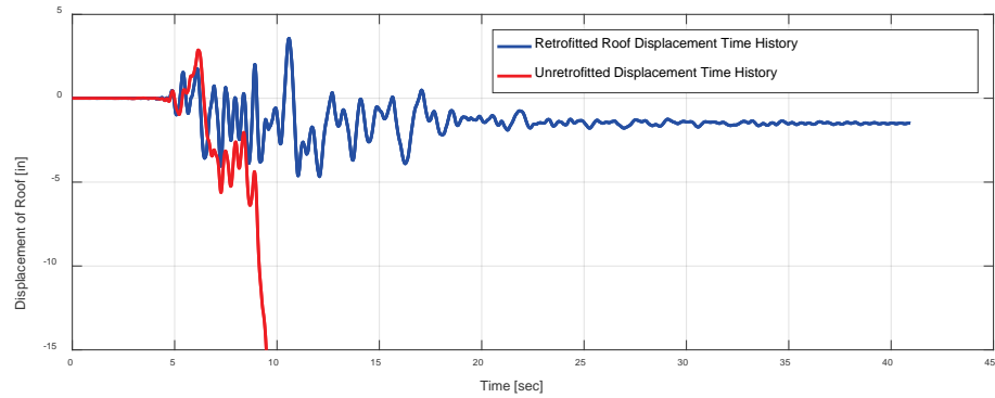
Figure 12-26 Lateral displacement time history of control roof node for retrofitted and un-retrofitted configuration of HOG3.
