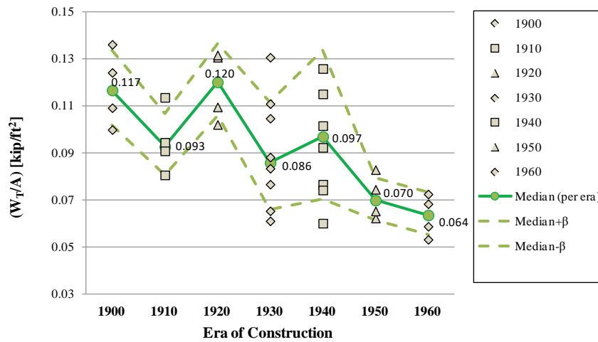
Figure 6-23 Total weight-to-plan area ratios for two-story configurations.
