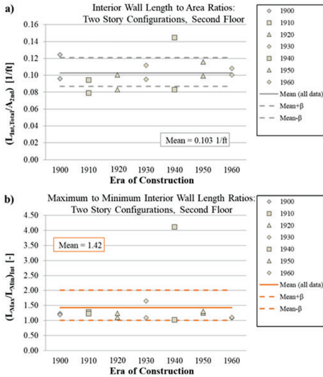
Figure 6-12 Interior criteria for the second floor of two-story configurations: (a) Interior wall density, (b) Maximum-to-minimum length ratio.
