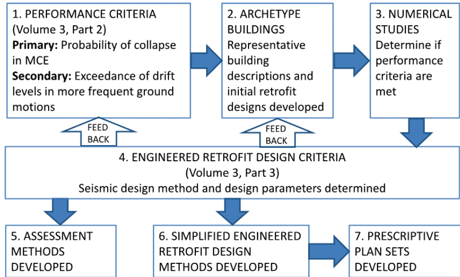
Figure 3-1 Relating numerical study performance criteria to retrofit criteria.
