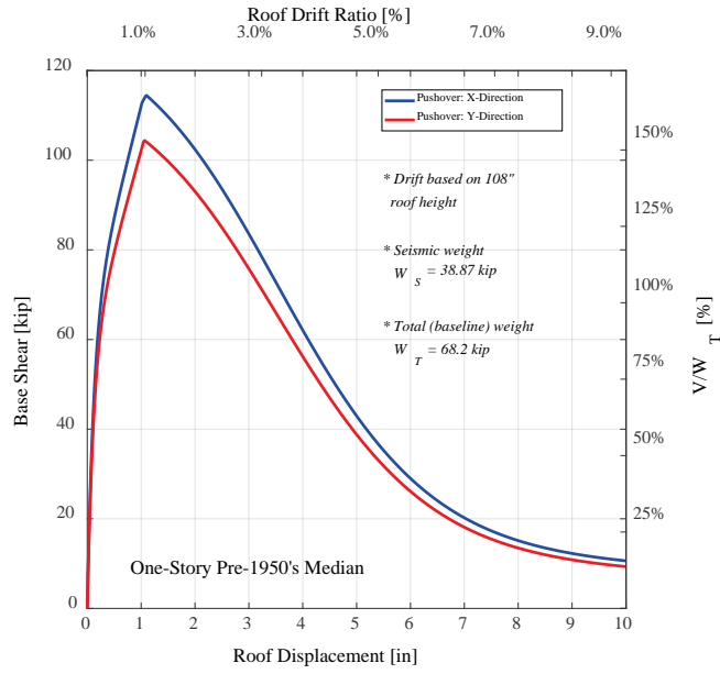
Figure 6-37 Pushover curves for the one-story pre-1950's Median Superstructure (Archetype 4-1R-M-E).
