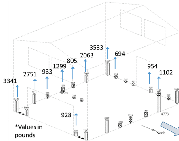
Figure 8-8 Example of anchorage elements assumed in tension for north loading: Test 9.S.4 (figure adapted from Fischer et al. (2001; 2002)).
