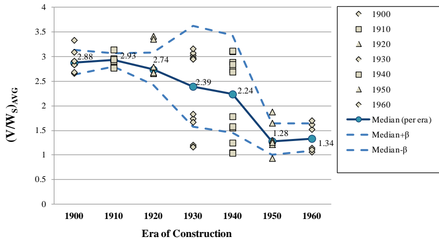
Figure 11-3 Sample of configuration data collected across different eras of construction showing the average superstructure strength to seismic weight ratios for all one-story configurations.
