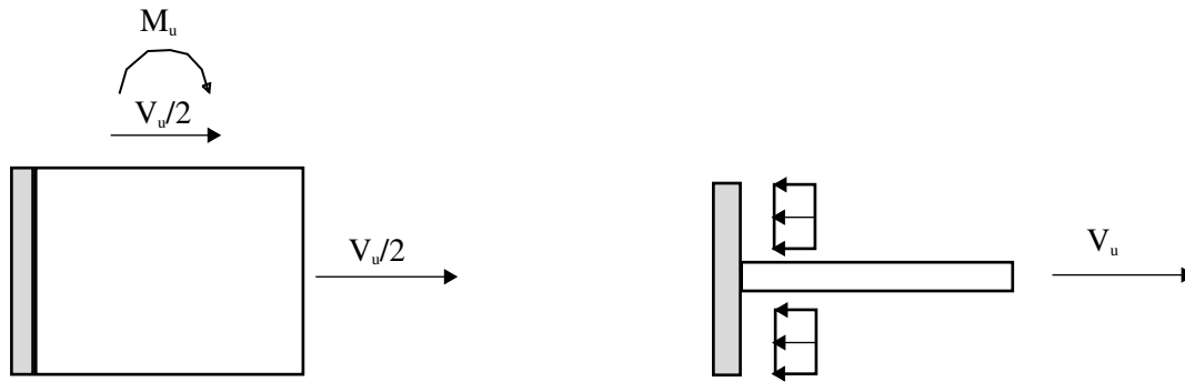
Saddle Connection Elevation
