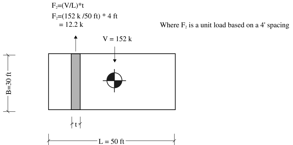
Figure 13A-13 Secondary anchor configuration
