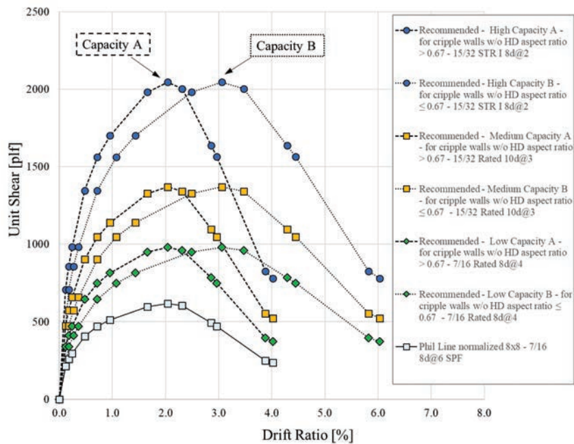
Figure 4-10 Plot of applicable test data and approximate backbone for wood structural panel shear walls with intermediate anchorage.
