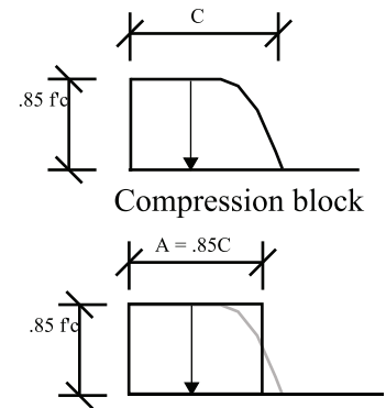
Figure 13A-20 Assumed compression block
