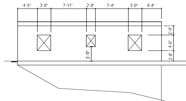
Figure 13-5 Dwelling elevation—side.
