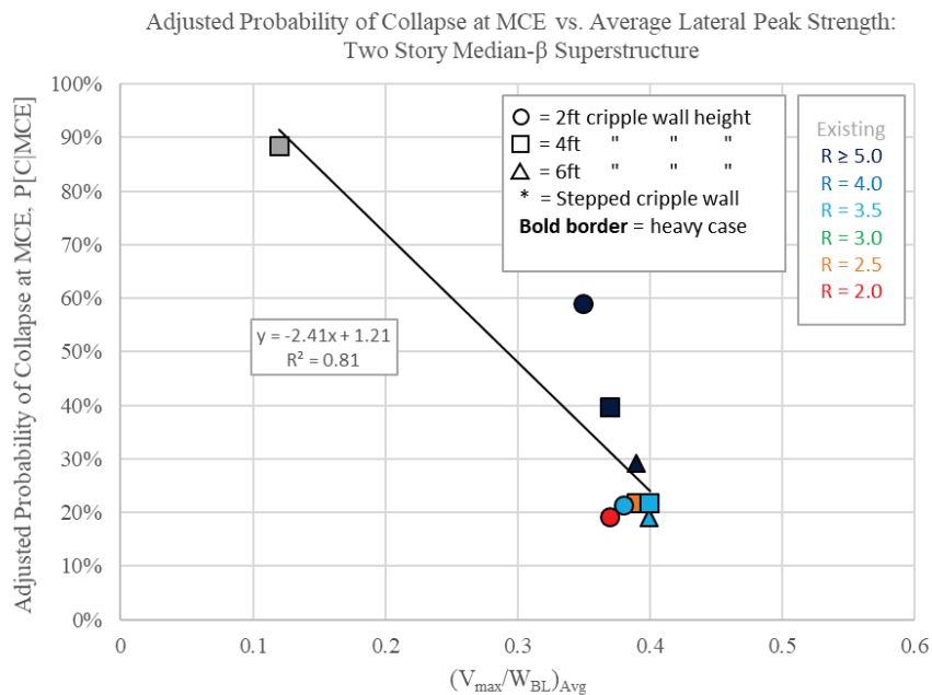
Figure 11-26 Trends of probability of collapse at the MCE intensity level versus the average peak strength-to-baseline weight ratio: Two-story median- \beta post-1950 superstructure. Note: Global strength controlled by superstructure strength for R < 4 . Saturation of points near (V/W)_{Avg} = 0.4 reflects global collapses occurring in superstructure.
