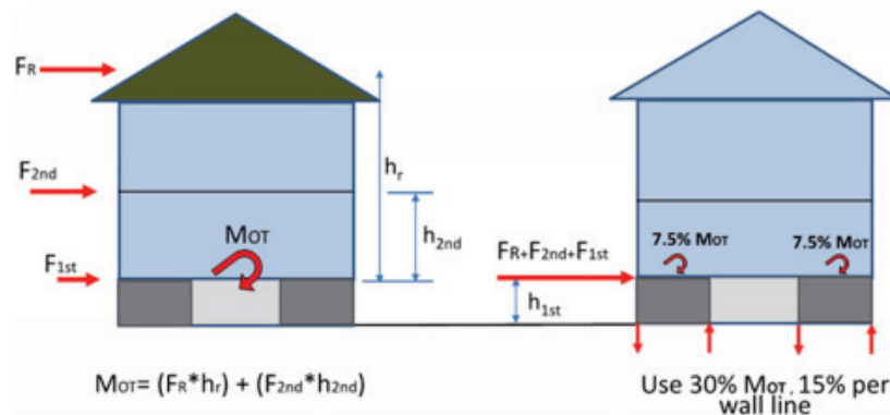
Figure 8-1 Illustration of simplified overturning assumptions for the design of cripple wall retrofit.
