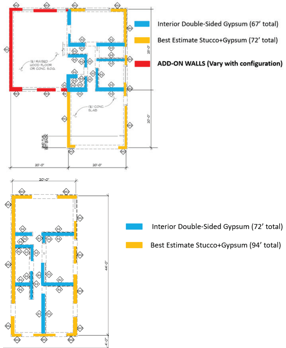
Figure 12-11 Typical existing wall layouts for ROG configurations.
