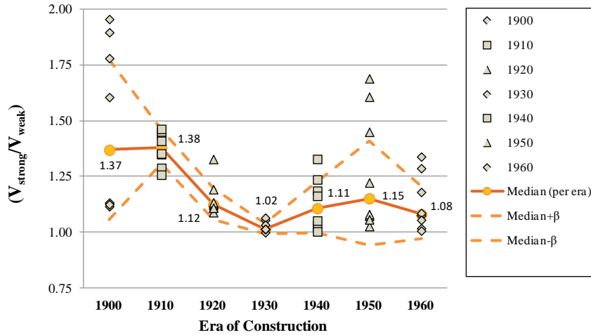
Figure 6-25 Strong-to-weak direction strength ratios for the bottom story of two-story configurations.
