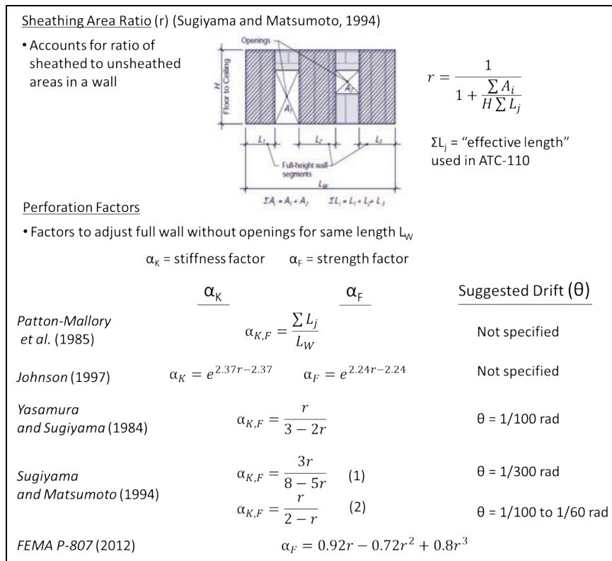
Figure 4-16 Illustration of different perforation factors to account for strength and stiffness reduction due to openings in exterior wall lines. Note: these relationships are developed based on testing of wood structural panel shear walls and intended for similar application.
