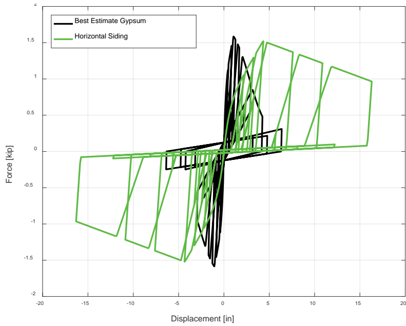
Figure 12-15 Hysteretic parameters for gypsum and horizontal siding.
