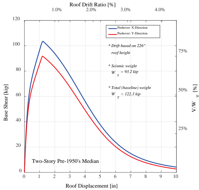
Figure 6-38 Pushover curves for the two-story pre-1950's Median Superstructure (Archetype 4-2R-M-E).
