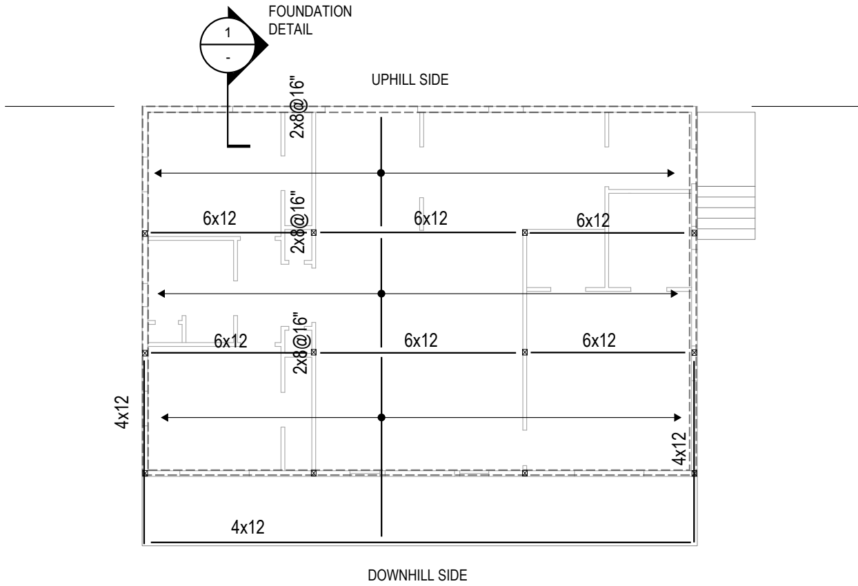
Figure 13A-4 First floor framing plan
