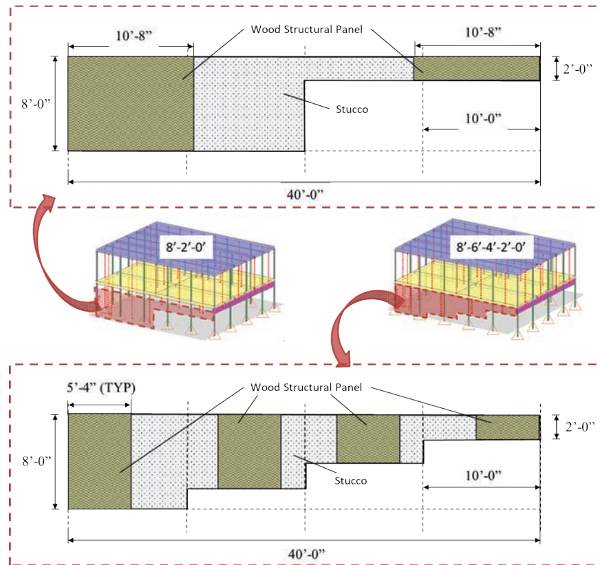
Figure 9-6 Illustration of the two variations of sloped cripple walls with a maximum downhill height of eight feet: Case 8’-2’0’ with large single transition height (above), Case 8’-6’-4’-2’-0’ with evenly distributed height transition (below).
