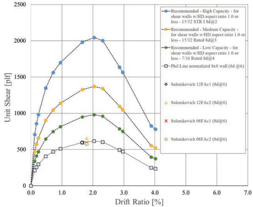
Figure 4-29 Test data and recommended backbone curves for wood structural panels with tie downs.
