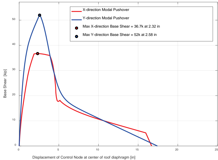
Figure 12-25 Non-linear static pushover analysis for 5-HOG3-H-5SW.
