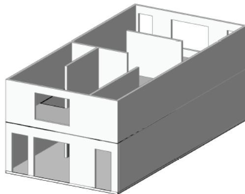
Figure 12-9 Rendering of typical HOG configuration with garage door opening.
