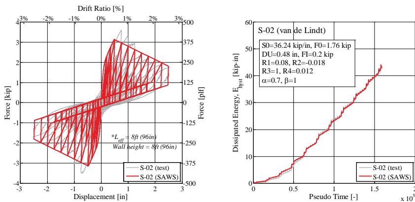
Figure 4-26 Comparison of hysteretic response and cumulative dissipated energy for test data (Test S-02 from Bahmani and van de Lindt, 2014) and optimized CUREE parameters (see Table 4-7) for walls sheathed with lower bound stucco.
