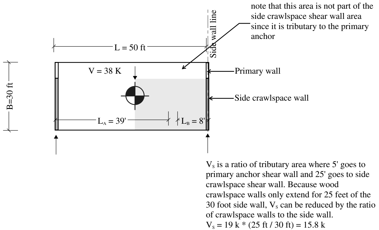
Figure 13A-16 Side crawlspace wall configuration
