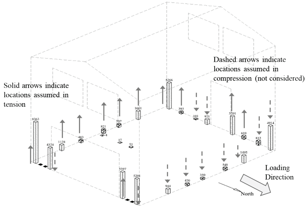
Figure 8-8 Example of anchorage elements assumed in tension for north loading: Test 9.S.4 (figure adapted from Fischer et al. (2001; 2002)).
