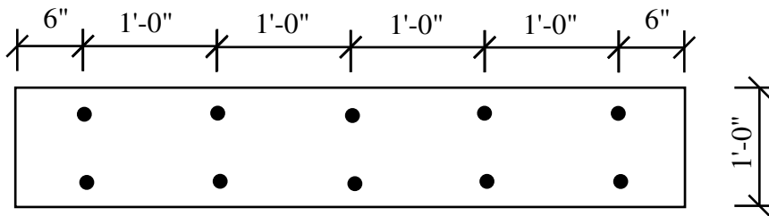
Concrete wall plan view
