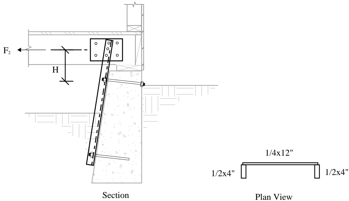
Figure 13A-32 Secondary anchor
