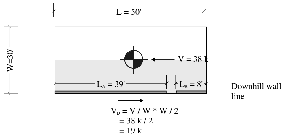
Figure 13A-42 Downhill crawspace wall force diagram
