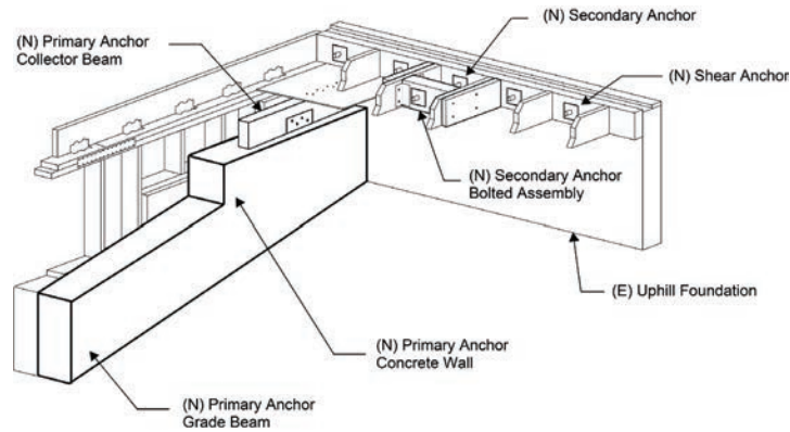
Figure 13-9 Hillside dwelling schematic illustration of retrofit elements.
