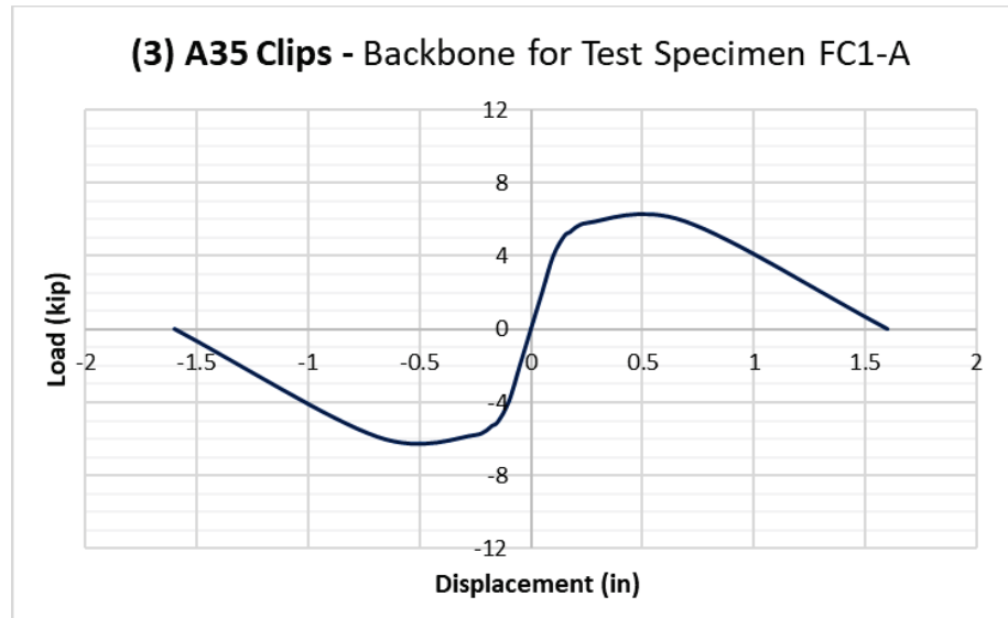
Figure 4-15 Backbone curve for Test Specimen FC1-A of cyclic response of shear transfer connections between shearwalls and diaphragms in woodframe construction (Ficcadenti et. al, 2004).
