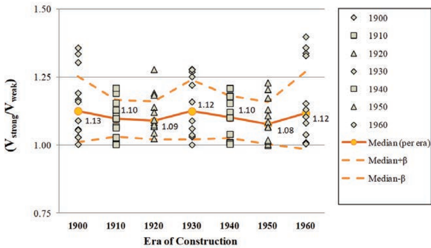
Figure 6-20 Strong-to-weak direction strength ratios for one-story configurations.
