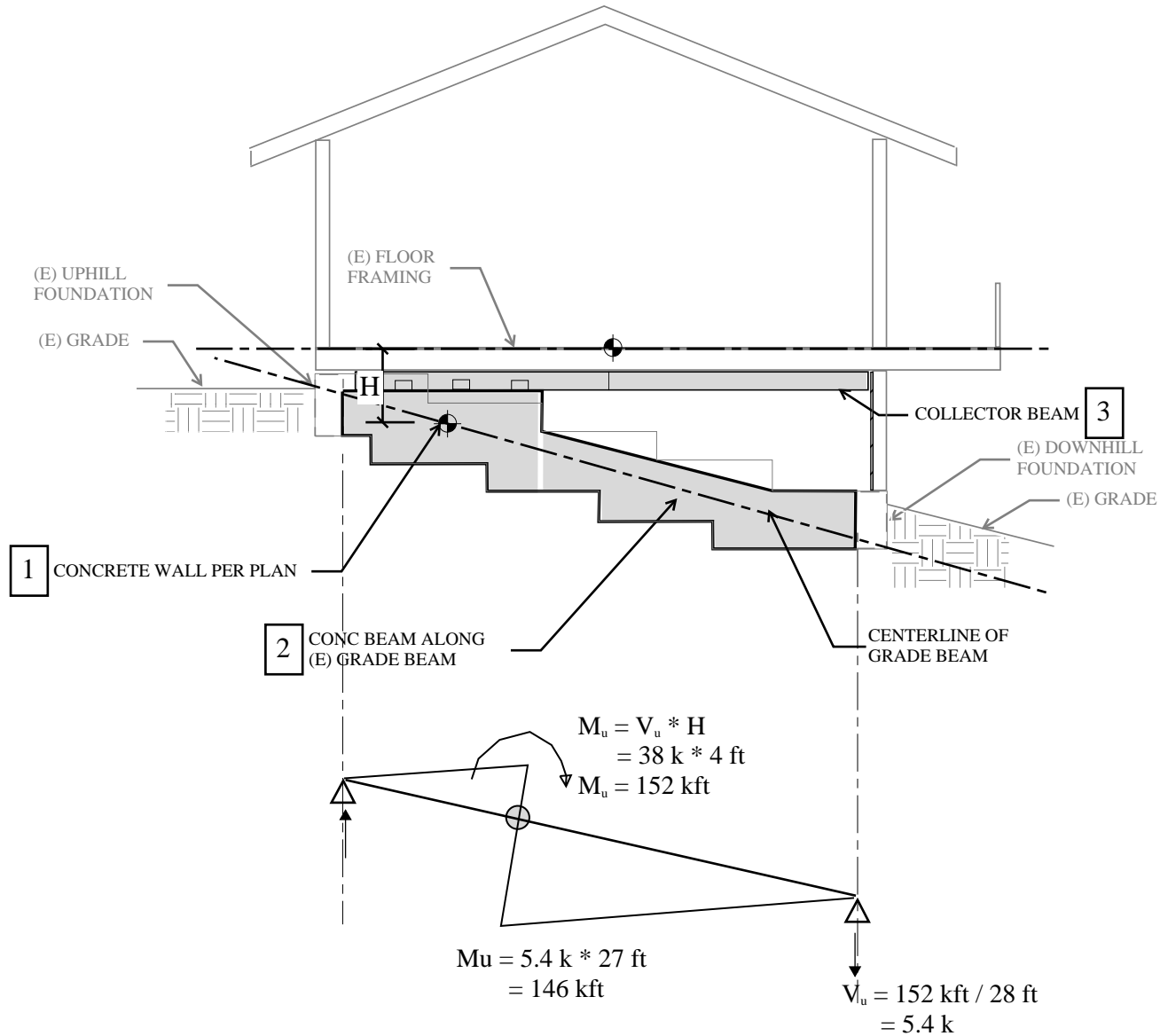
Figure 13A-21 Grade Beam
