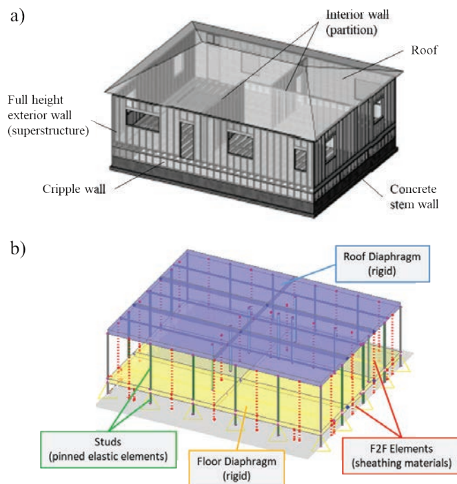
Figure 11-14 Illustration of the basic modelling components of a cripple wall dwelling: a) Rendering and components of one-story house with two-foot tall cripple walls; b) Equivalent model in Timber3D .
