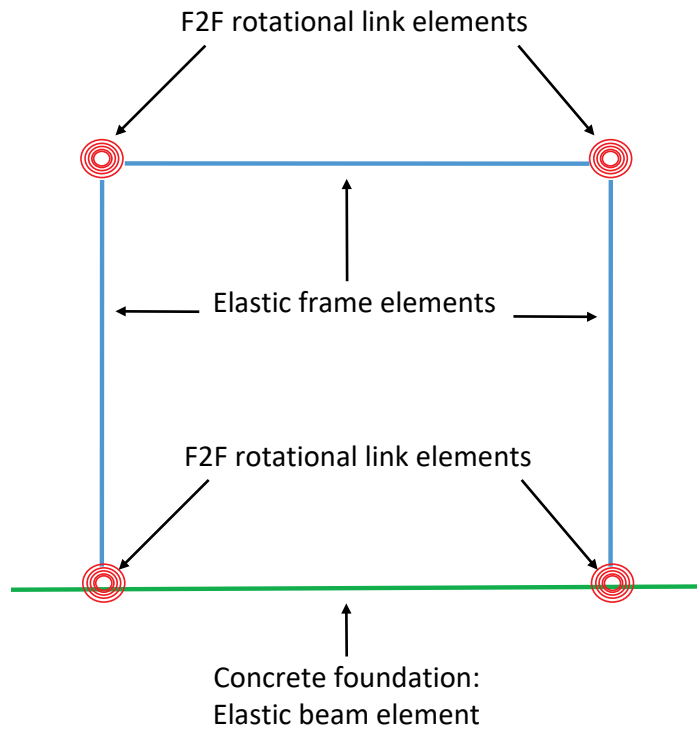
Figure 1-11 Schematic illustration of modeling of an inelastic moment-resisting frame rigidly anchored to an elastic concrete foundation.
