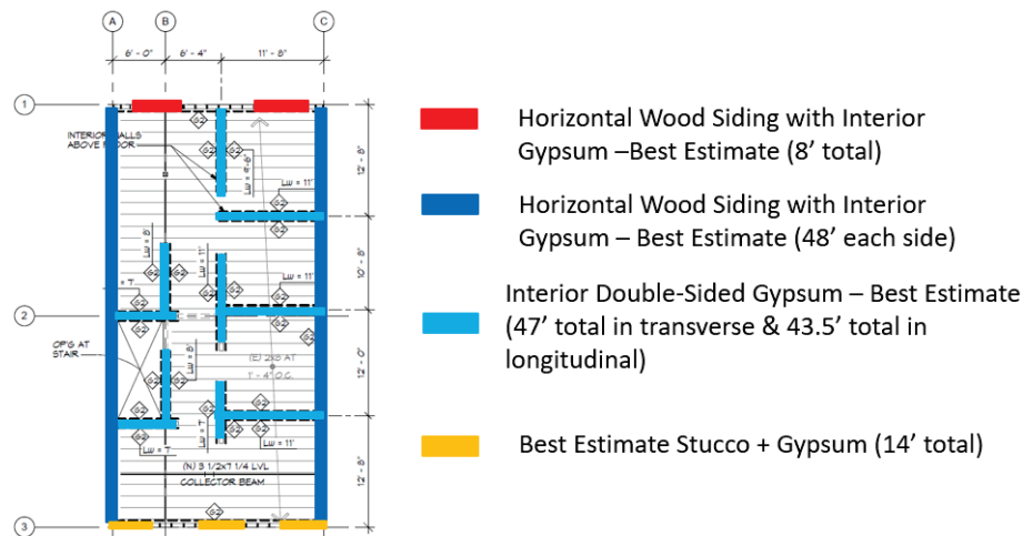
Figure 12-8 Typical existing wall layouts for the first story of HOG configurations.
