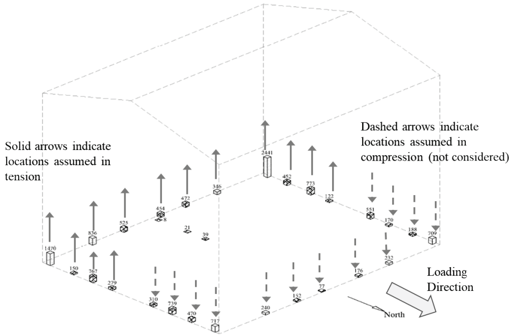
Figure 8-6 Example of anchorage elements assumed in tension for north loading: Test 5.S.4R (figure adapted from Fischer et al. (2001; 2002)).
