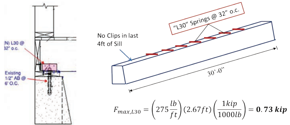
Figure 9-9 Illustration of the out-of-plane (OOP) connection at the sill plate (left) and the placement of equivalent L30 clip elements along the foundation beam (right).
