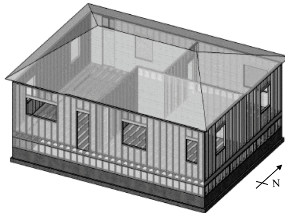
Figure 11-5 Rendering of one-story superstructure baseline configuration on two-foot cripple wall used in numerical modeling.
