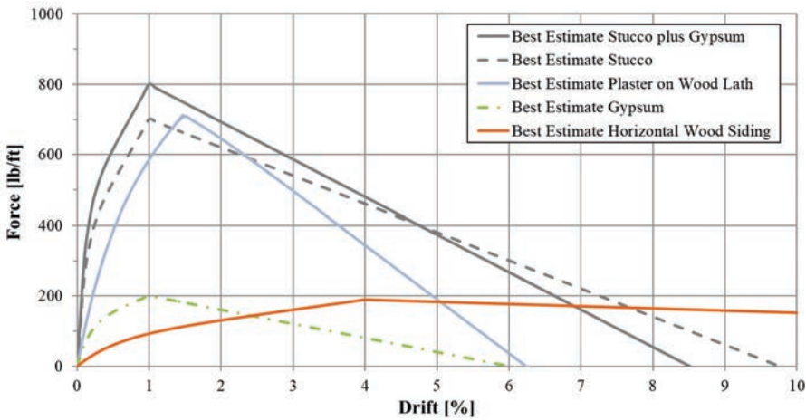
Figure 6-17 SAWS backbone curves for best-estimate materials used in superstructure study for analysis of cripple wall dwellings. Backbones reflect best-estimate properties.
