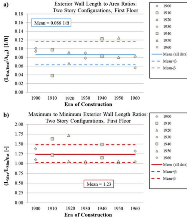
Figure 6-9 Exterior wall criteria for the first floor of two-story configurations: (a) Exterior wall density, (b) Maximum-to-minimum length ratio.
