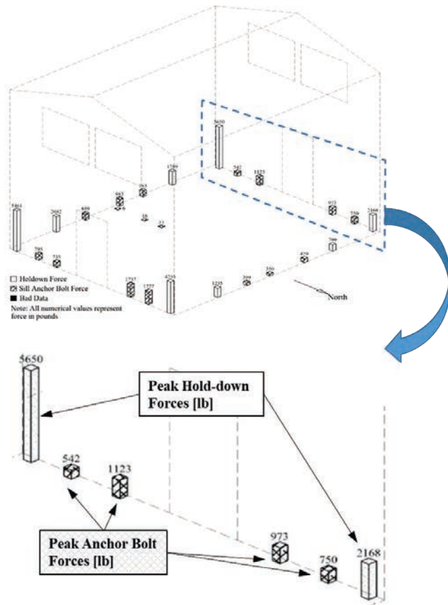
Figure 8-3 Example of documented anchorage uplift forces from the test by Fischer et al. (2001; 2002) (Current case is Test 7.S.4).
