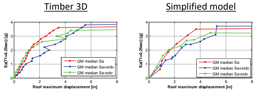
Figure 1-19 Incremental dynamic analysis curves for base line building model under three selected ground motion records predicted by Timber3D and simplified model.
