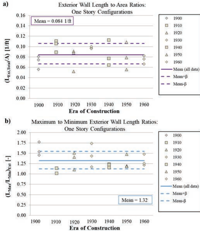
Figure 6-7 Exterior wall criteria for one-story configurations: (a) Exterior wall density, (b) Maximum-to-minimum wall length ratio.
