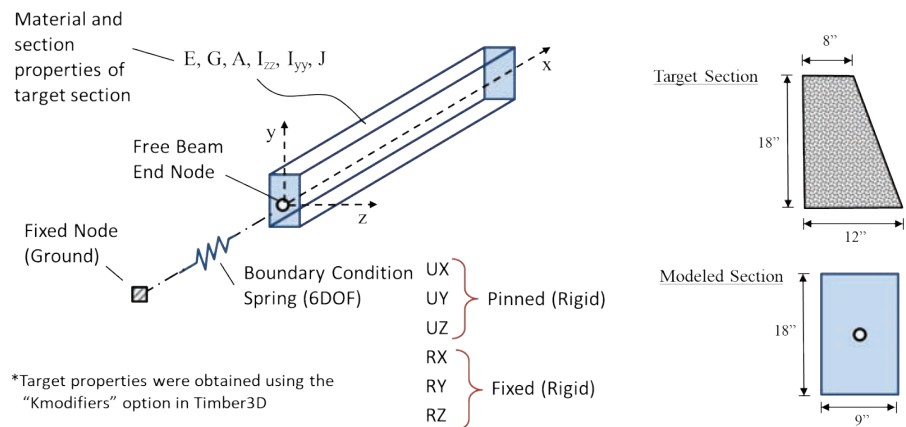
Figure 9-10 Modeling assumptions for creating the foundation beam at the uphill wall line.
