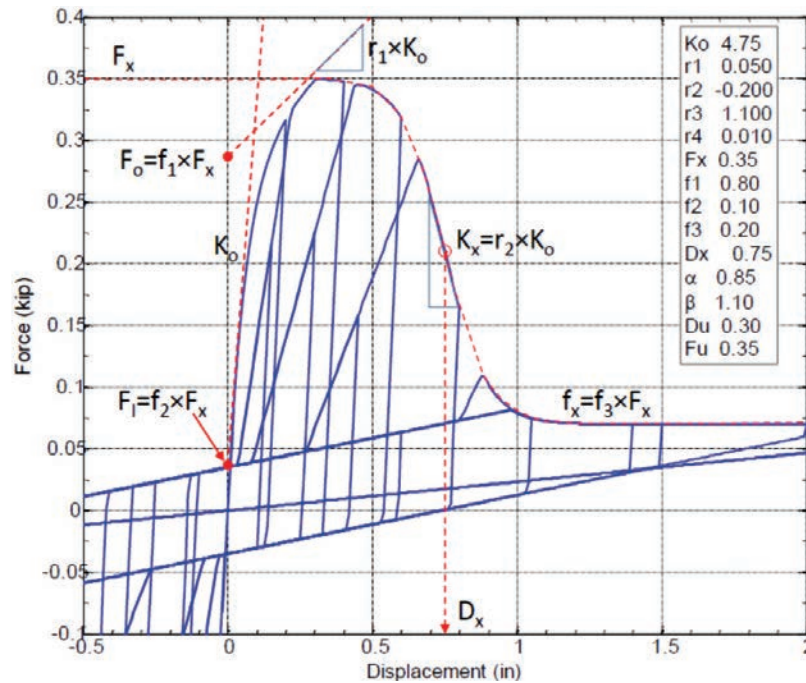
Figure 4-19 Modification of CUREE hysteretic rule for modeling residual strength (RESST hysteresis model in Timber3D ).
