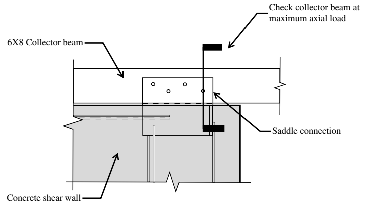
Figure 13A-25 Collector beam to saddle connection diagram
