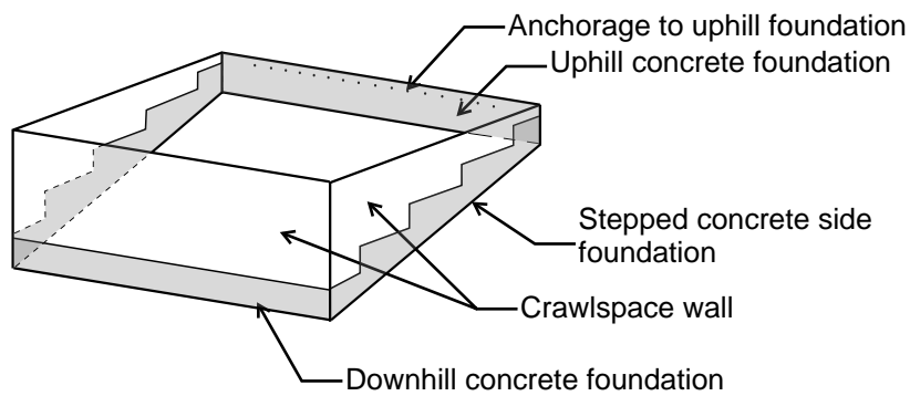
Figure 13A-9 Hillside dwelling schematic isometric of dwelling. (FEMA P-1100 Volume 1, Figure 6.1-2)
