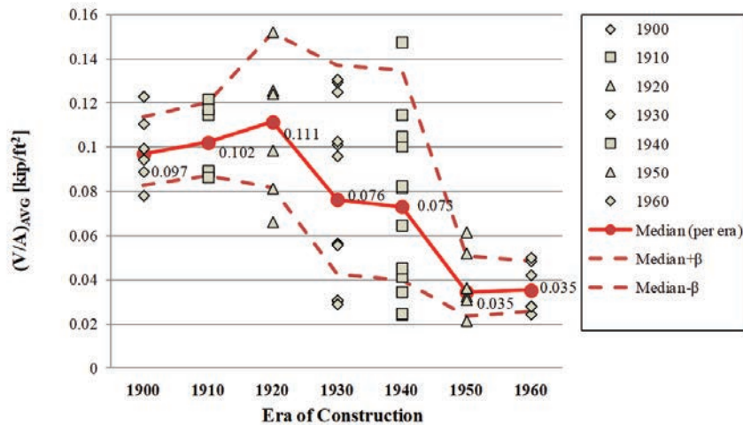
Figure 6-22 Strength-to-plan area ratios for one-story configurations.
