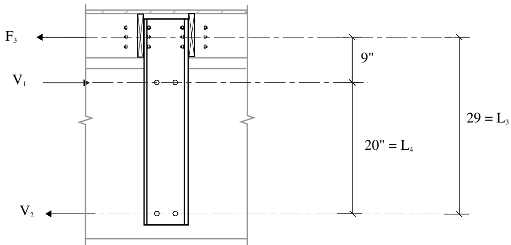
Figure 13A-37 Shear anchor elevation
