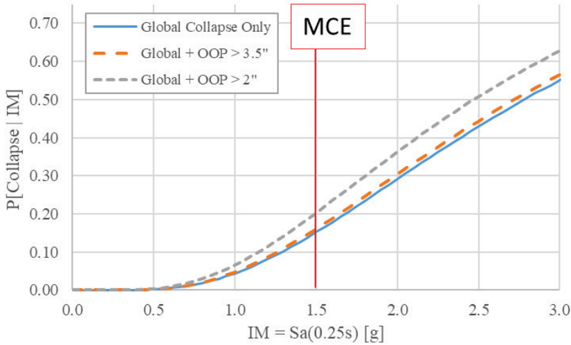
Figure 9-13 Example of using out-of-plane (OOP) displacement to relate to non-simulated collapse in addition to global collapse returned from structural analysis.
