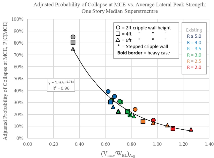
Figure 11-20 Trends of probability of collapse at the MCE intensity level versus the average peak strength-to-baseline weight ratio: One-story median pre-1950 superstructure. Note: All collapses occur at the cripple wall level.
