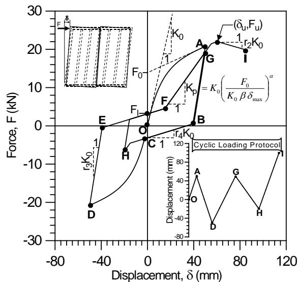
Figure 1-1 CUREE hysteretic rule for modeling force-displacement response of wood shear walls under cyclic loading.
