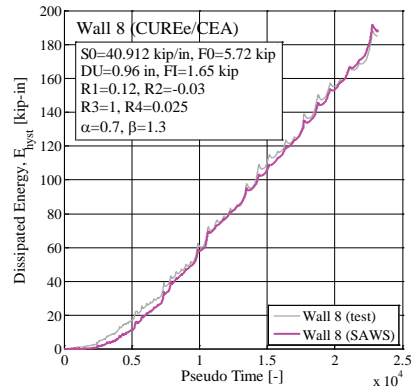
Figure 4-27 (ctd) Comparison of hysteretic response and cumulative dissipated energy for test data (Tests 7 and 8 from Arnold et al., 2003b) and optimized CUREE parameters (see Table 4-7) for walls sheathed with single/upper story stucco + gypsum.
