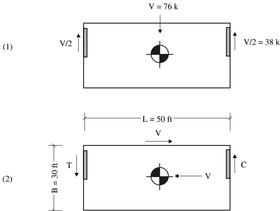
Figure 13A-12 Primary anchor configuration
