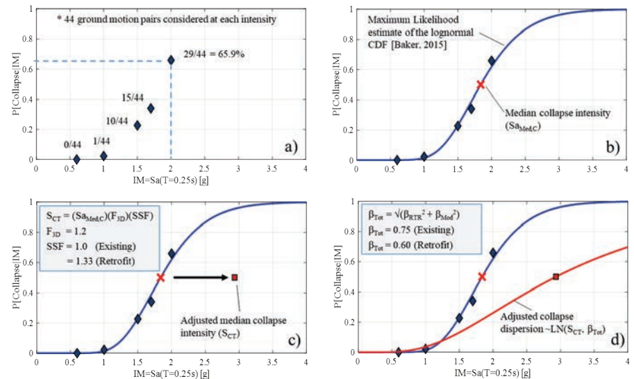
Figure 11-16 Illustration of process used for estimating the collapse fragility of a cripple wall dwelling according to the FEMA P-695 procedure: a) estimate fractions of collapse; b) maximum likelihood estimate of median collapse intensity from analysis; c) adjusted median intensity for spectral shape and 3-D effects (i.e., correction factors applied); d) adjusted collapse fragility dispersion.
