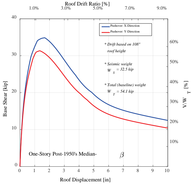
Figure 6-39 Pushover curves for the one-story post-1950's Median- \beta Superstructure (Archetype 4-1R-M \beta -E).
