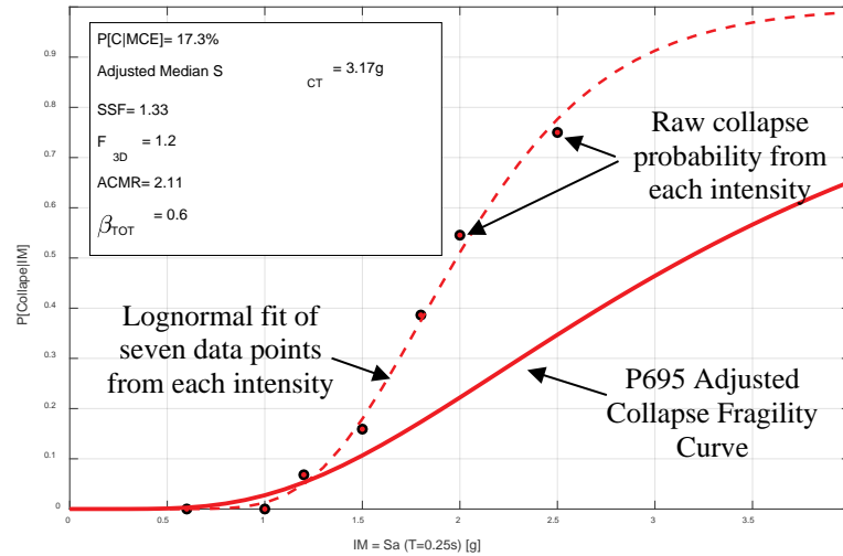
Figure 12-18 Conversion of raw collapse information to full FEMA P-695 collapse fragility curve.
