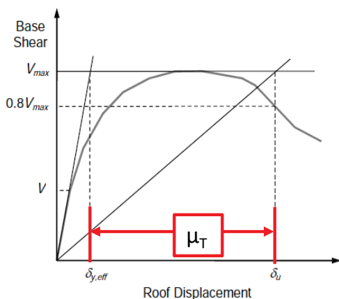
Figure 5-1 Definition of period-based ductility factor ( \mu_T ).
