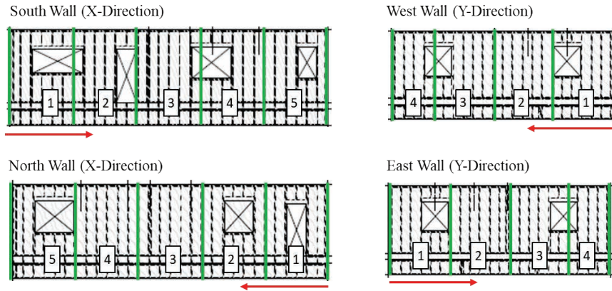
Figure 6-34 Building block discretization for exterior wall lines of archetype buildings.
