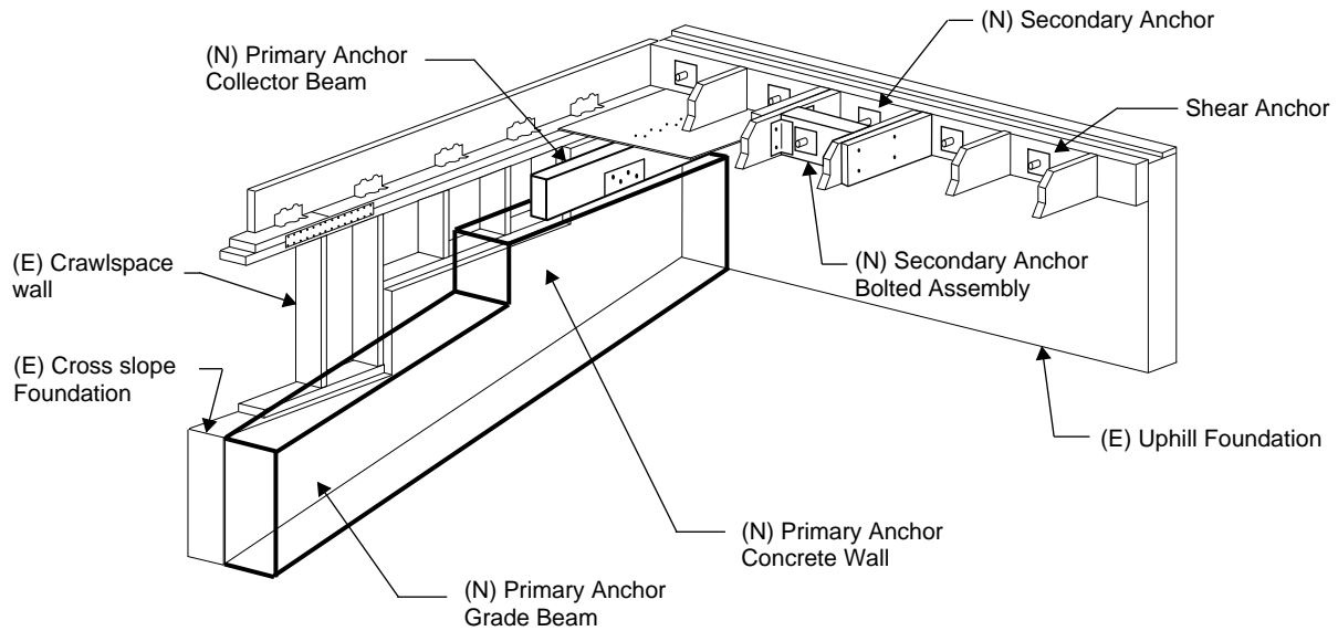
Figure 13A-10 Interior uphill foundation corner isometric showing primary anchors, secondary anchors, and shear anchors. (FEMA P-1100 Volume 1, Figure 6.5-1)
