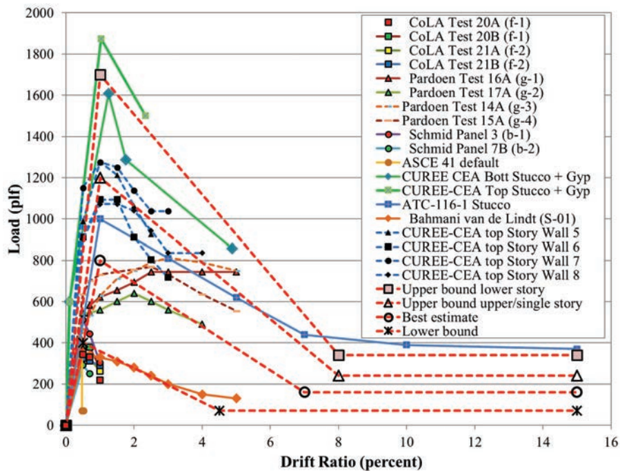
Figure 4-1 Plot of applicable test data and approximate backbone for stucco plus gypsum wallboard.
