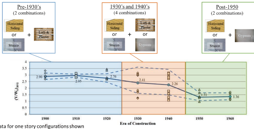
Figure 11-4 Illustration of the different building materials assumed when considering the existing one story building stock of cripple wall dwellings.
