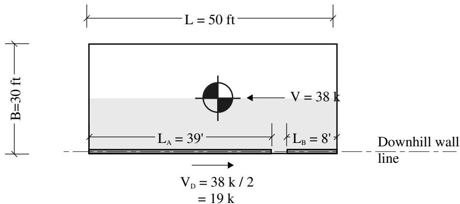
Figure 13A-15 Downhill crawspace wall configuration
