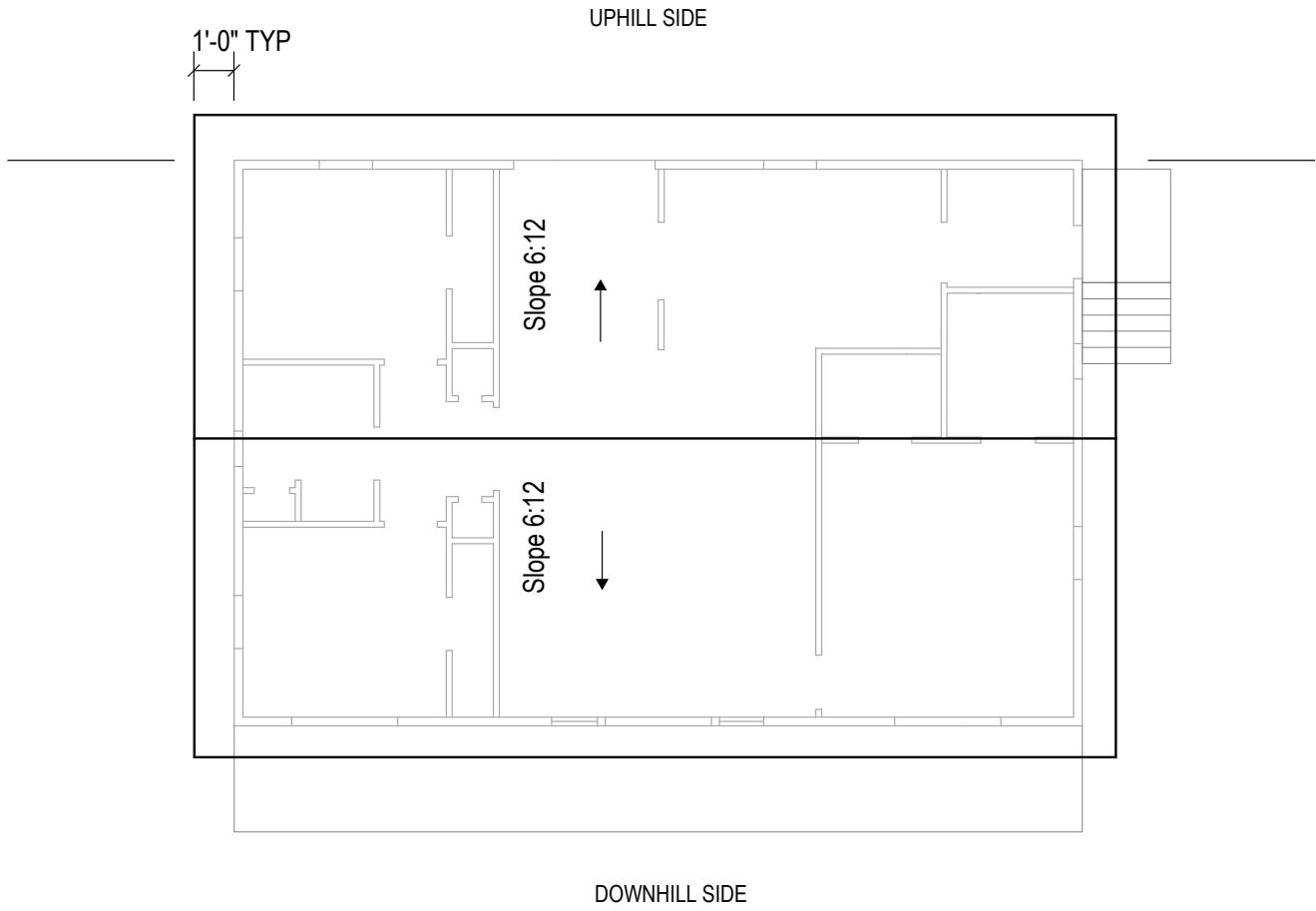
Figure 13A-2 Roof plan
