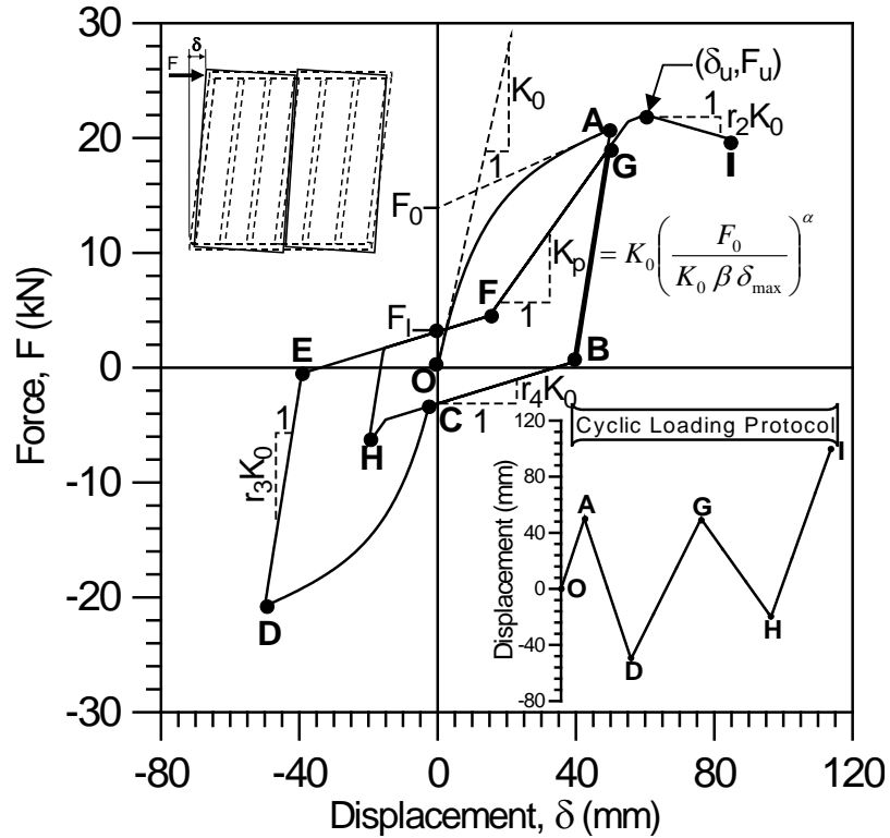
Figure 4-18 CUREE hysteretic rule for modeling force-displacement response of wood shear walls under cyclic loading.
