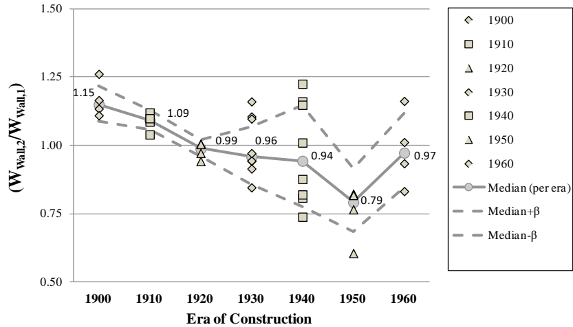
Figure 6-24 Second-to-first-story wall weight ratios for two-story configurations.
