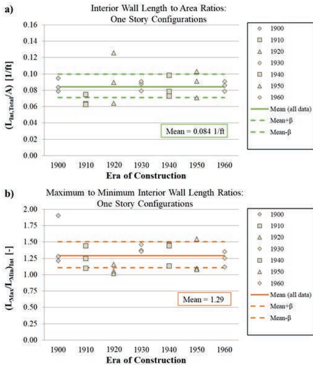
Figure 6-8 Interior wall criteria for one-story configurations: (a) Interior wall density, (b) Maximum-to-minimum wall length ratio.
