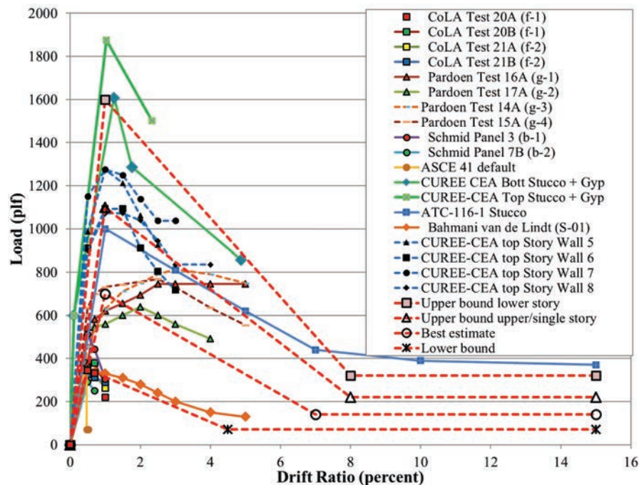
Figure 4-3 Plot of applicable test data and approximate backbone for stucco.
