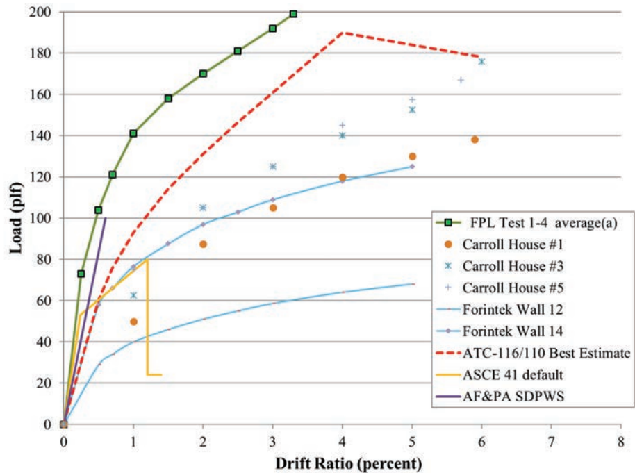
Figure 4-4 Plot of applicable test data and approximate backbone for horizontal lumber sheathing.
