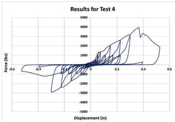
Figure 13-15 Hysteresis plots for a wood to steel 1/2" bolt specimen tested at Washington State University.
