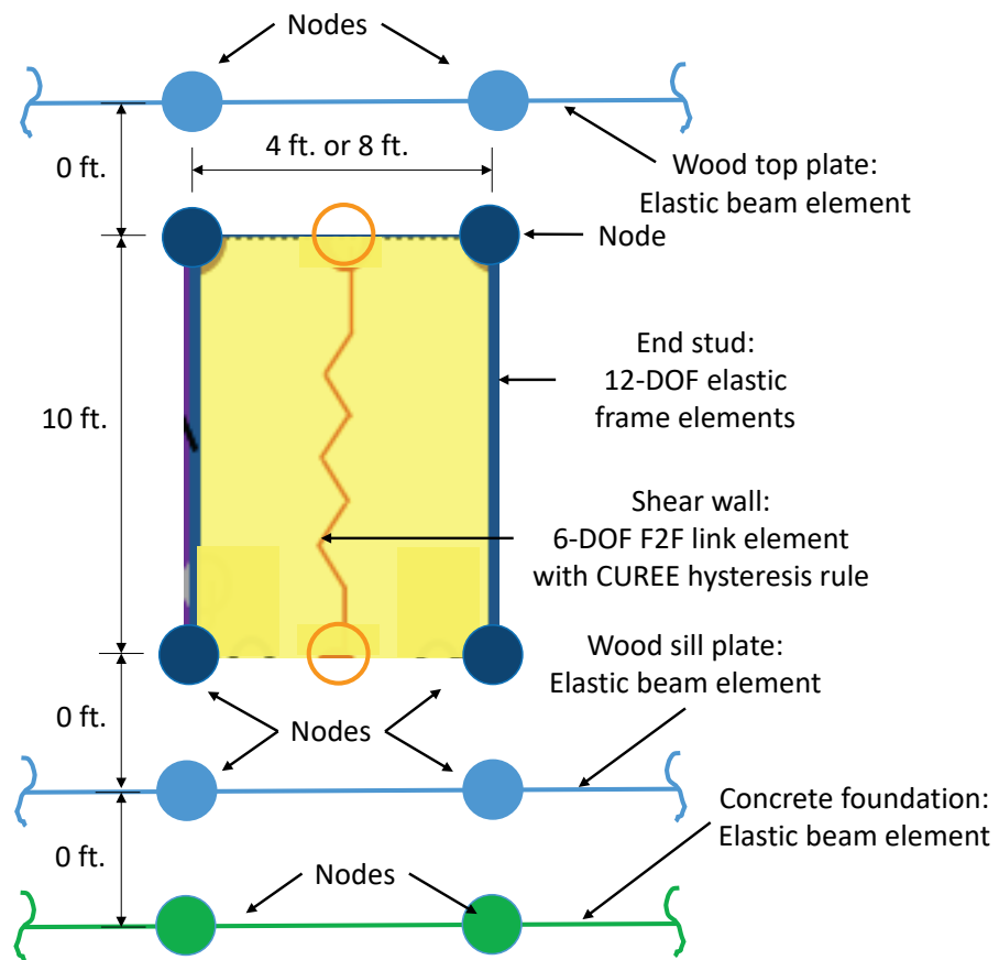
Figure 1-4 Schematic illustration of vertical wall building block.
