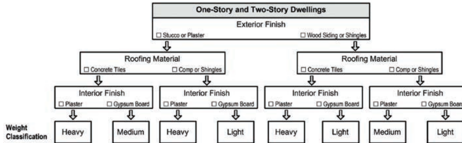
Figure 11-31 Mapping of material weight combinations into weight classifications for cripple wall constructability analysis.
