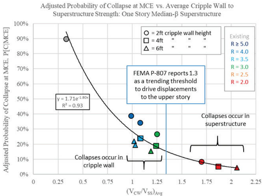
Figure 11-23 Trends of probability of collapse at the MCE intensity level versus the average cripple wall-to-superstructure strength ratio: One-story median-β post-1950 superstructure.
