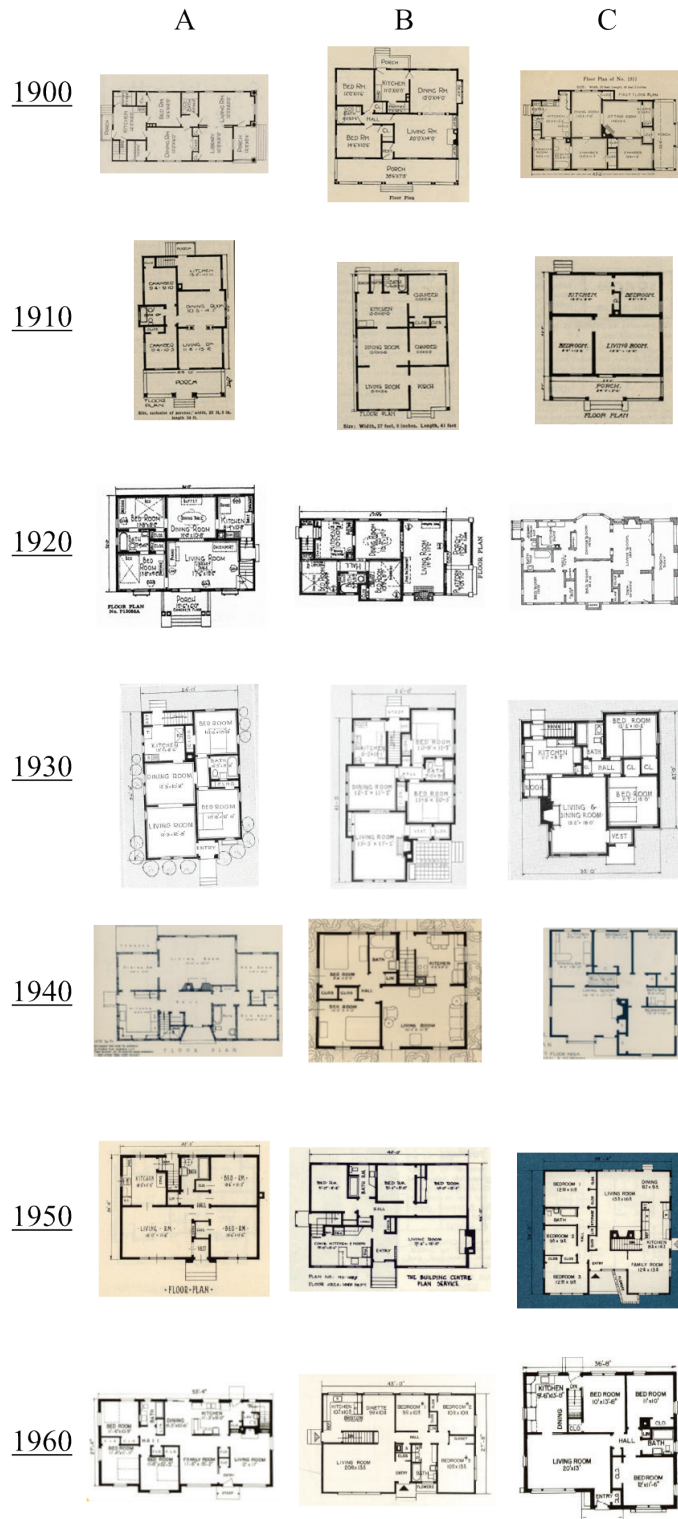
Figure 6-2 Plan drawings for the three one-story configurations considered for each construction era. Images are not to relative scale.
