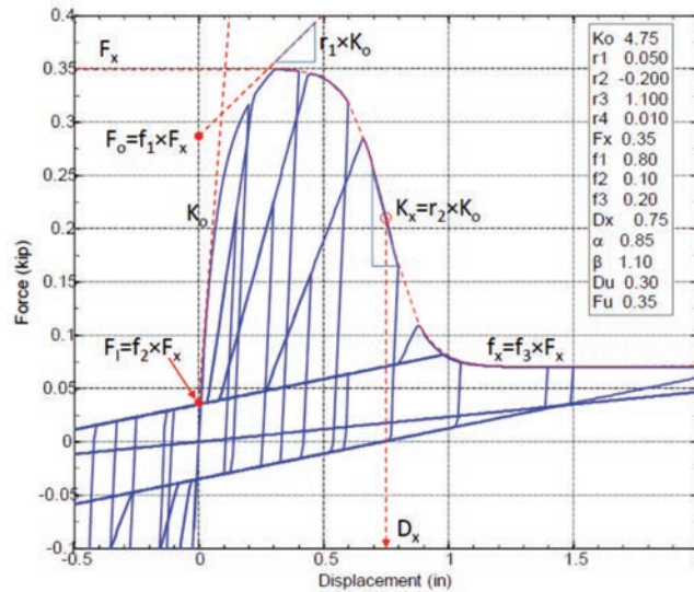
Figure 11-9 Illustration of the residual strength (RESST) hysteretic model used in Timber3D for modeling the behavior of wall materials.
