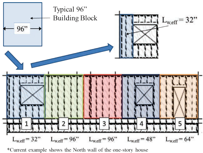
Figure 6-33 Example of the effective length assumption used for accounting for openings within building block of exterior wall lines. Current example is for the north wall line of the one-story configuration.
