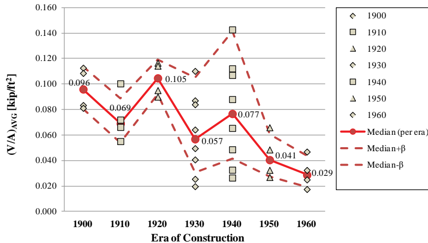
Figure 6-28 Strength-to-area ratios for the bottom story of two-story configurations.
