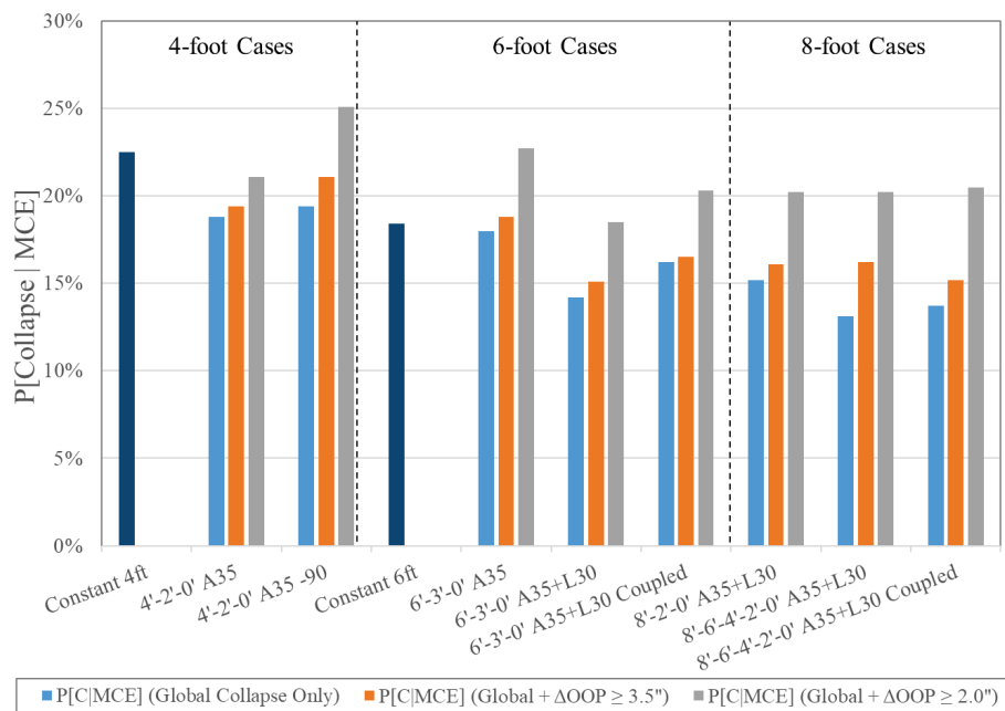
Figure 9-14 Collapse performance summary at the MCE level for all transition study archetypes. All archetypes included retrofit.
