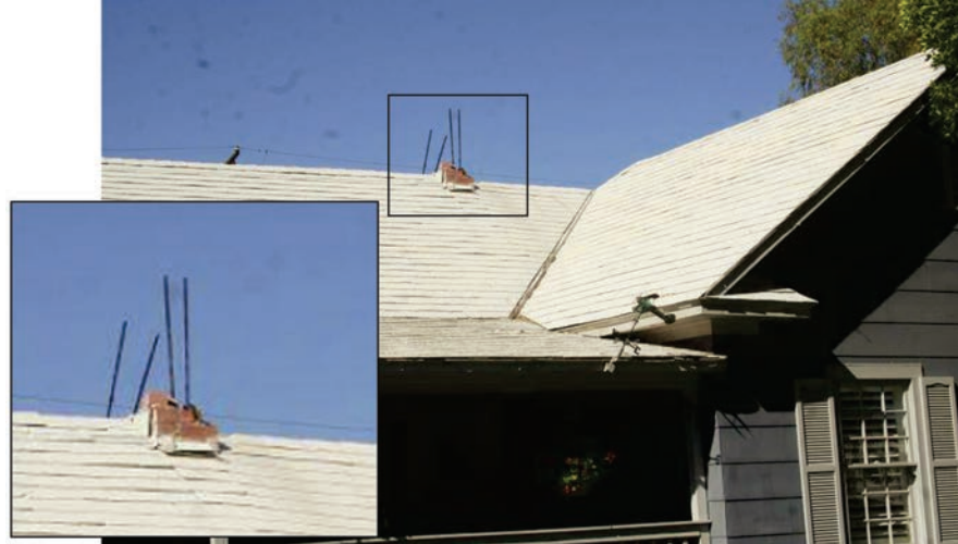
Figure 10-6 Atypical failure of reinforced, one-story interior chimney. Note that the chimney is fully braced on all sides at the ridge, and the rebar protruding from the remaining masonry indicates that the chimney was reinforced and did not extend very high above the roof. (Photo by authors)
