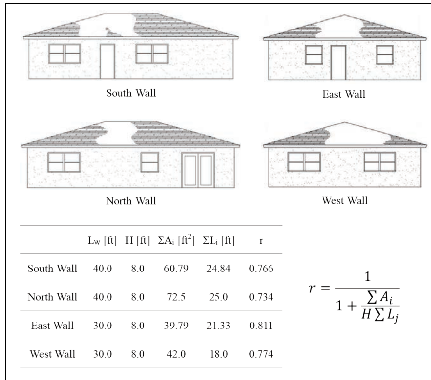
Figure 4-17 Calculation of sheathing area ratios ( r ) for the exterior walls of the CUREE Small House (Isoda et al., 2002)
