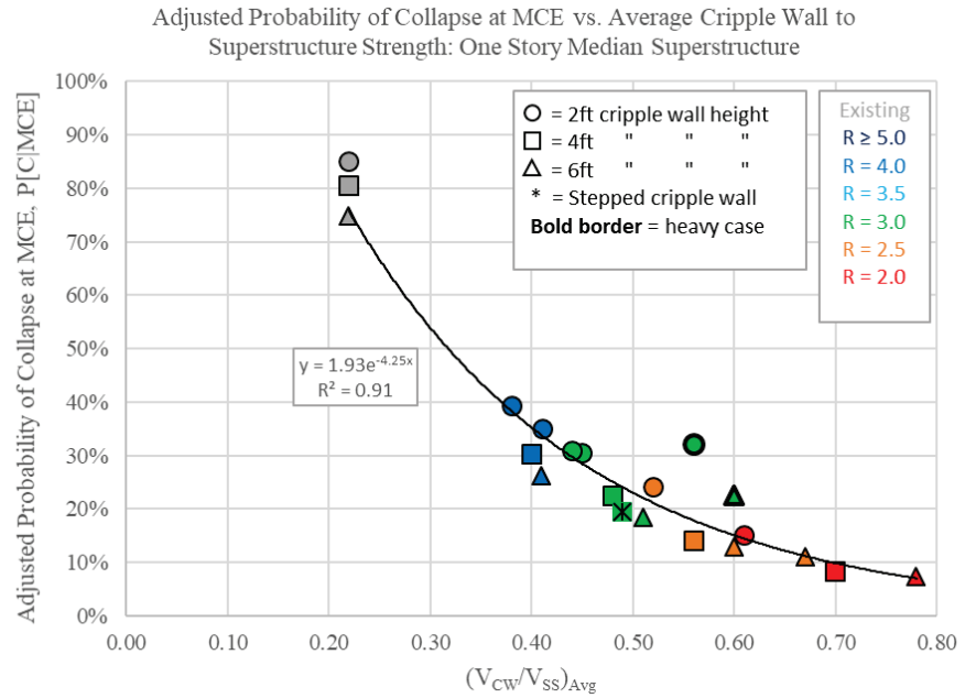
Figure 11-21 Trends of probability of collapse at the MCE intensity level versus the average cripple wall-to-superstructure strength ratio: One-story median pre-1950 superstructure. Note: All collapses occur at the cripple wall level.
