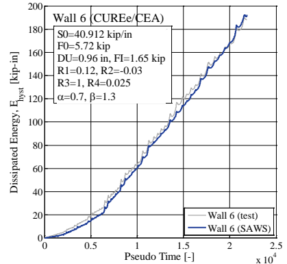
Figure 4-27 Comparison of hysteretic response and cumulative dissipated energy for test data (Tests 5 and 6 from Arnold et al., 2003b) and optimized CUREE parameters (see Table 4-7) for walls sheathed with single/upper story stucco + gypsum.
