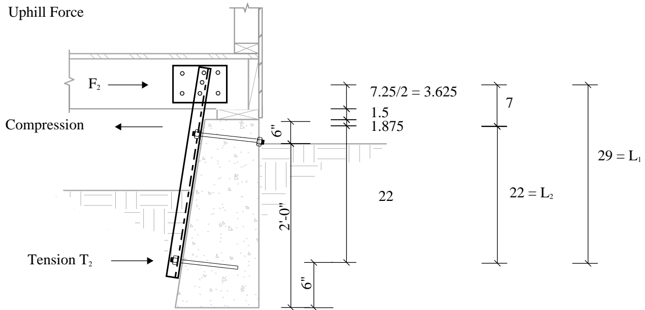
Figure 13A-33 Secondary anchor uphill force diagram
