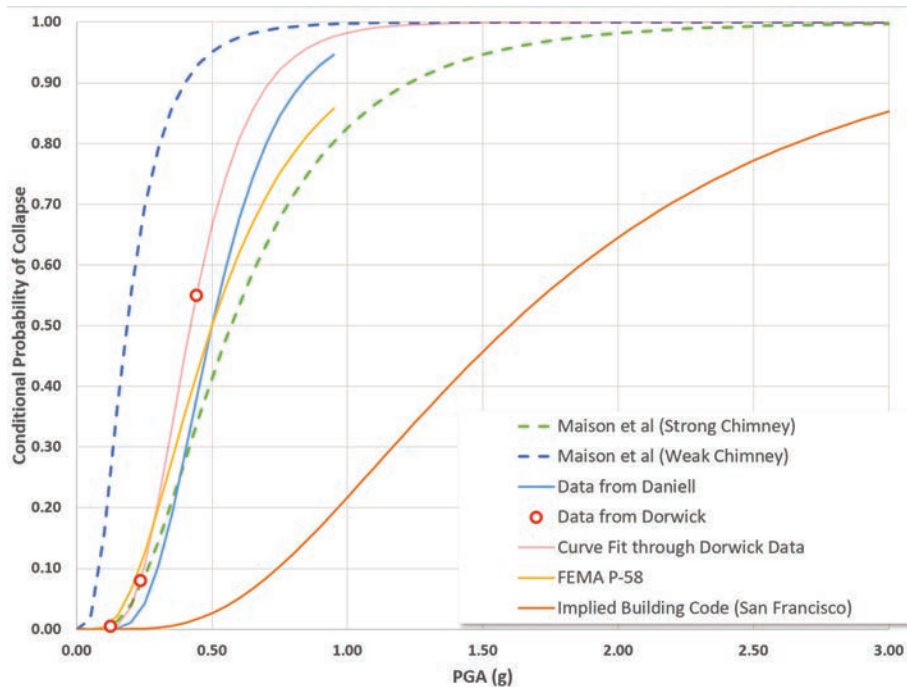
Figure 10-7 Masonry residential chimney fragility functions derived from various sources show that the collapse vulnerability is much higher than the implicit performance goal of the building code (shown for San Francisco in terms of peak ground acceleration).
