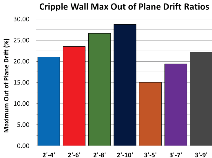
Figure 9-16 Maximum out of plane crawl space wall drift ratio (%) values for 32'×48' monotonic study.
