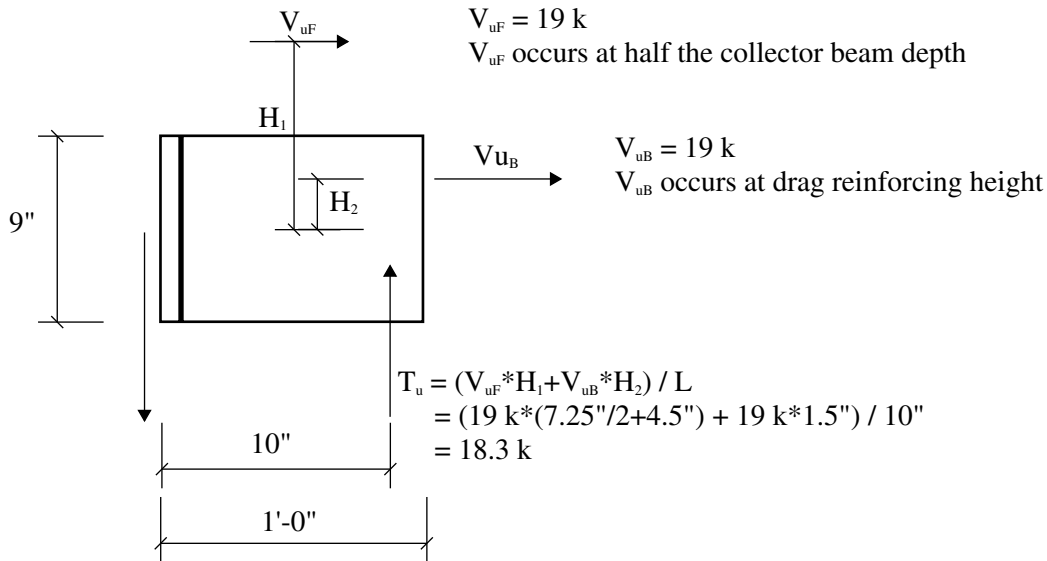
Figure 13A-24 Saddle Connection Elevation
