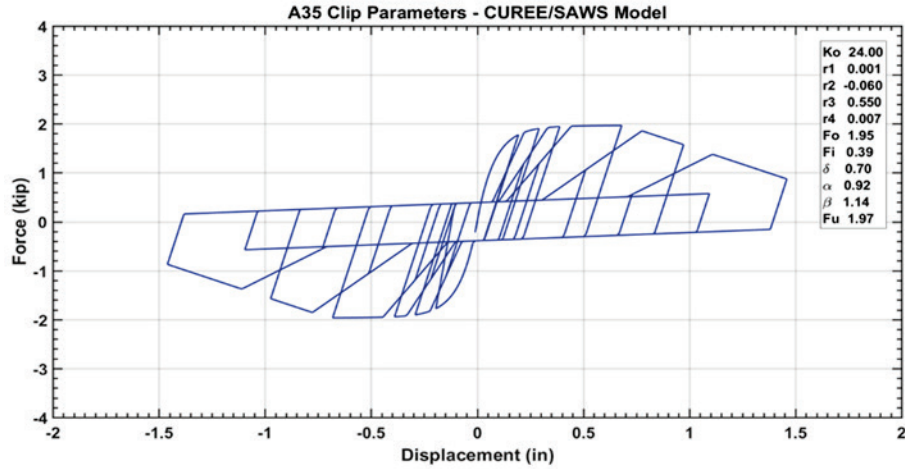
Figure 4-34 CUREE hysteretic model parameters for A35 clips with in-plane shear loading.
