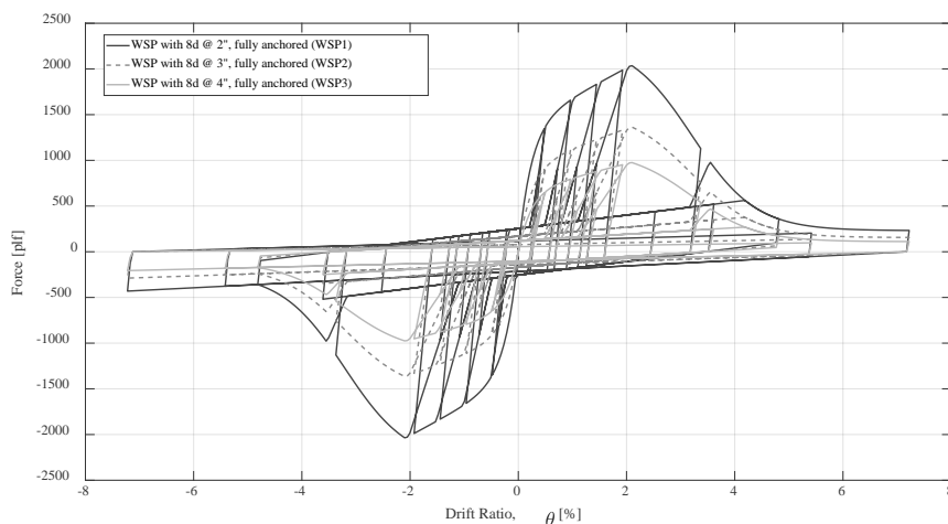
Figure 11-17 Hysteretic behavior of baseline wood structural panels assuming full anchorage conditions with tie-downs (WSP1 to WSP3).
