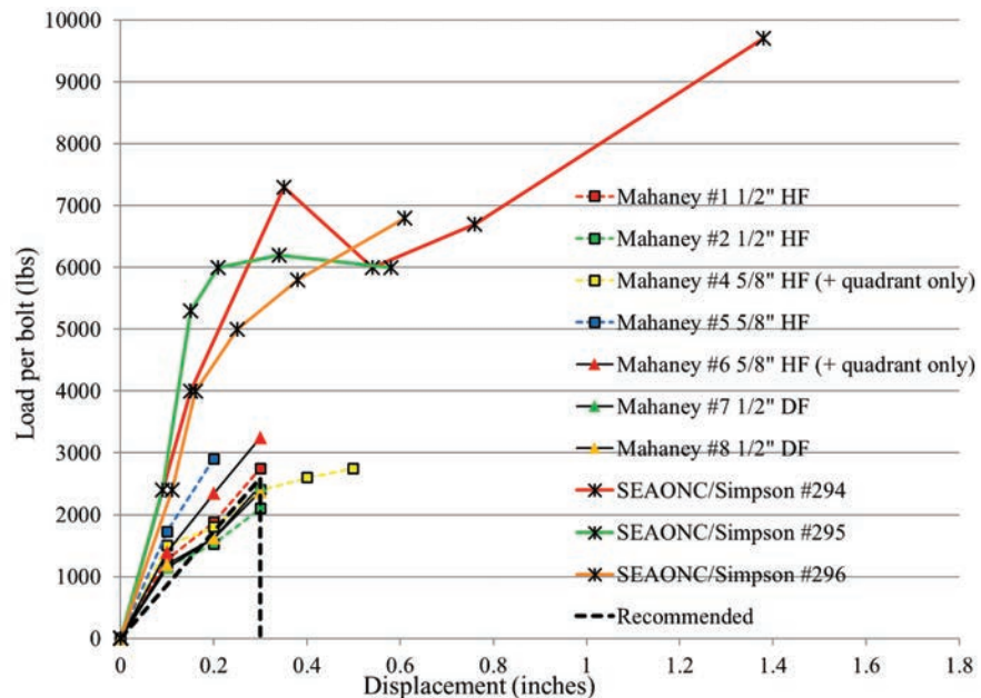
Figure 4-12 Plot of applicable test data and load-deflection behavior of anchor bolts in-plane.
