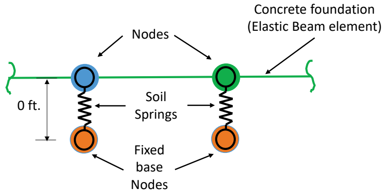
Figure 1-10 Schematic illustration of modeling of non-linear soil springs.
