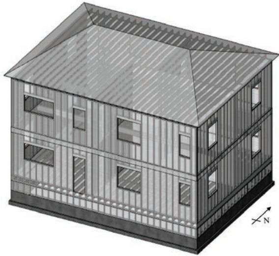
Figure 11-6 Rendering of two-story superstructure baseline configuration on two-foot cripple wall used in numerical modeling.
