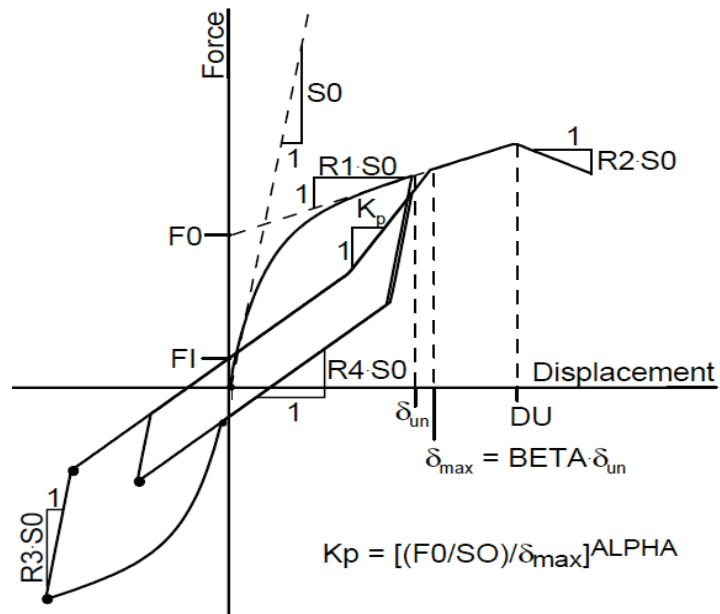
Figure 12-13 Illustration of the modified STEWart (MSTEW) hysteretic model used in Timber3D for modeling the behavior of wall materials.
