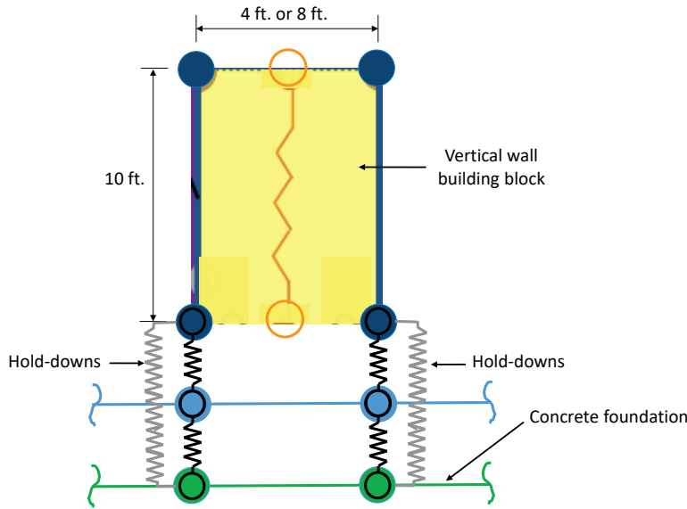
Figure 1-8 Schematic illustration of modeling of non-linear hold-down devices.
