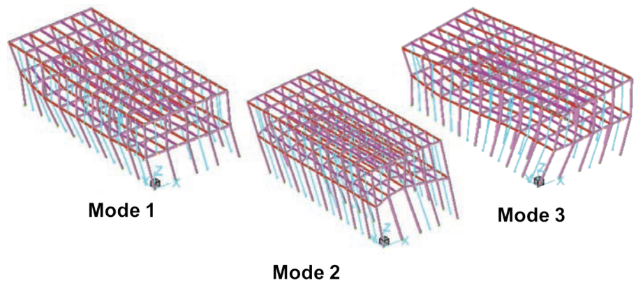
Figure 12-24 Plotted mode shapes for 5-HOG3-H-5SW configuration.
