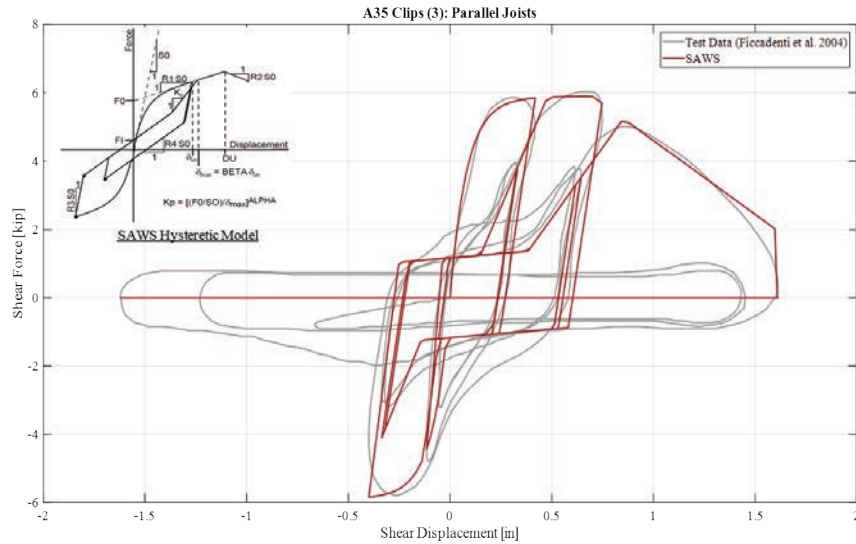
Figure 9-7 Fitting of SAWS hysteretic model to A35 clip testing conducted by Ficcadenti et al. (2004). NOTE: The test shown is for three clips in parallel.
