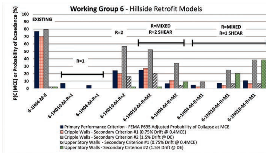
Figure 13-25 Criteria plot for the various hillside retrofit models illustrating performance criteria as discussed in Part 2.
