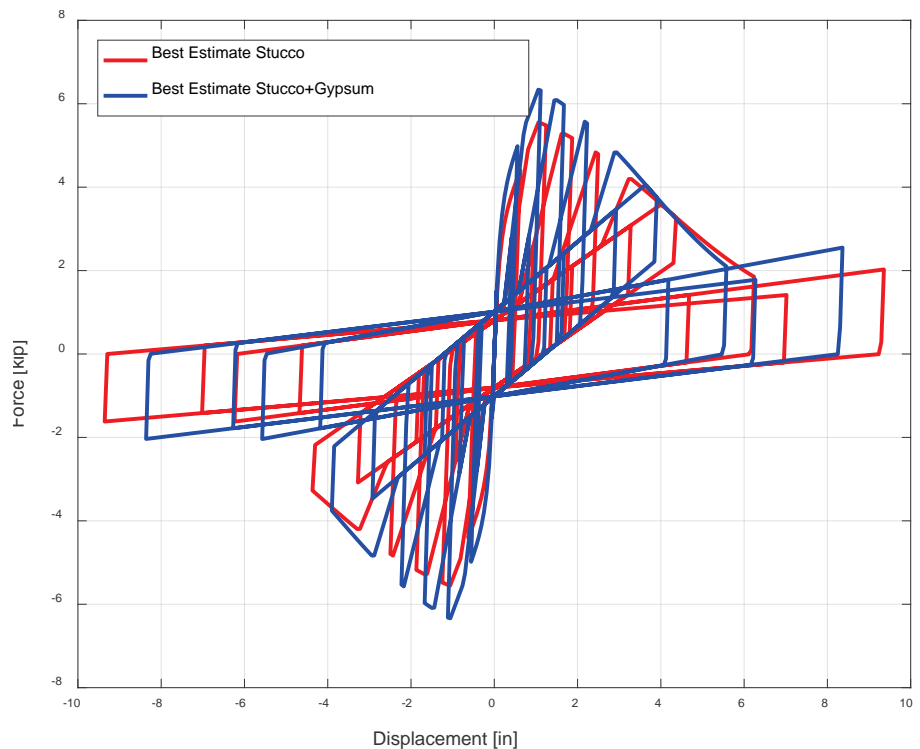
Figure 12-14 Hysteretic parameters for stucco and stucco+gypsum.
