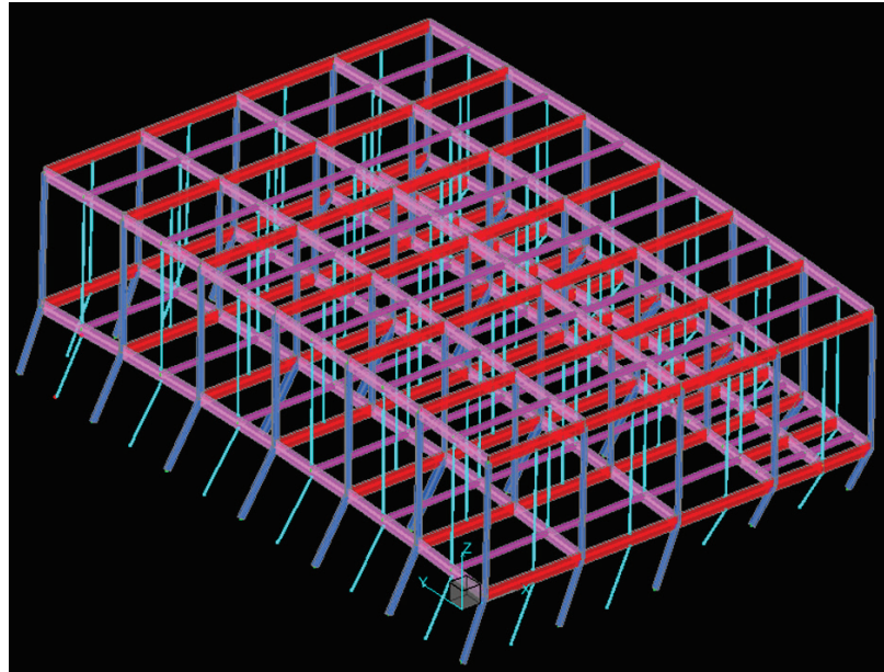
Figure 9-15 Deformed shape for monotonic uphill push (32'×48').
