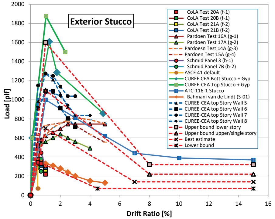
Figure 4-22 Test data and recommended backbone curves for walls sheathed with stucco.
