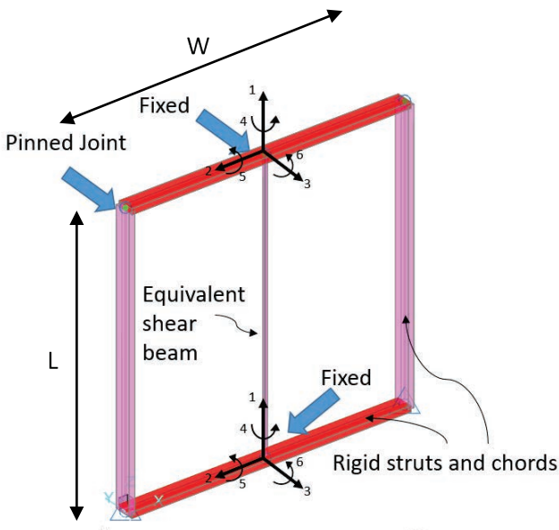
Figure 1-15 Schematic illustration of modeling of a semi-rigid diaphragm.
