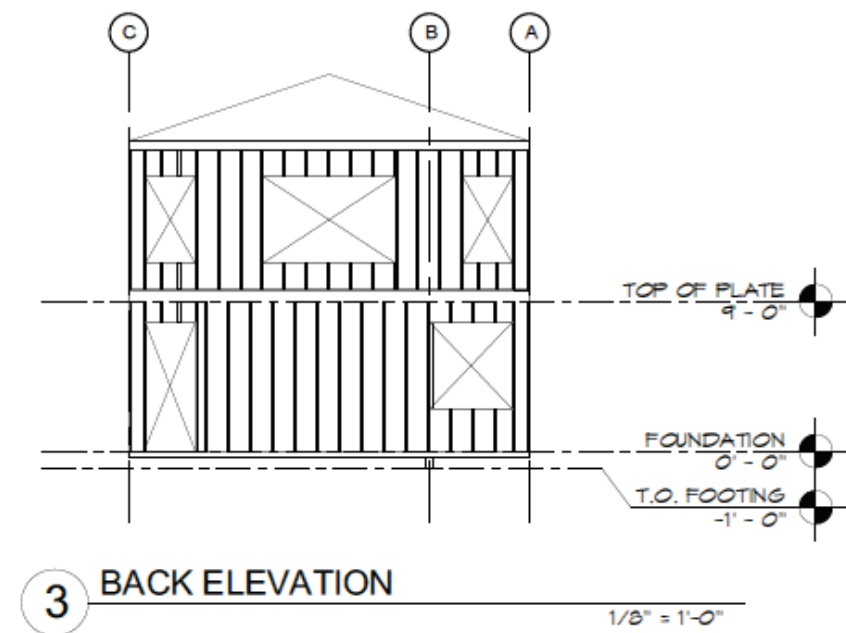
Figure 12-4 Elevation views of house-over-garage configurations.
