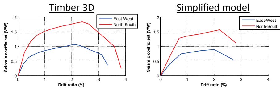
Figure 1-17 Pushover curves for base line building model predicted by Timber3D and simplified model.
