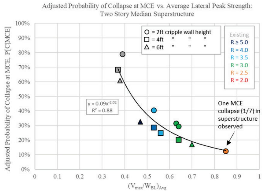
Figure 11-24 Trends of probability of collapse at the MCE intensity level versus the average peak strength to baseline weight ratio: Two-story median pre-1950 superstructure.
