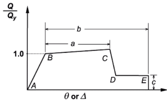
Figure 12-19 Steel backbone behavior from ASCE 41-13.
