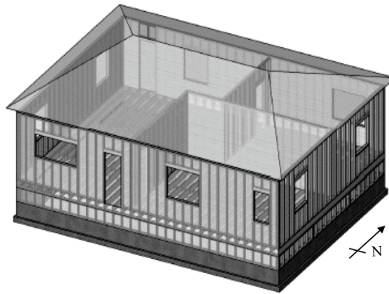
Figure 6-29 Rendering of one-story superstructure baseline configuration used in numerical modeling (rendering depicts structure on a 2-foot tall cripple-wall).
