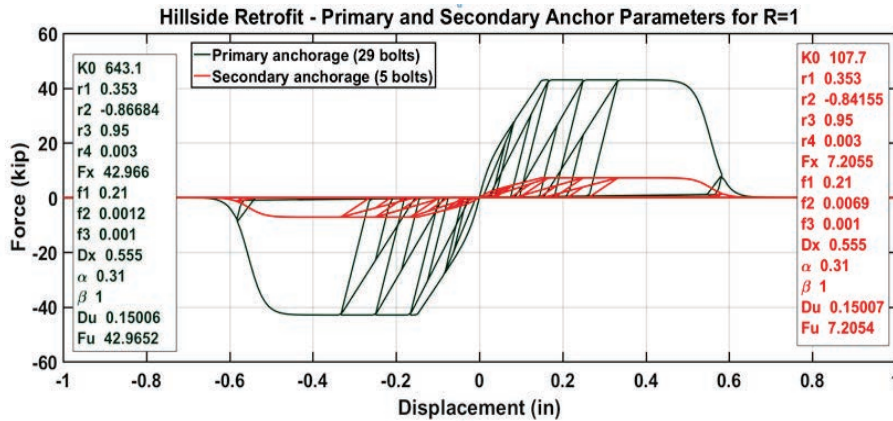
Figure 13-17 Primary and secondary anchor parameters for Model 6-1H04-M-R=1.
