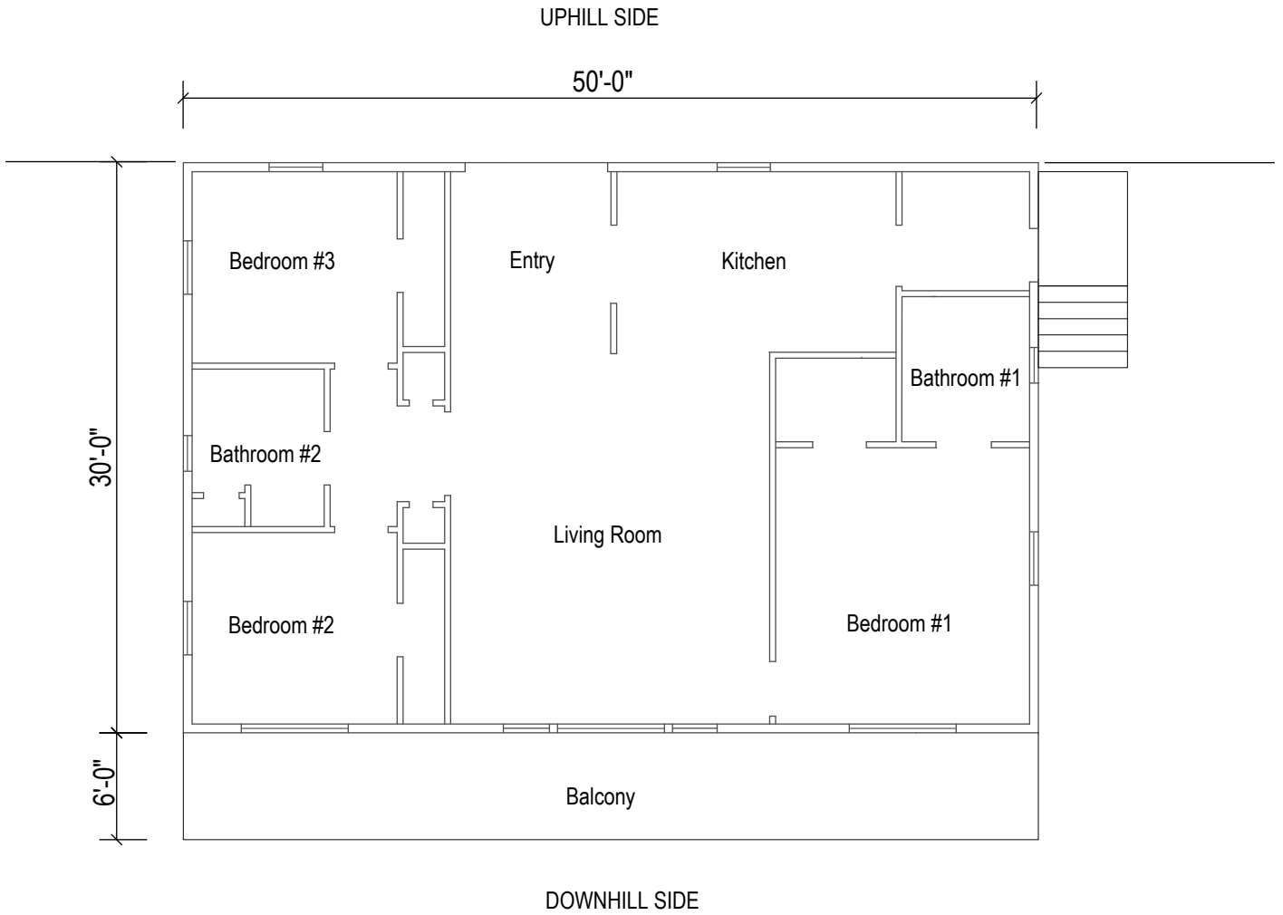
Figure 13A-1 First floor plan
