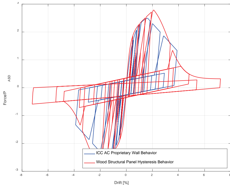
Figure 12-23 Hysteresis behavior of ICC AC proprietary and wood structural panel walls.
