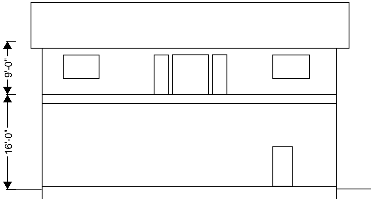
Figure 13A-5 Downhill elevation
