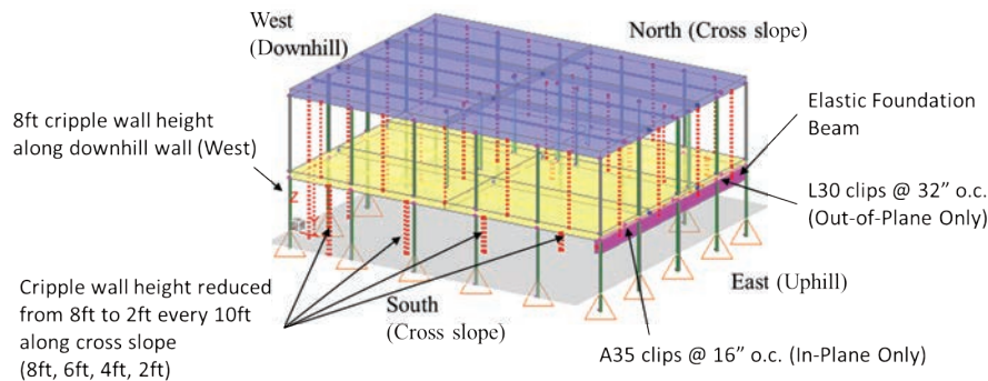
Figure 9-11 Rendering of Timber3D model representing a one-story cripple wall dwelling with a ‘zero-height’ condition. Current case shows both in-plane and out-of-plane resistance considered at the uphill wall line.
