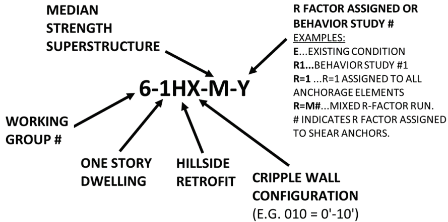
Figure 13-10 Numerical modeling nomenclature.
