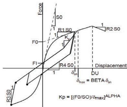
Figure 11-10 Illustration of the SAWS hysteretic model (image from Christovasilis and Filiatrault, 2009).
