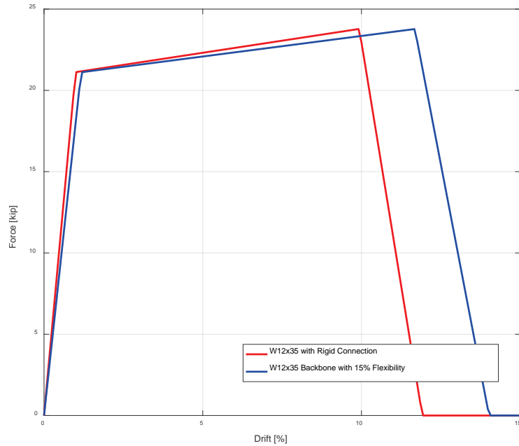
Figure 12-20 Backbone behavior of steel retrofits with and without stiffness decrease.
