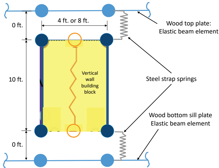
Figure 1-9 Schematic illustration of modeling of non-linear steel straps.
