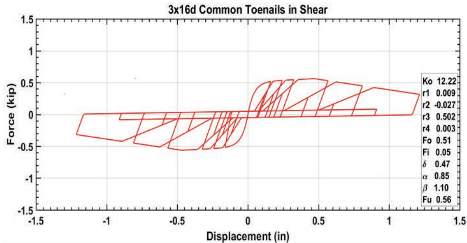
Figure 4-33 CUREE hysteretic model parameters for 3-16d common toenails in lateral shear.
