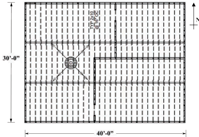
Figure 6-31 Plan view of the one- and two-story configurations selected for modeling of cripple-wall dwellings.
