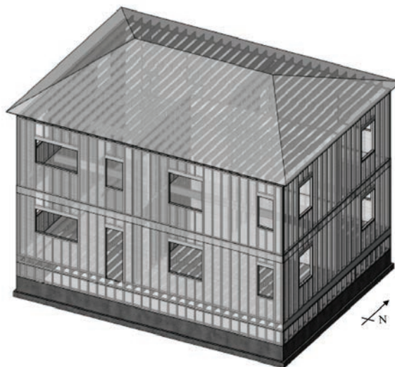
Figure 6-30 Rendering of baseline two-story superstructure configuration on two-foot cripple-wall used in numerical modeling.
