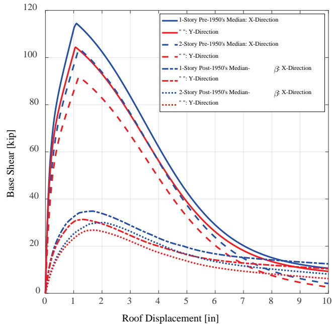
Figure 11-8 Modal pushover analysis ( Timber3D ) comparison of all four superstructure configurations considered for cripple wall dwelling analysis.
