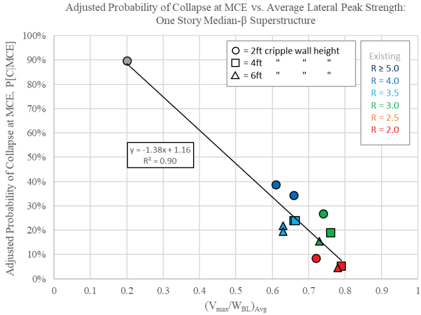
Figure 11-22 Trends of probability of collapse at the MCE intensity level versus the average peak strength-to-baseline weight ratio: One-story median-β post-1950 superstructure.
