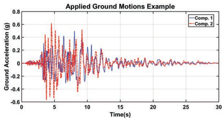
Figure 13-21 Example horizontal ground motions components shown for an earthquake included in the 22-far field ground motions.
