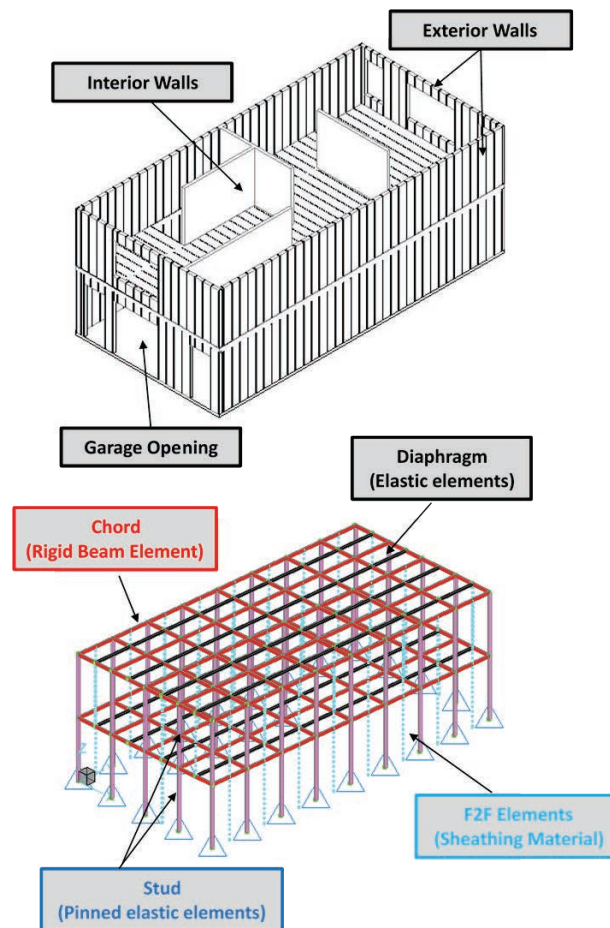
Figure 12-17 Illustration of modeling components of HOG dwelling including a rendering of actual dwelling and Timber3D components.
