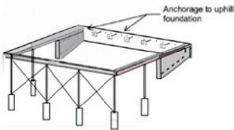
Figure 13-3 Hillside dwelling schematic illustration of the underfloor area with diagonal bracing and open area crawl space.
