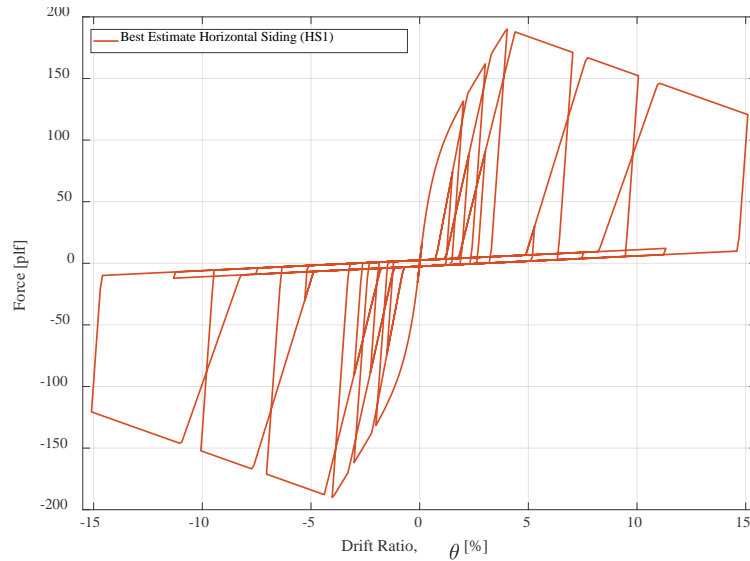
Figure 4-32 Example hysteretic response for horizontal wood siding using the CUREE hysteretic model and inputs parameters used within the ATC-116 project.
