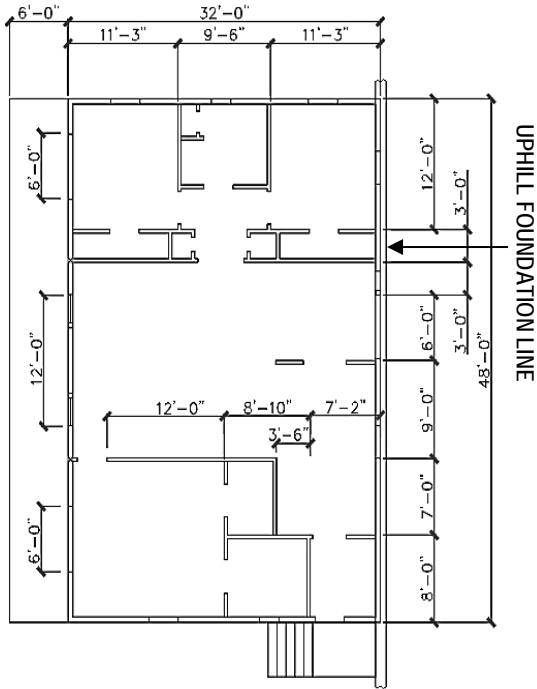
Figure 13-6 Dwelling occupied base level story plan for all models except Model 6-1H016-M-R=M1R.
