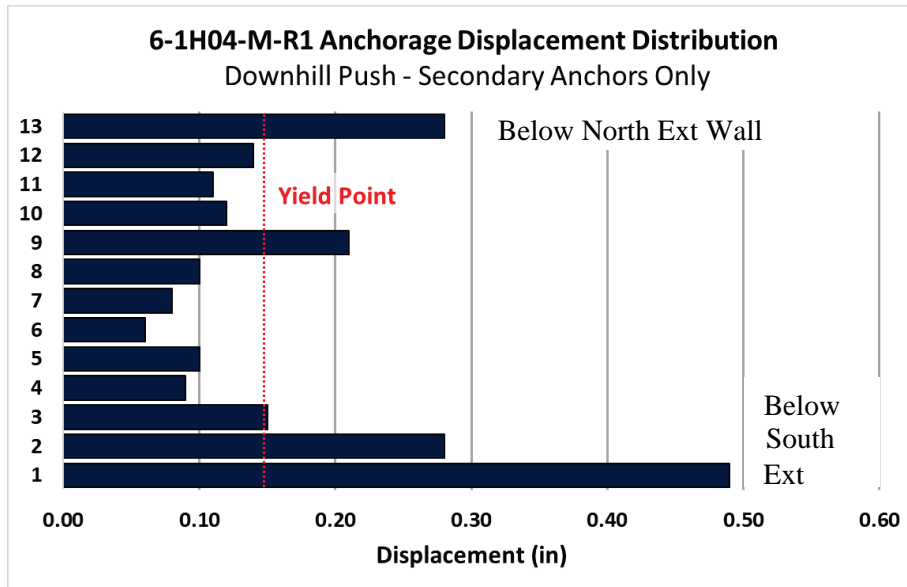
Figure 13-24 Secondary anchor displacement distribution for Model 6-1H04-M-R1 at peak loading when subjected to an out-of-hill monotonic push. The highest anchorage demand occurs near the stiffest superstructure wall lines, as discussed in Section 5.1.
