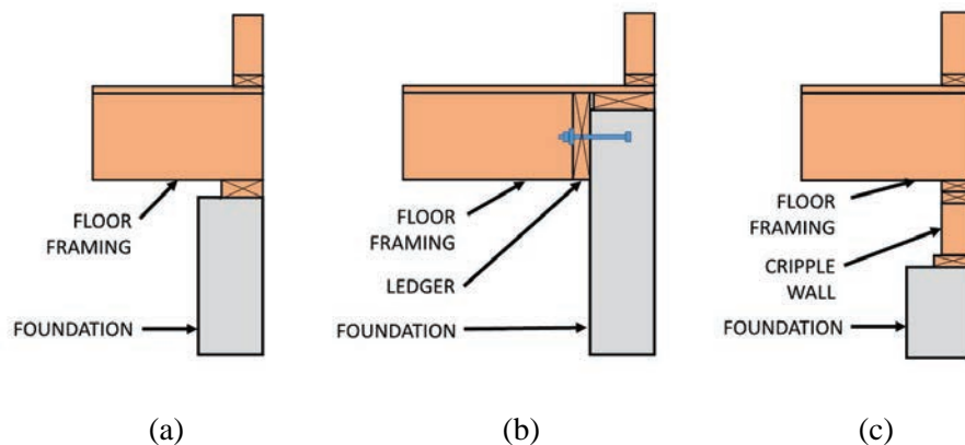
Figure 9-3 Floor diaphragm case examples: (a) illustrates Case 1 with the floor diaphragm sitting on top of the foundation, (b) illustrates Case 2 with the floor diaphragm supported on a ledger on the face of the foundation wall, and (c) illustrates Case 3 with the floor diaphragm sitting on a short cripple wall.
