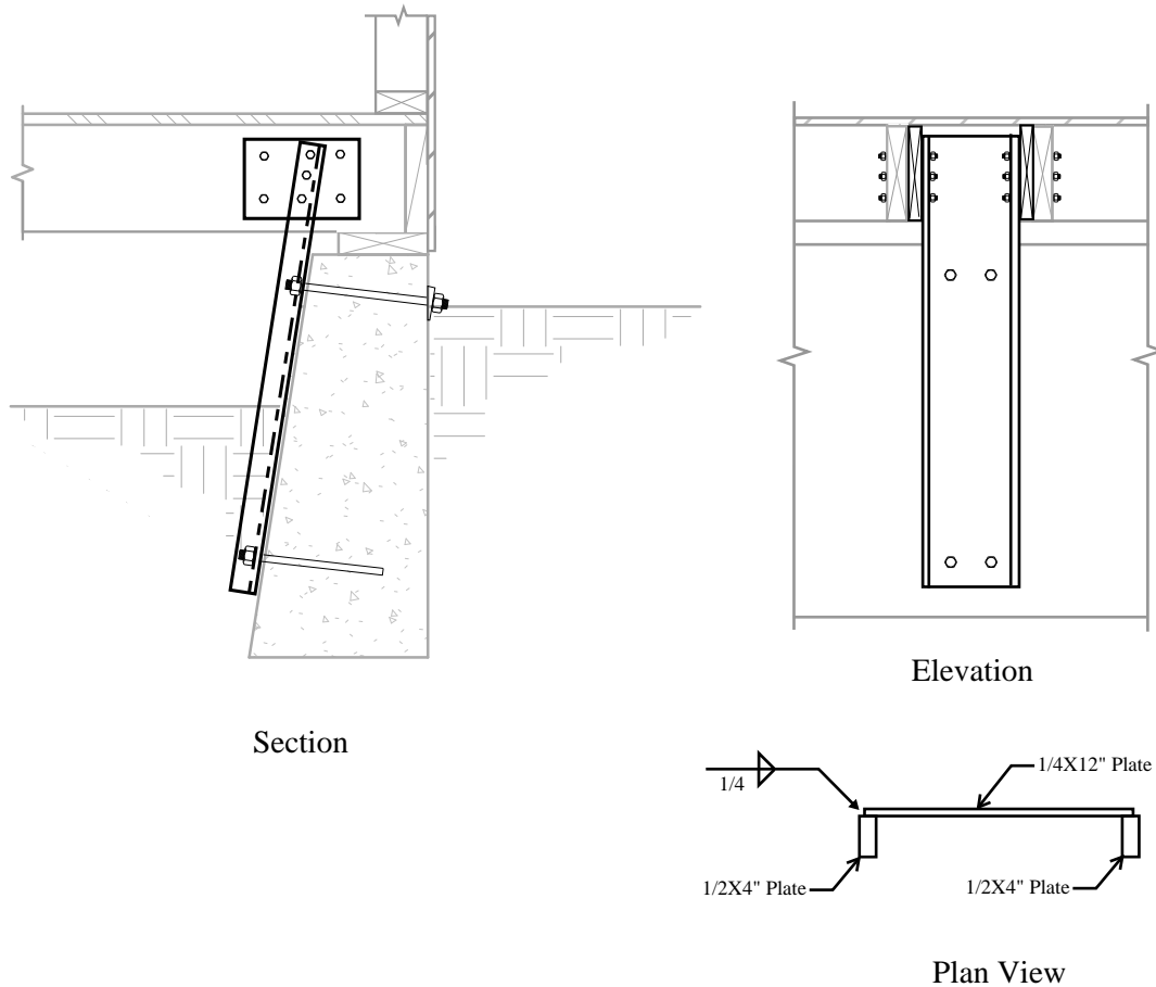
Figure 13A-31 Secondary anchor
