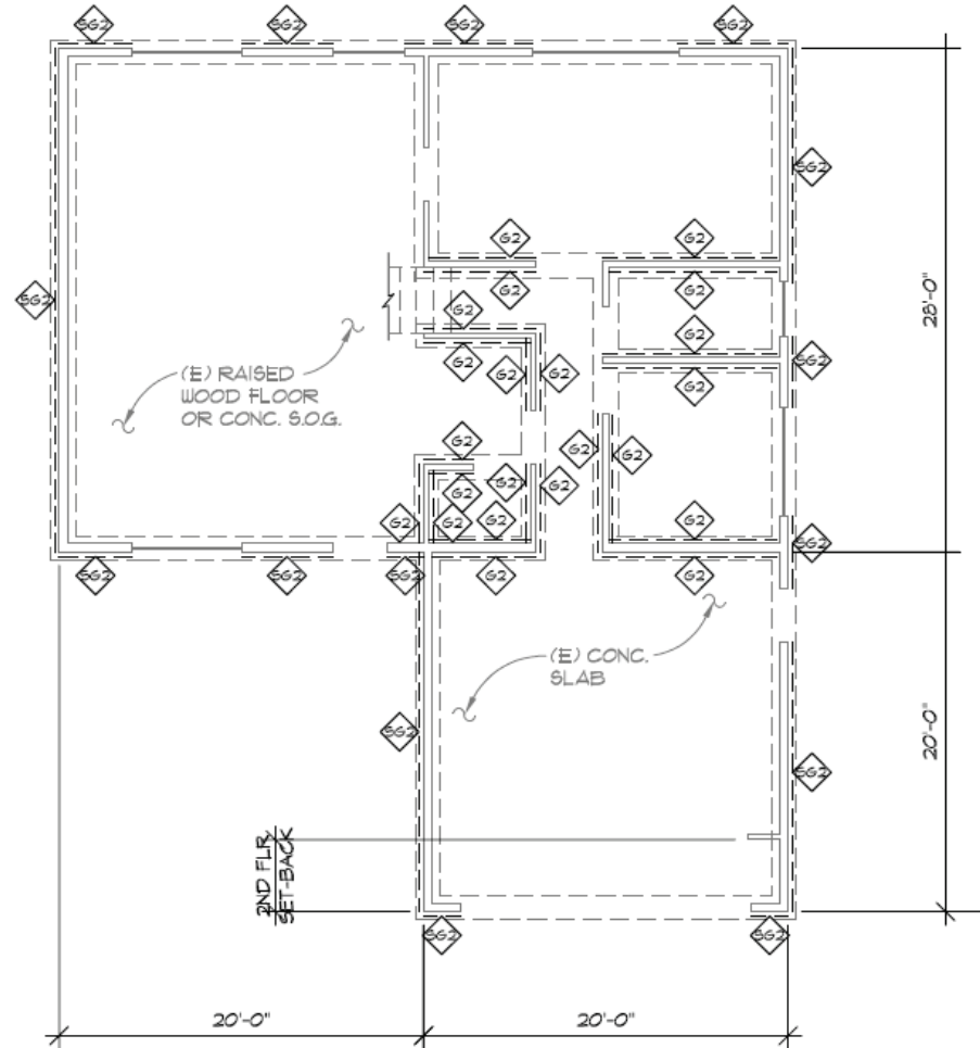
Figure 12-6 First floor plan view of existing room-over-garage configuration.
