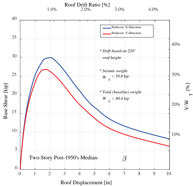
Figure 6-40 Pushover curves for the two-story post-1950's Median- \beta Superstructure (Archetype 4-2R-M \beta -E).
