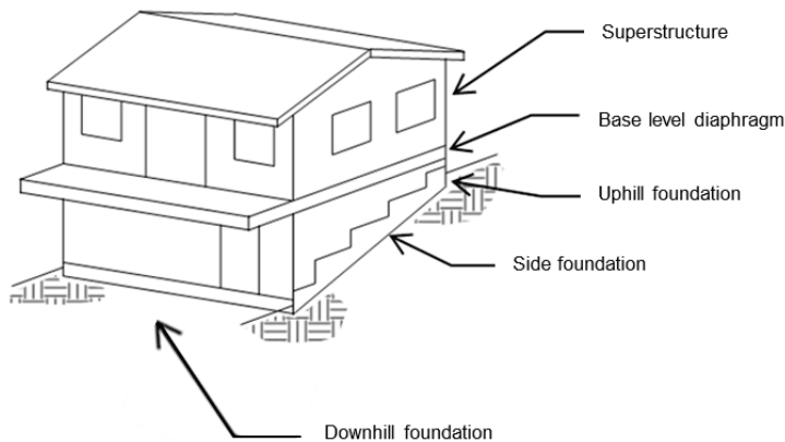
Figure 13-8 Hillside dwelling isometric with applicable terminology.
