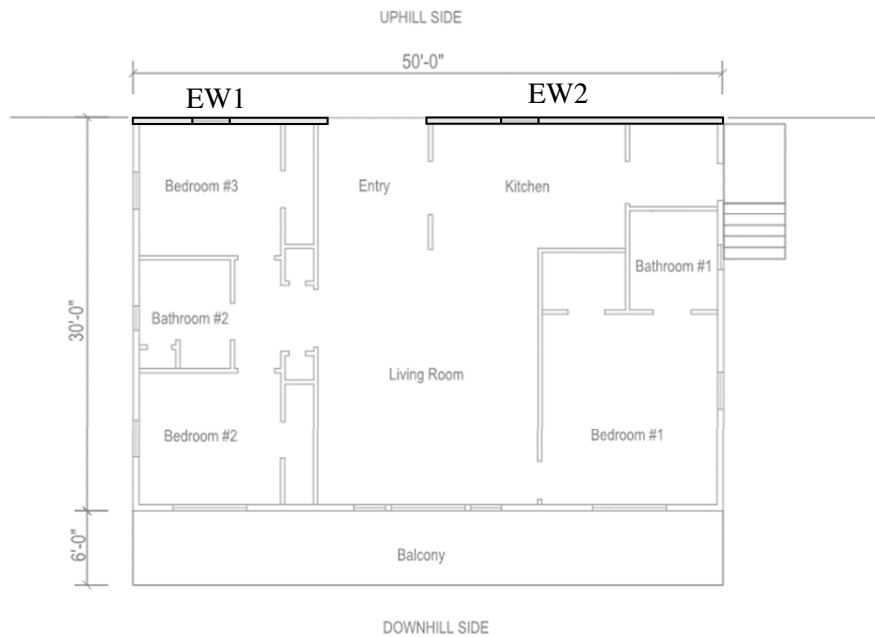
Figure 13A-43 Uphill superstructure wall location
