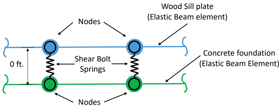
Figure 1-5 Schematic illustration of modeling of semi-rigid connectivity between the wood sill plate and the concrete foundation.
