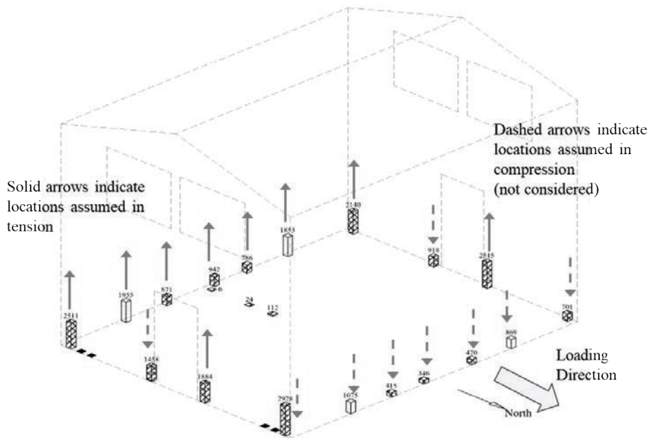
Figure 8-7 Example of anchorage elements assumed in tension for north loading: Test 8.S.4 (figure adapted from Fischer et al. (2001; 2002)).
