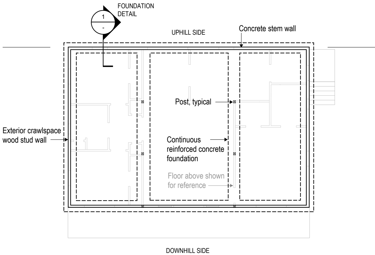
Figure 13A-3 Foundation and crawlspace plan
