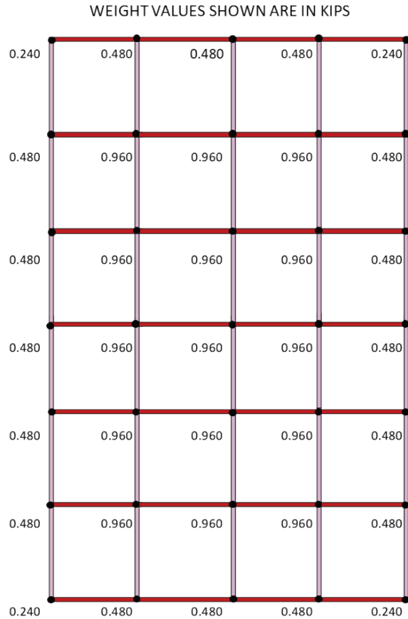
Figure 13-11 Roof diaphragm seismic weight distribution to diaphragm nodes based on tributary area.
