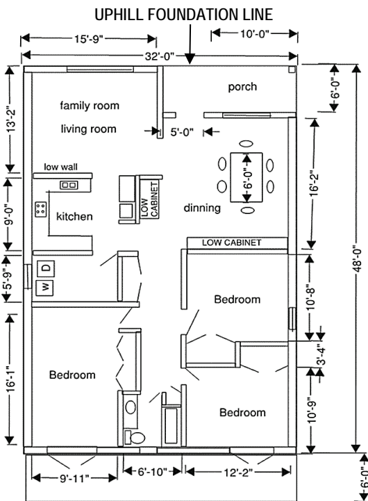
Figure 13-7 Dwelling occupied story plan for rotated model, (Model 6-1H016-M-R=M1R.)
