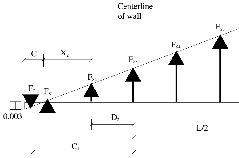
Figure 13A-19 Strain in wall plan view
