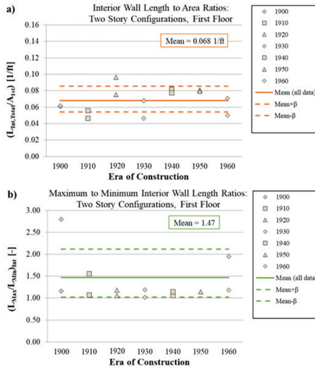
Figure 6-10 Interior wall criteria for the first floor of two-story configurations: (a) Interior wall density, (b) Maximum-to-minimum length ratio.
