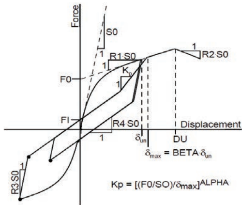
Figure 6-16 Illustration of the SAWS hysteretic model (image from Christovasilis and Filiatrault, 2009).
