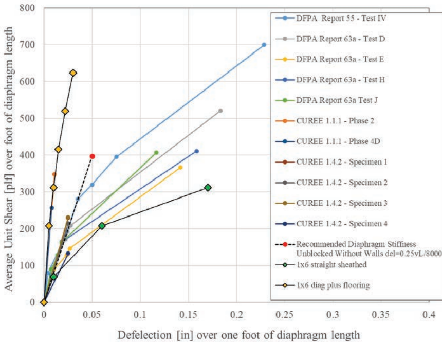
Figure 4-11 Plot of applicable test data and proposed linear stiffness of numerical description of semi-rigid diaphragms. Units are inches per foot increment of diaphragm span, plotted relative to average unit shear over that foot.
