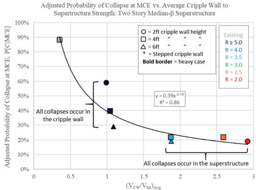
Figure 11-27 Trends of probability of collapse at the MCE intensity level versus the average cripple wall-to-superstructure strength ratio: Two-story median- \beta post-1950 superstructure.
