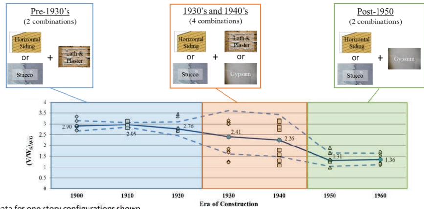
Figure 6-15 Illustration of the different building materials assumed when considering the existing building stock of cripple wall dwellings. Data shown is the average strength-to-seismic weight ratios for the one-story configurations.
