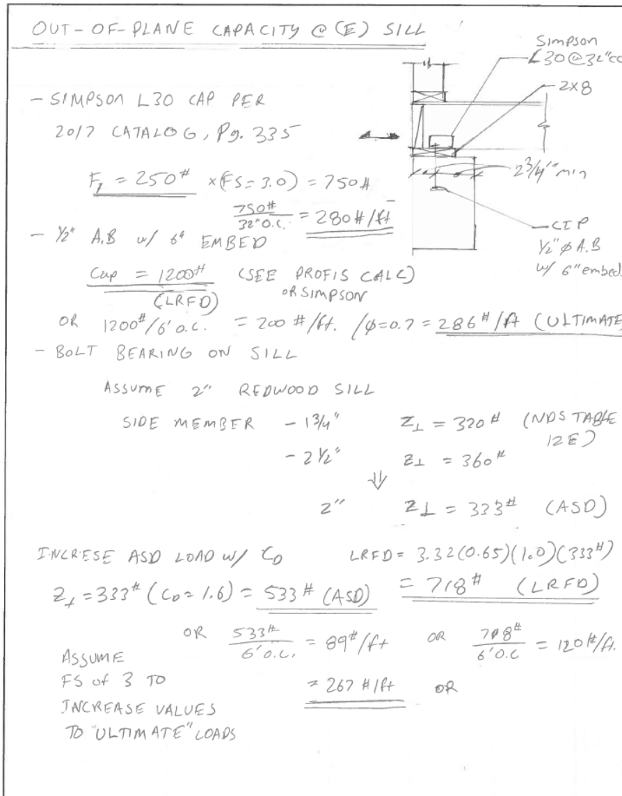
Figure 9-18 Page one of calculations for out-of-plane resistance at uphill wall line: L30 ultimate capacity, existing anchor bolt and bolt bearing on sill.
