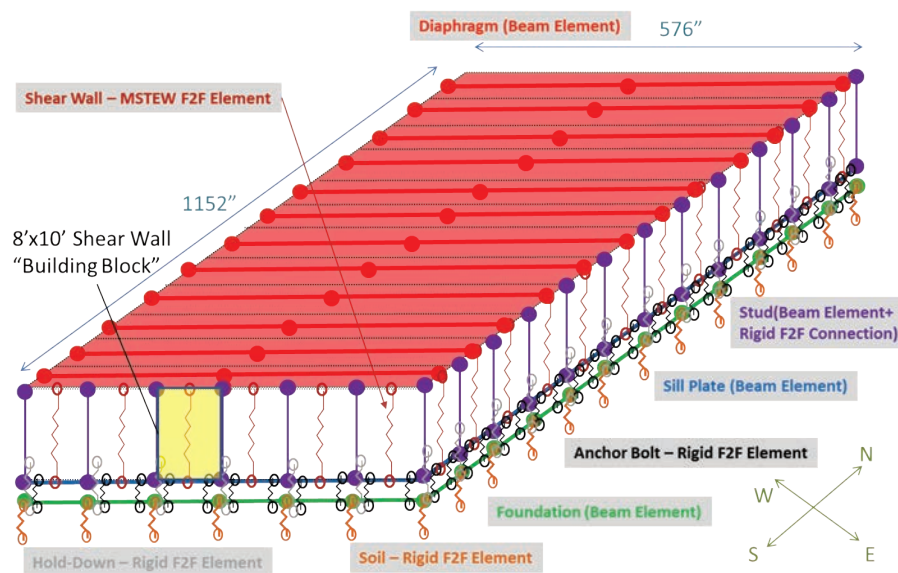
Figure 1-3 Schematic illustration of one-story, light-frame wood building model in Timber3D .
