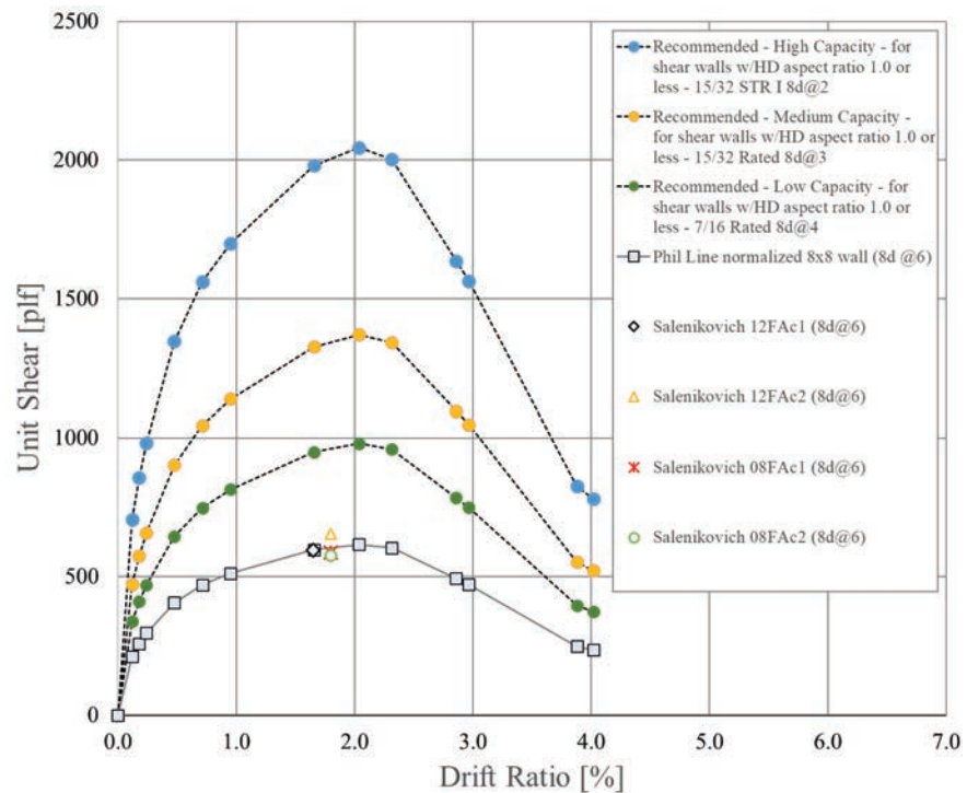
Figure 4-6 Plot of applicable test data and approximate backbone for wood structural panel shear walls with an aspect ratio of one or less and with tie-downs.
