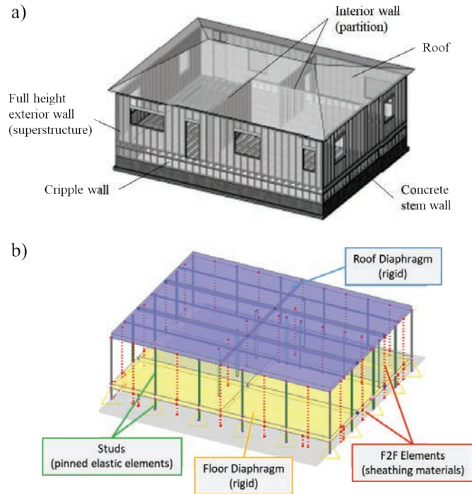
Figure 6-32 Illustration of the basic modelling components of a cripple wall dwelling: (a) Rendering and components of one-story house with two-foot tall cripple-walls; (b) Equivalent model in Timber3D .
