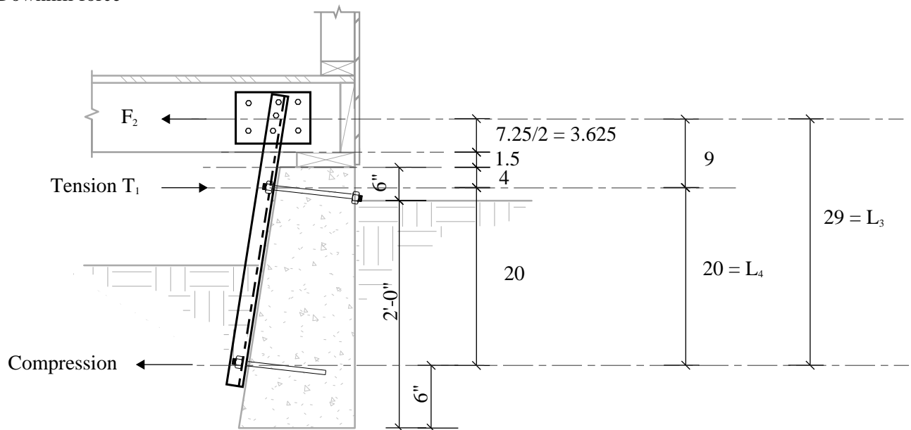
Figure 13A-34 Secondary anchor downhill force diagram
