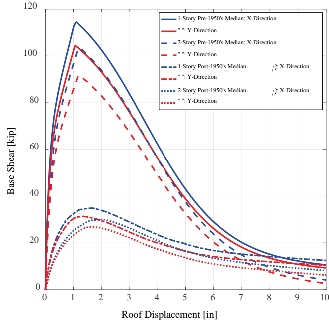
Figure 6-41 Pushover analysis comparison of all four superstructure configurations considered for cripple wall dwelling analysis.
