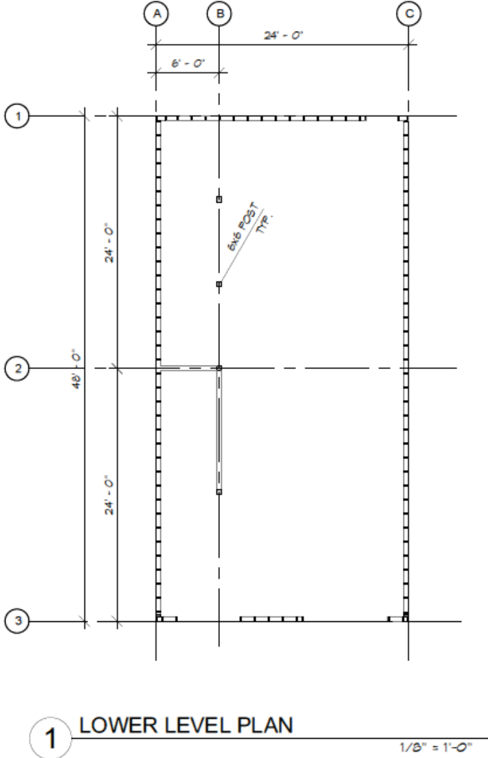
Figure 12-3 First floor plan of house-over-garage without living space at ground floor.
