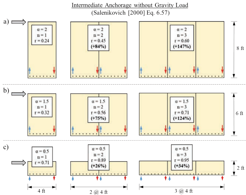
Figure 4-8 Illustration of the simplified relationship proposed by Salenikovich (2000) to account for panel aspect ratio ( \alpha ) and number of panels ( n ) to estimate the fraction of the total bottom fastener resistance developed by shear walls with intermediate anchorage ( r ). a) 8 feet by 4 feet panels (panel size tested); b), c) panel sizes common for cripple wall retrofit with heights of 6 feet and 2 feet, respectively. Percentages in bold show relative increase in normalized per linear foot capacity due to addition of panels compared to single panel.
