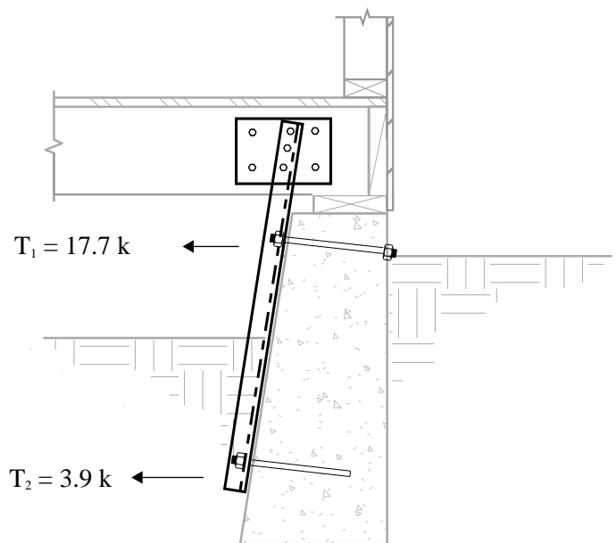
Figure 13A-35 Secondary anchor force summary
