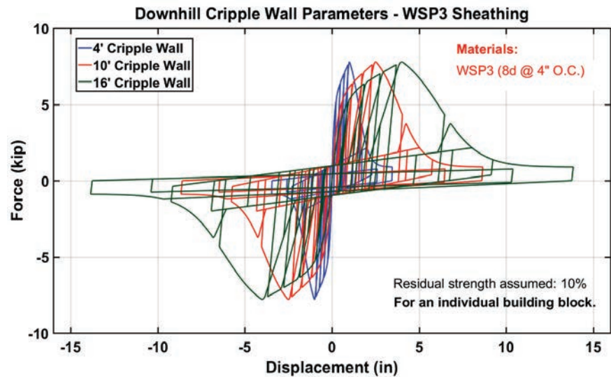
Figure 13-14 Hysteresis plots for downhill cross-slope cripple walls sheathed with WSP3 parameters.
