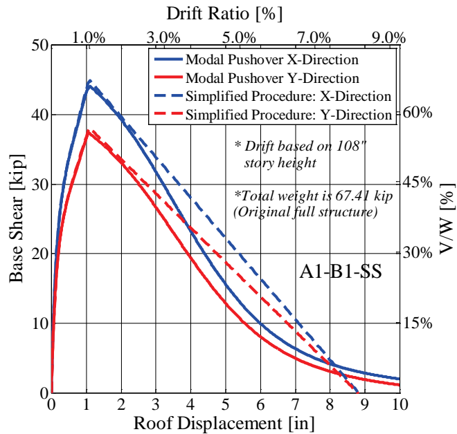
Figure 6-18 Example of simplified pushover analysis (dashed lines) and modal pushover analysis conducted in Timber3D using three-dimensional models (solid lines).
