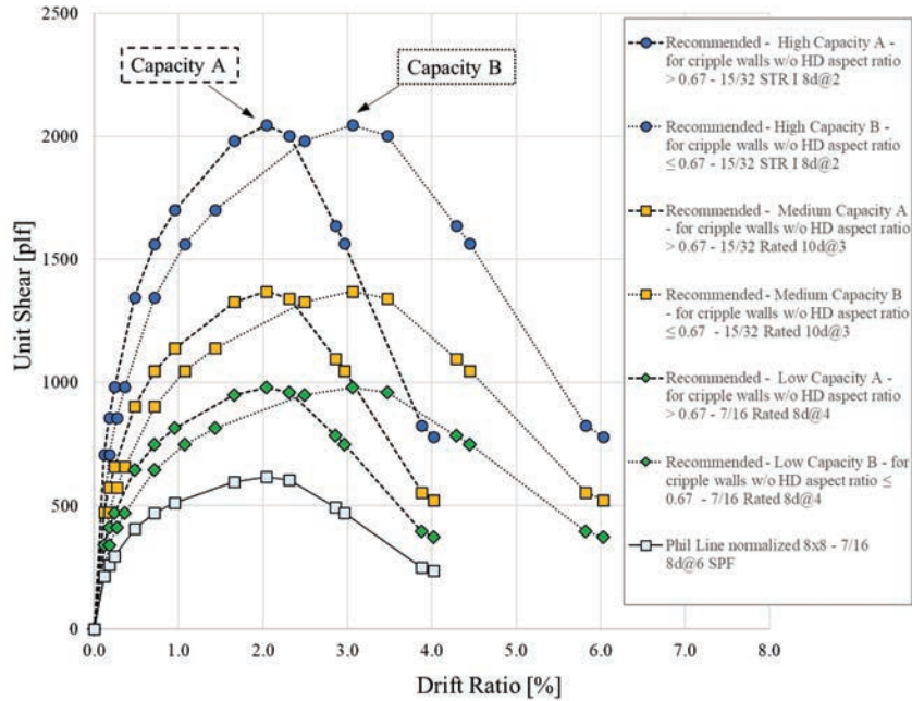
Figure 4-30 Test data and recommended backbone curves for cripple walls wood structural panels without tie downs.
