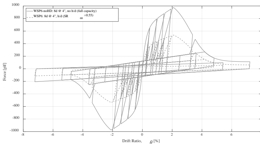
Figure 11-19 Comparison of hysteretic responses of wood structural panel WSP6 for a 6 foot tall cripple wall: No aspect ratio reduction (solid line); with aspect ratio reduction (dashed line).
