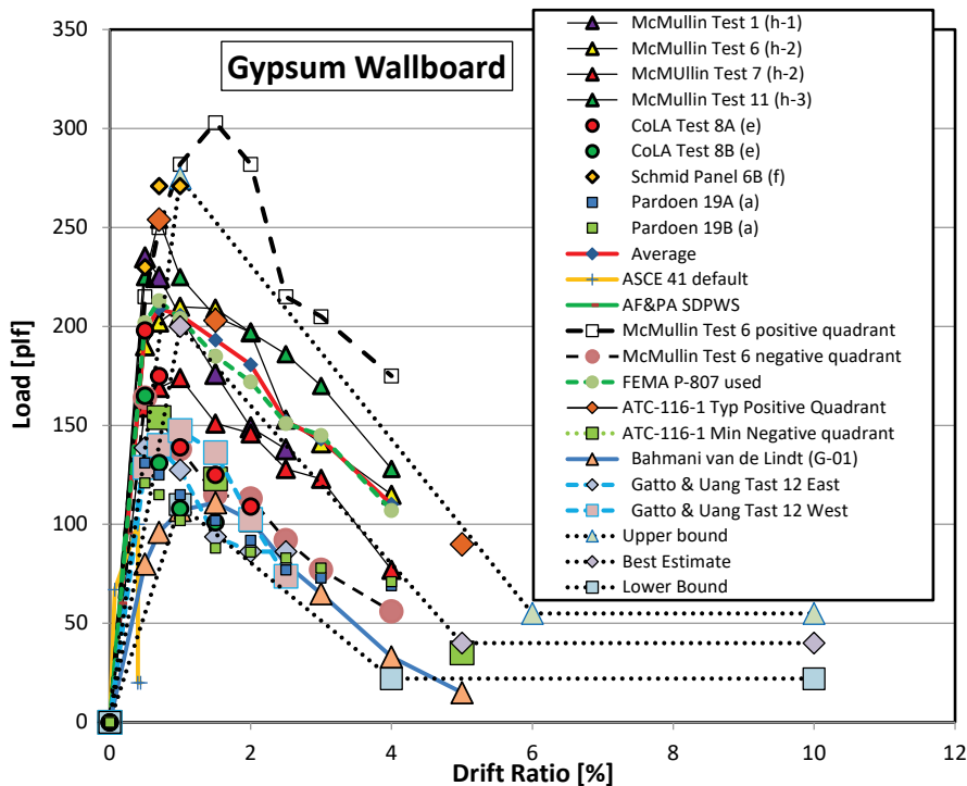
Figure 4-21 Test data and recommended backbone curves for walls sheathed with gypsum.
