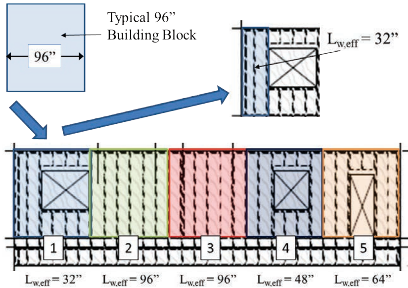
Figure 11-15 Example of the effective length assumption used for accounting for openings within building block of exterior wall lines.
