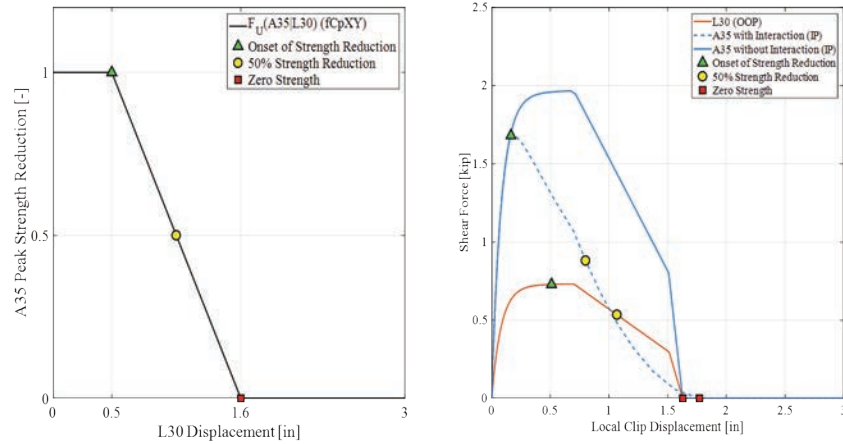
Figure 9-12 Illustration of interaction surface assumed for in-plane (IP) resistance at uphill wall line conditioned on peak out-of-plane (OOP) displacement history: example of surface (left); monotonic capacity curves (right)
