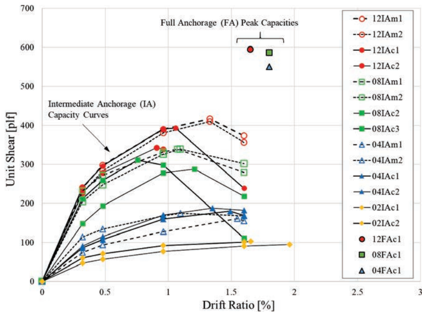
Figure 4-7 Plot of Salenikovich test data for full anchorage (FA) and intermediate anchorages (IA) of 8 feet tall walls ranging from 12 to 2 feet in length. Following the IA designation, “m” denotes monotonic loading, “c” denotes cyclic loading.
