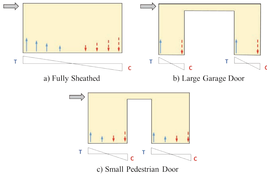
Figure 8-5 Illustration of assuming the neutral axis at the center of full-height wall segments to determine anchorage locations in tension for a direction of loading: a) fully sheathed wall, b) large garage door, c) small pedestrian door.
