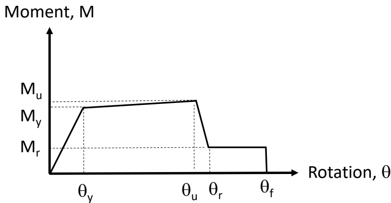
Figure 1-12 Generalized illustration of inelastic moment-rotation relationship for F2F rotational link elements.
