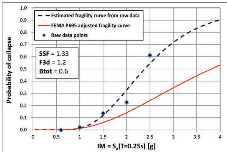
Figure 13-22 Example of an estimated raw data fragility curve being modified with FEMA P695's various seismic performance factors.
