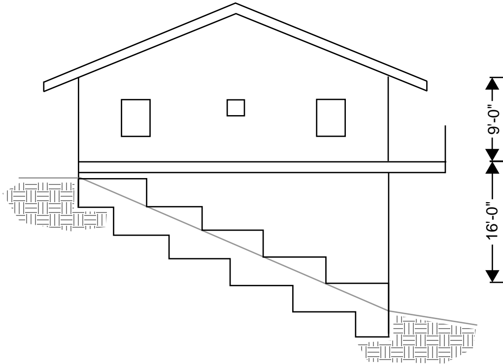
Figure 13A-6 Cross slope elevation
