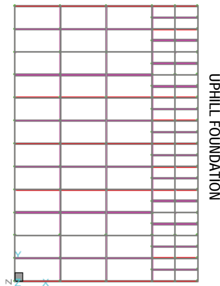
Figure 13-19 Diaphragm mesh for an example hillside model.
