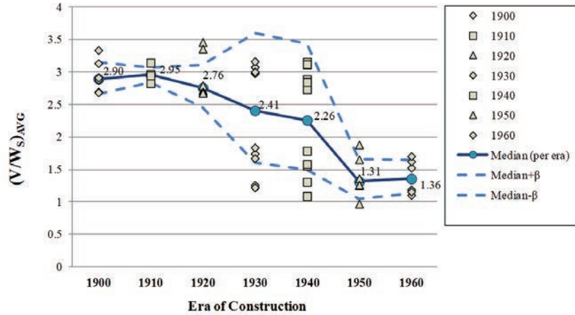
Figure 6-21 Strength-to-seismic weight ratios for one-story configurations.
