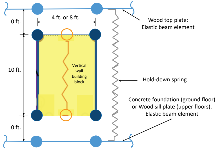
Figure 1-7 Schematic illustration of modeling of semi-rigid connectivity introduced by hold-down rods.
