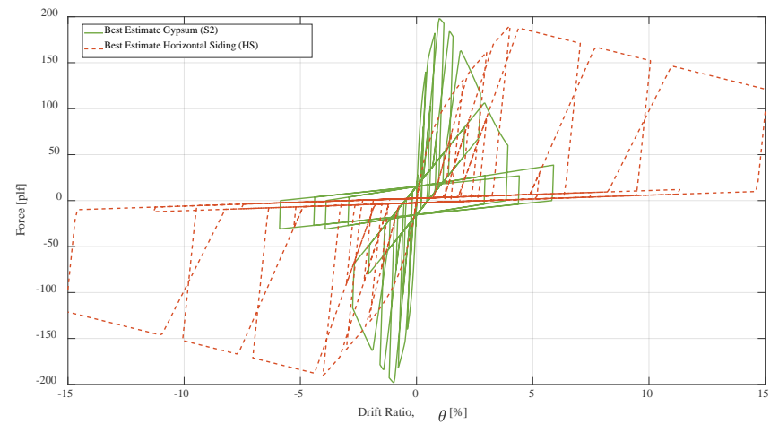
Figure 11-13 Assumed hysteretic behavior for best estimate gypsum wallboard (solid line) and horizontal wood siding (dashed line).
