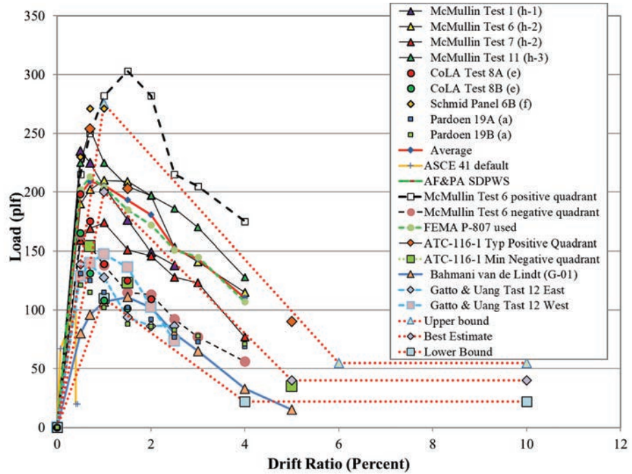
Figure 4-2 Plot of applicable test data and approximate backbone for gypsum wallboard.
