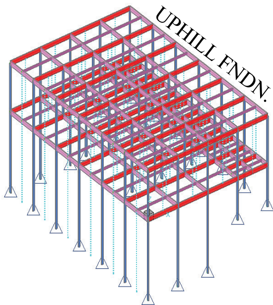
Figure 13-12 Example 0'-16' hillside retrofit model in Timber3D.
