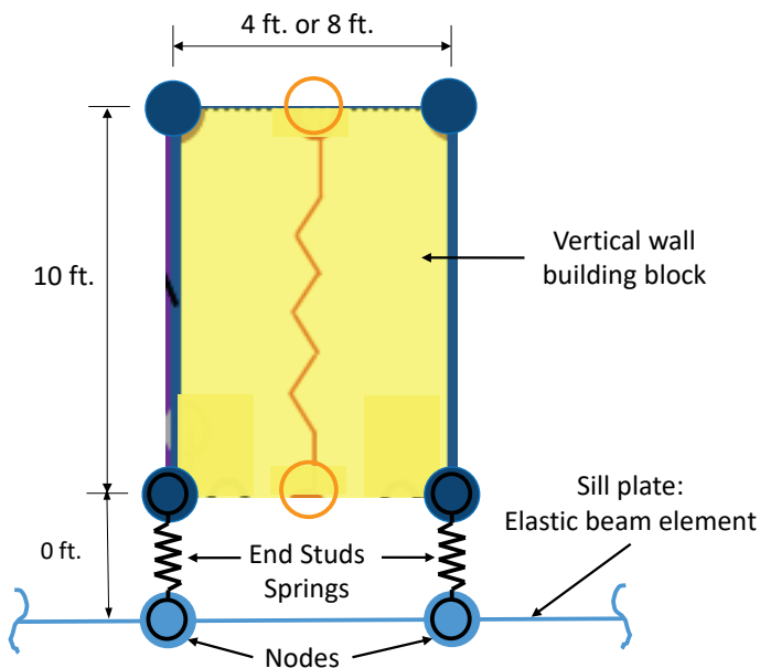
Figure 1-6 Schematic illustration of modeling of semi-rigid connectivity between the end studs and the sill plate.
