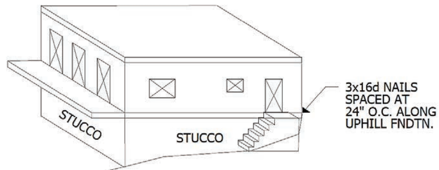
Figure 13-23 Existing model (6-1H04-M-E) crawl space configuration.
