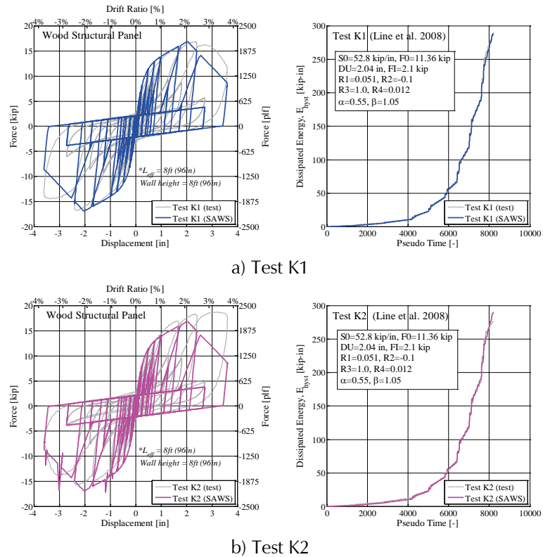
Figure 4-31 Comparison of hysteretic response and cumulative dissipated energy for test data (Line et al., 2008) and optimized CUREE parameters (see Table 4-9) for wood structural panels.
