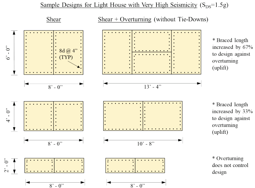
Figure 4-9 Illustration of different wood structural panel brace length requirements when designing cripple wall retrofits of various heights with intermediate anchorage: shear only (left); shear and overturning (right). Wall lengths would be applied in every corner and side of the dwelling. Designs on the right would represent those modeled in numerical studies for the given dwelling and site.
