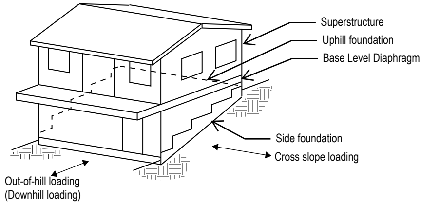
Figure 13A-8 Hillside dwelling isometric with applicable terminology
