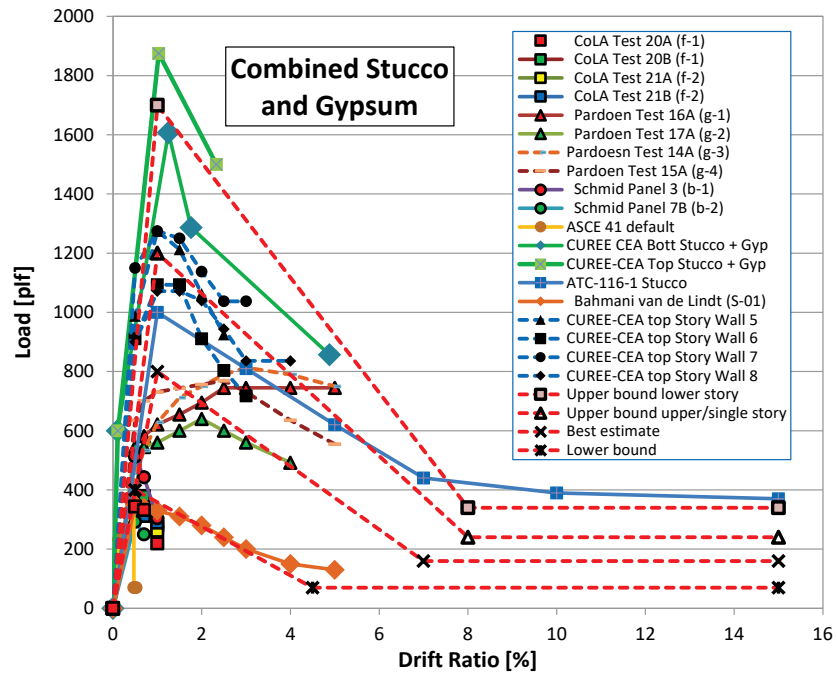
Figure 4-23 Test data and recommended backbone curves for walls sheathed with a combination of interior gypsum and exterior stucco.
