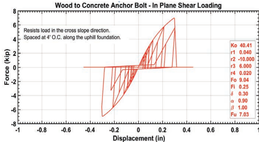
Figure 13-18 Shear anchor parameters for Model 6-1H04-M-R=1.
