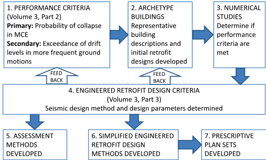
Figure 2-1 Relating performance criteria to assessment and retrofit criteria.
