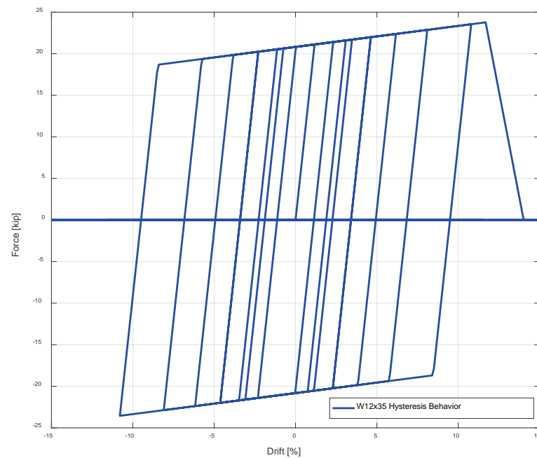
Figure 12-21 Hysteresis behavior of W12×35 steel retrofit.
