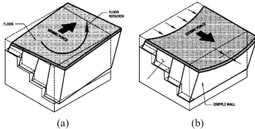
Figure 9-1 Short cripple wall at the uphill side of the dwelling in combination with the tall downhill cripple wall: (a) illustrates cross-slope loading, with rotation of the diaphragm resulting in the floor diaphragm pulling away from the uphill foundation; (b) illustrates direct out-of-hill loading.
