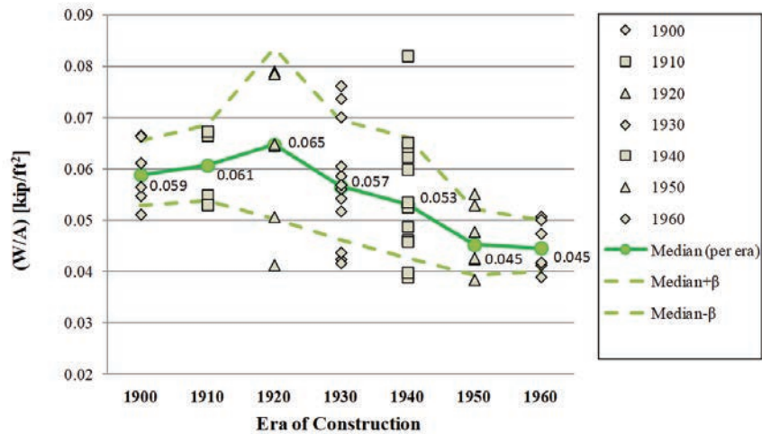
Figure 6-19 Total weight-to-plan area ratios for one-story configurations.
