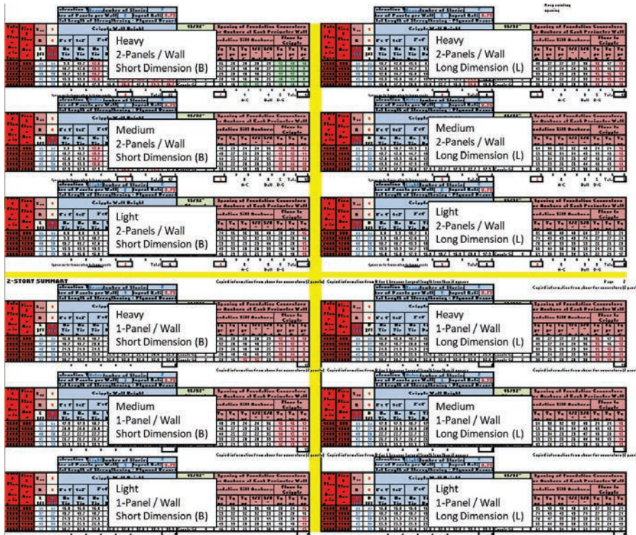
Figure 11-32 Example of constructability tables for all weight combinations, plan dimensions, and number of sheathed panels per wall line. (Tables for two-story cases with an S_{DS}=1.0g and R=4 shown. Only 2-Panel solutions were included in plan set.)
