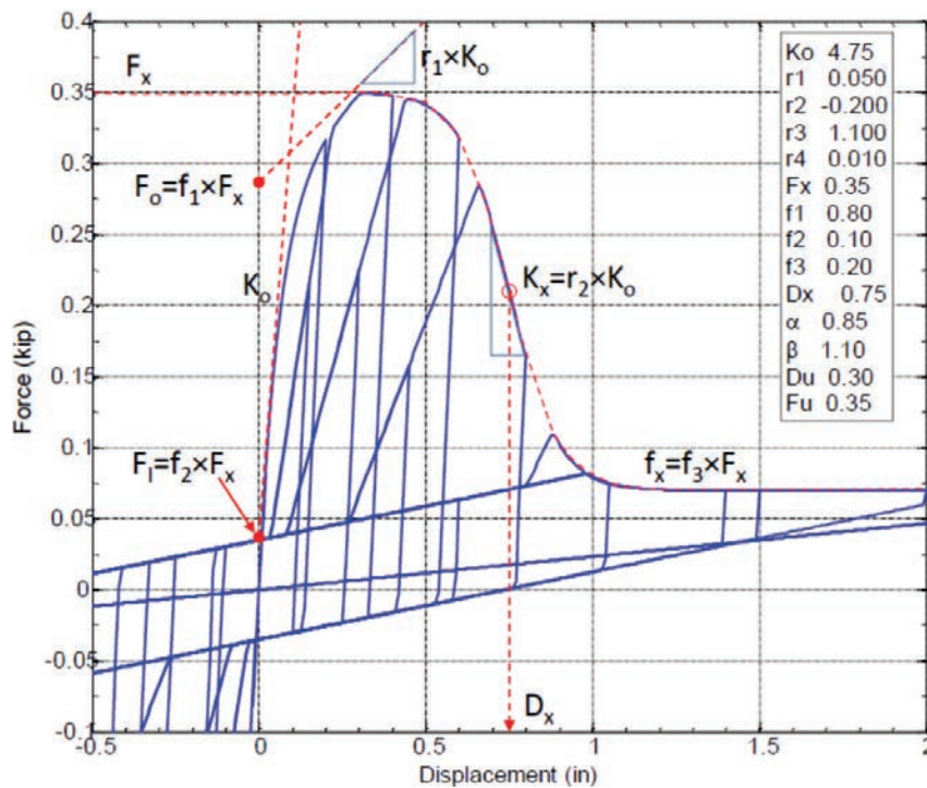
Figure 12-12 Illustration of the residual strength (RESST) hysteretic model used in Timber3D for modeling the behavior of wall materials.
