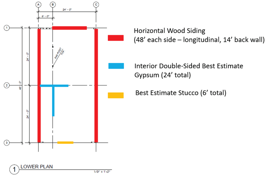
Figure 12-7 Typical existing wall layouts for the first story of HOG configurations.
