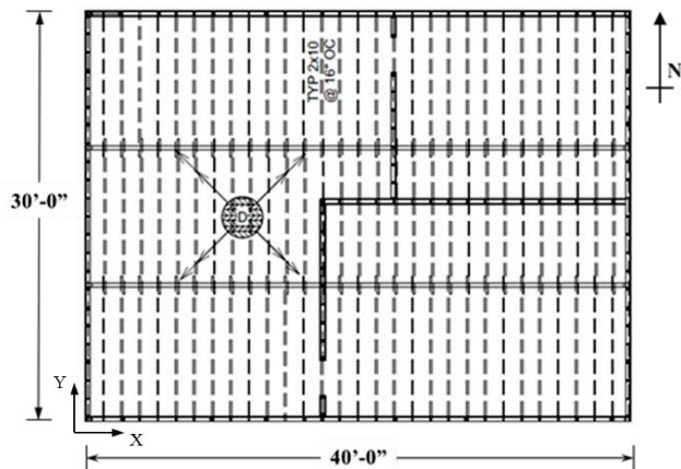
Figure 11-7 Plan view of the one- and two-story baseline configurations selected for modeling of cripple wall dwellings. Note: axes shown are used throughout the crawlspace dwelling analysis.
