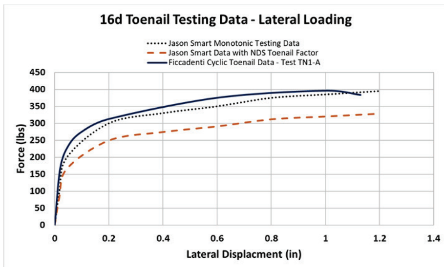
Figure 4-14 Plot of applicable test data and load-deflection behavior for a single 16d common toenail/nail in shear.
