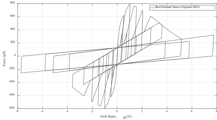
Figure 11-11 Assumed hysteretic behavior for stucco plus gypsum wallboard.
