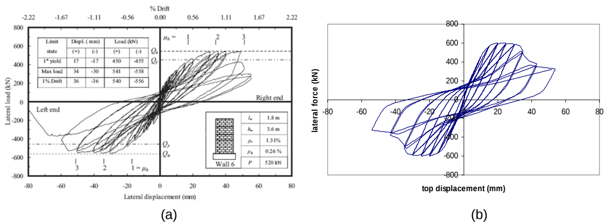
Figure A-8 Lateral load versus displacement curves for Specimen 6 tested by Shedid et al. (2008): (a) experimental results; (b) analytical model.
