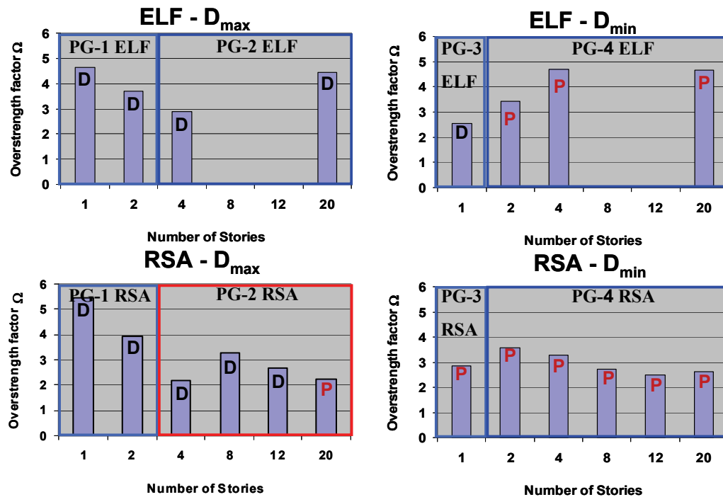
Figure 6-10 Graphical representation of overstrength factor for all archetypes.
