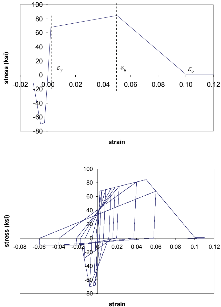
Figure 3-6 Reference stress-strain relations used for reinforcing steel: backbone curve (top) and cyclic loading and unloading curves (bottom).
