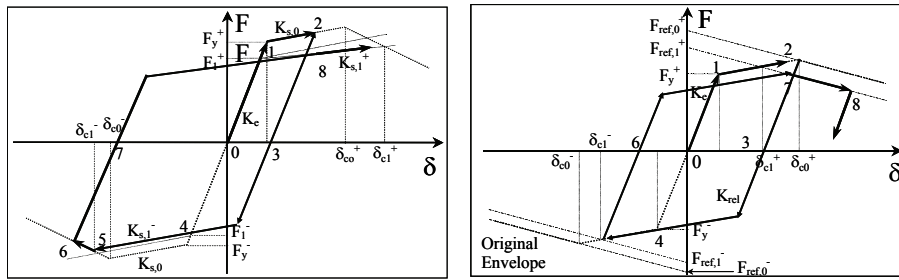
Figure 6-5 Basic and post-capping strength deterioration.
