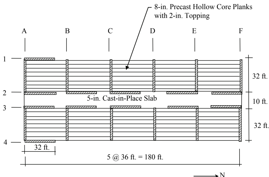
Figure 3-2 Plan view of typical multistory reinforced masonry shear wall building configuration (design for 12-story SDC D_{max} shown).
