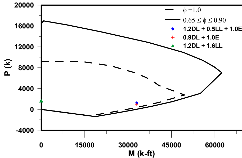
Figure B-1 Axial load-moment ( P - M ) interaction diagram for Archetype 12.
