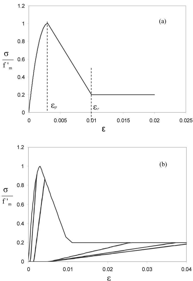
Figure 3-5 Normalized reference stress-strain curves used for compressive behavior of masonry: backbone curve (top) and cyclic loading and unloading curves (bottom).
