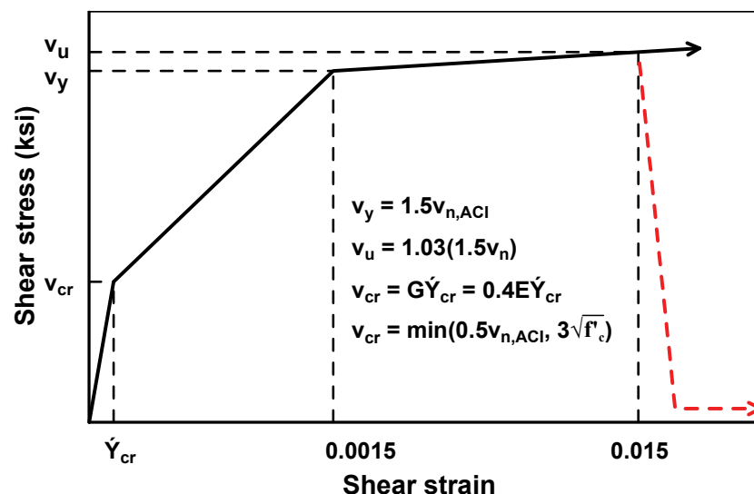
Figure 4-5 Generalized shear model adapted from ASCE/SEI 41-06.
