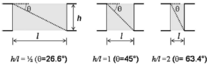
Figure B-4 Wall pier geometry and critical crack angles (Wallace et al., 2008).
