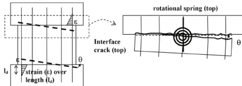
Figure 4-4 Rotational spring model for reinforcing steel extension and slip (Massone et al., 2009).
