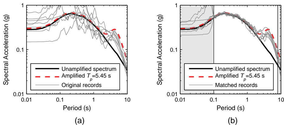
Figure B-25 Comparison of target spectrum unamplified for velocity pulses and spectrum with narrow-band adjustment for T_p=5.45\text{s} velocity pulse with record spectra: (a) before and (b) after matching. Unshaded period range was considered in matching.
