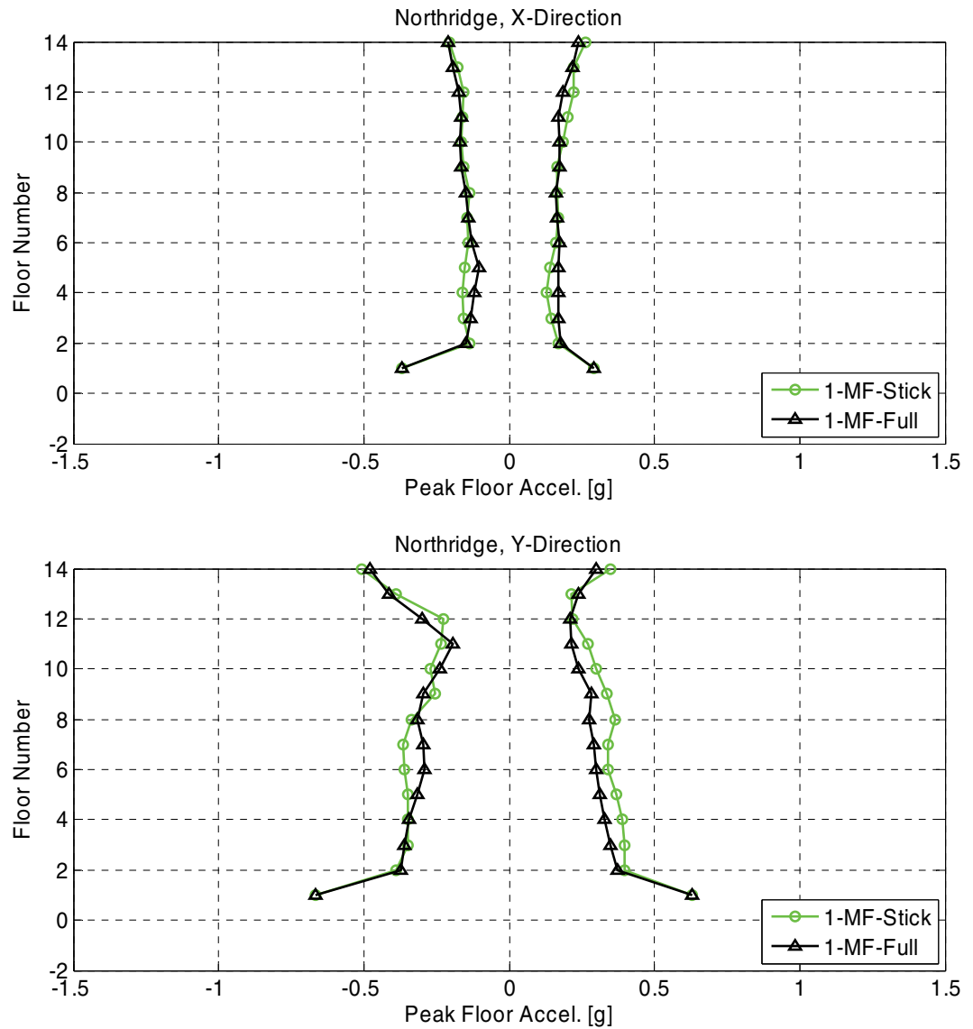
Figure B-15 Comparison of peak floor acceleration envelopes for the moment frame stick Model 1 and the full-building Model 1.
