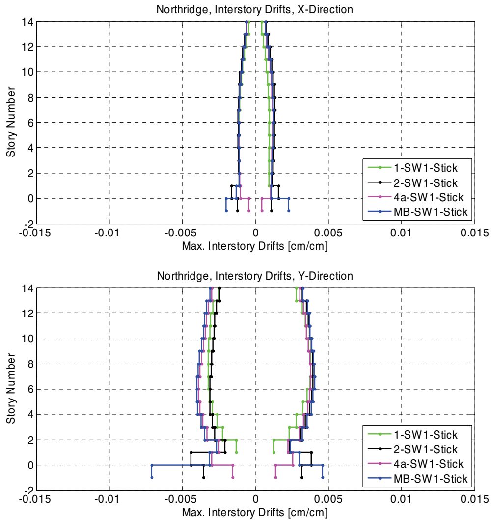
Figure B-33 Comparison of maximum story drift envelopes for the SW1 stick Models 1, 2, 4a, and MB.
