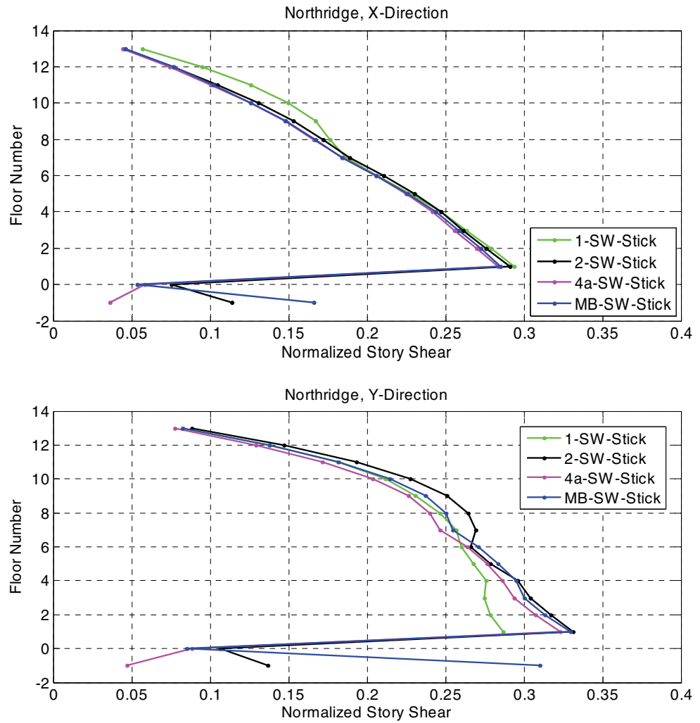
Figure B-30 Comparison of normalized story shear envelopes for the SW stick Models 1, 2, 4a, and MB.
