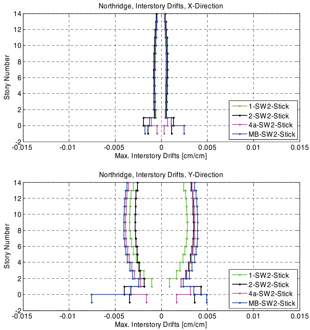
Figure B-37 Comparison of maximum story drift envelopes for the SW2 stick Models 1, 2, 4a, and MB.
