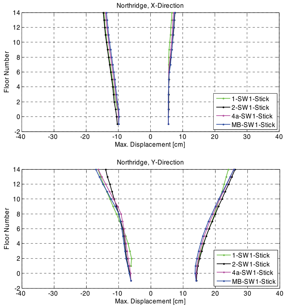
Figure B-32 Comparison of maximum displacement envelopes for the SW1 stick Models 1, 2, 4a, and MB.
