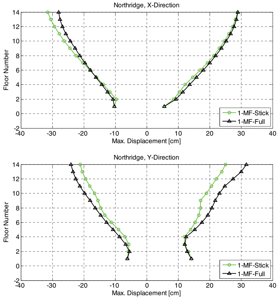
Figure B-12 Comparison of maximum displacement envelopes for the moment frame stick Model 1 and the full-building Model 1.
