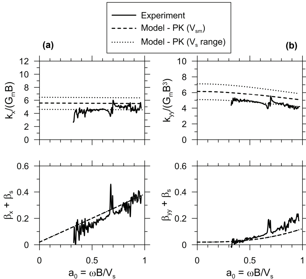
Figure 5-2 Normalized impedance values from experimental data compared with theoretical predictions for the Garner Valley site for: (a) translational; and (b) rotational modes (adapted from Tileylioglu et al., 2011). Velocity, V_{sm} , and modulus, G_m , denote median values from test data.
