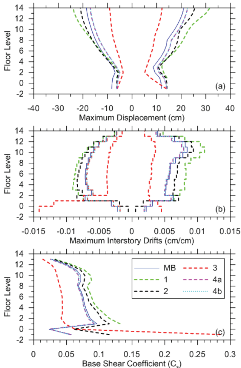
Figure 7-16 Comparison of peak displacements, drift ratios, and story shears from all model configurations, in the transverse direction.
