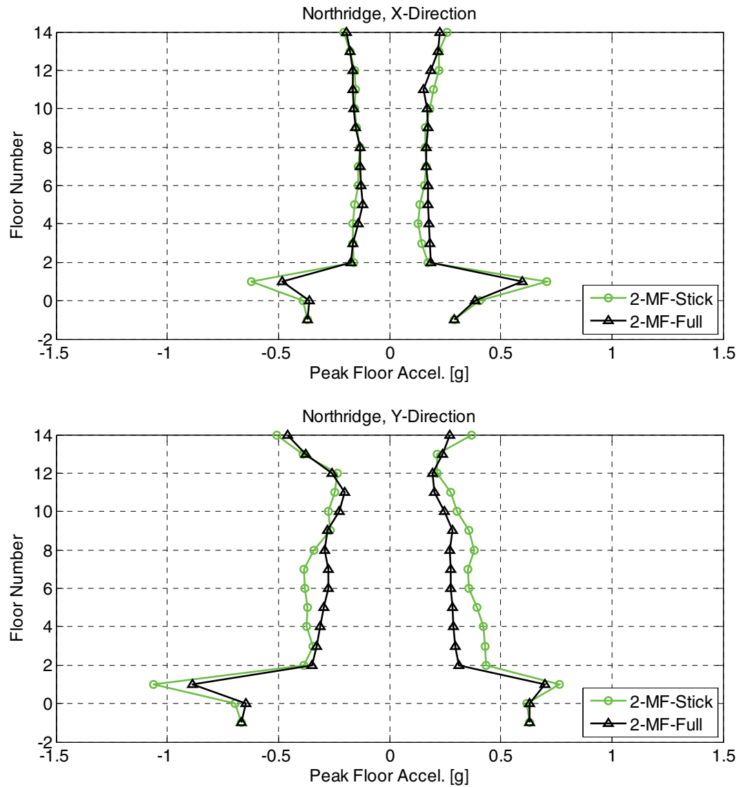
Figure B-19 Comparison of peak floor acceleration envelopes for the moment frame stick Model 2 and the full-building Model 2.
