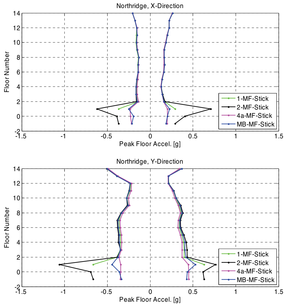
Figure B-27 Comparison of peak floor acceleration envelopes for the moment frame stick Models 1, 2, 4a, and MB.
