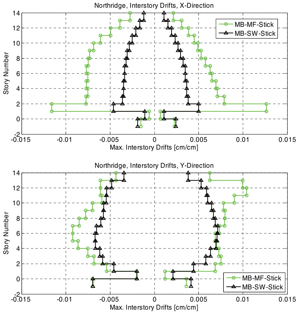
Figure B-45 Comparison of maximum story drift envelopes for the moment frame stick Model MB and the shear wall stick Model MB.
