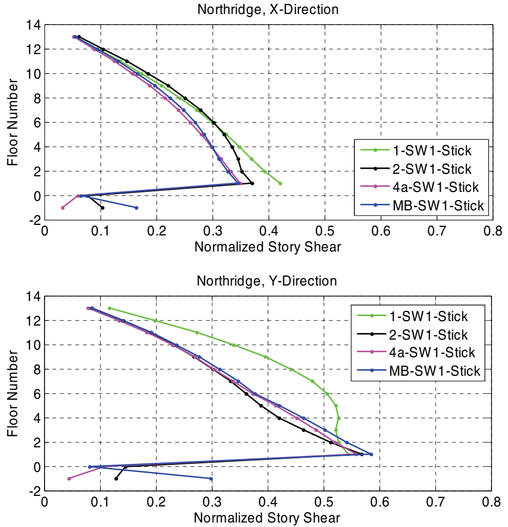
Figure B-34 Comparison of normalized story shear envelopes for the SW1 stick Models 1, 2, 4a, and MB.
