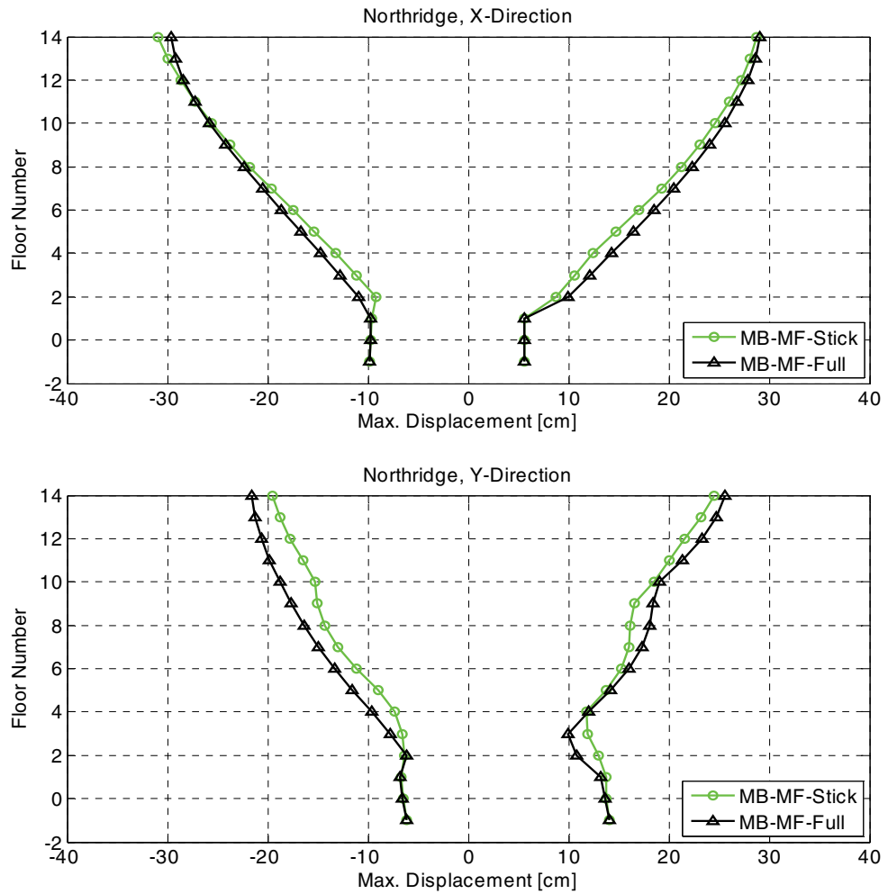
Figure B-8 Comparison of maximum displacement envelopes for the moment frame stick Model MB and the full-building Model MB.
