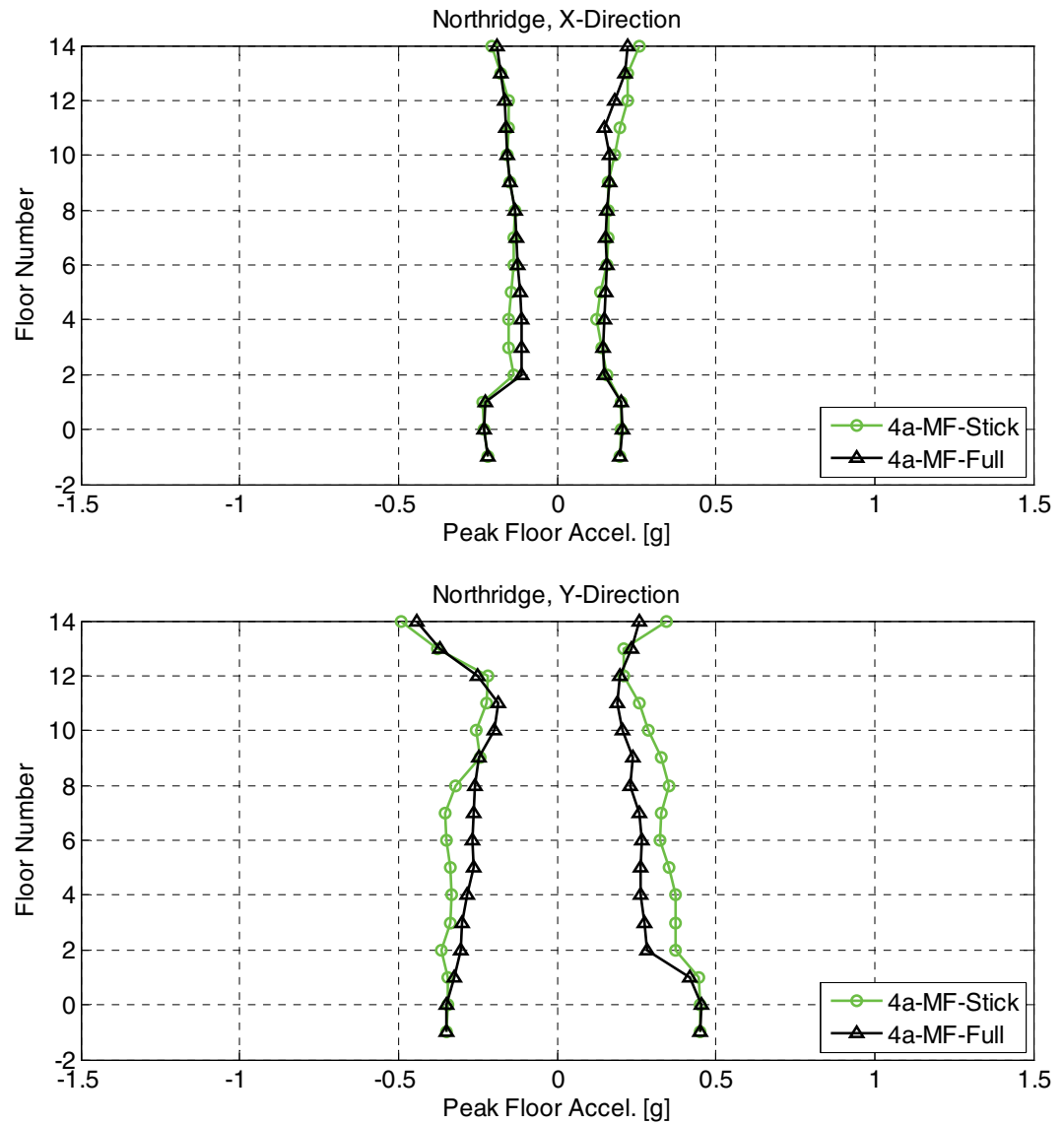
Figure B-23 Comparison of peak floor acceleration envelopes for the moment frame stick Model 4a and the full-building Model 4a.
