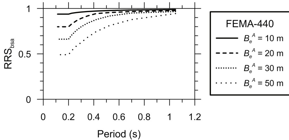
Figure 4-5 Ratios of response spectra ( u_{FIM}/u_g ) for base slab averaging using the semi-empirical formulation adopted in FEMA 440.
