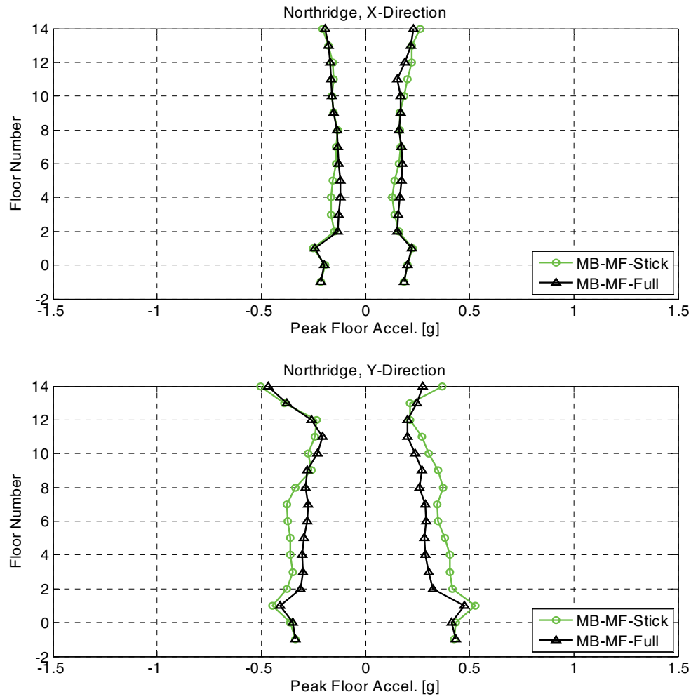
Figure B-11 Comparison of peak floor acceleration envelopes for the moment frame stick Model MB and the full-building Model MB.
