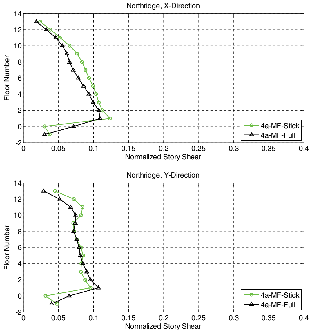
Figure B-22 Comparison of normalized story shear envelopes for the moment frame stick Model 4a and the full-building Model 4a.
