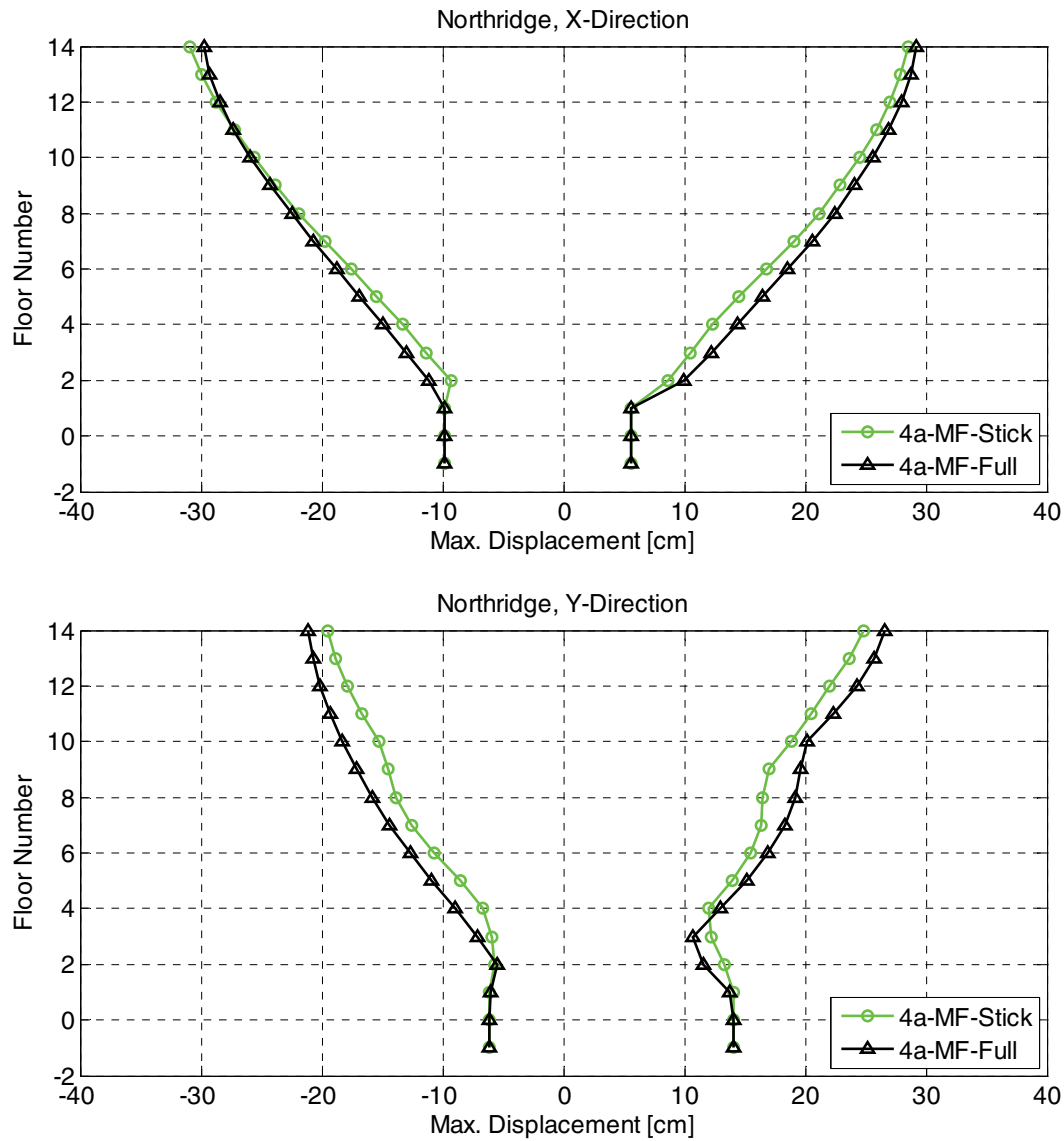
Figure B-20 Comparison of maximum displacement envelopes for the moment frame stick Model 4a and the full-building Model 4a.
