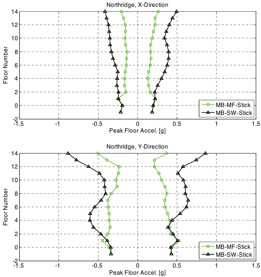
Figure B-47 Comparison of peak floor acceleration envelopes for the moment frame stick Model MB and the shear wall stick Model MB.
