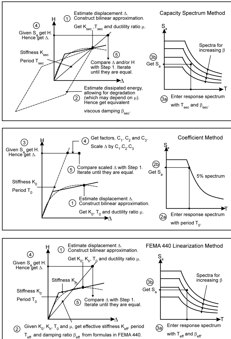
Figure 4-4 Schematic illustration of procedures used to combine pushover curves with design response spectra to estimate seismic displacements in a structure (Powell, 2006, with permission).
