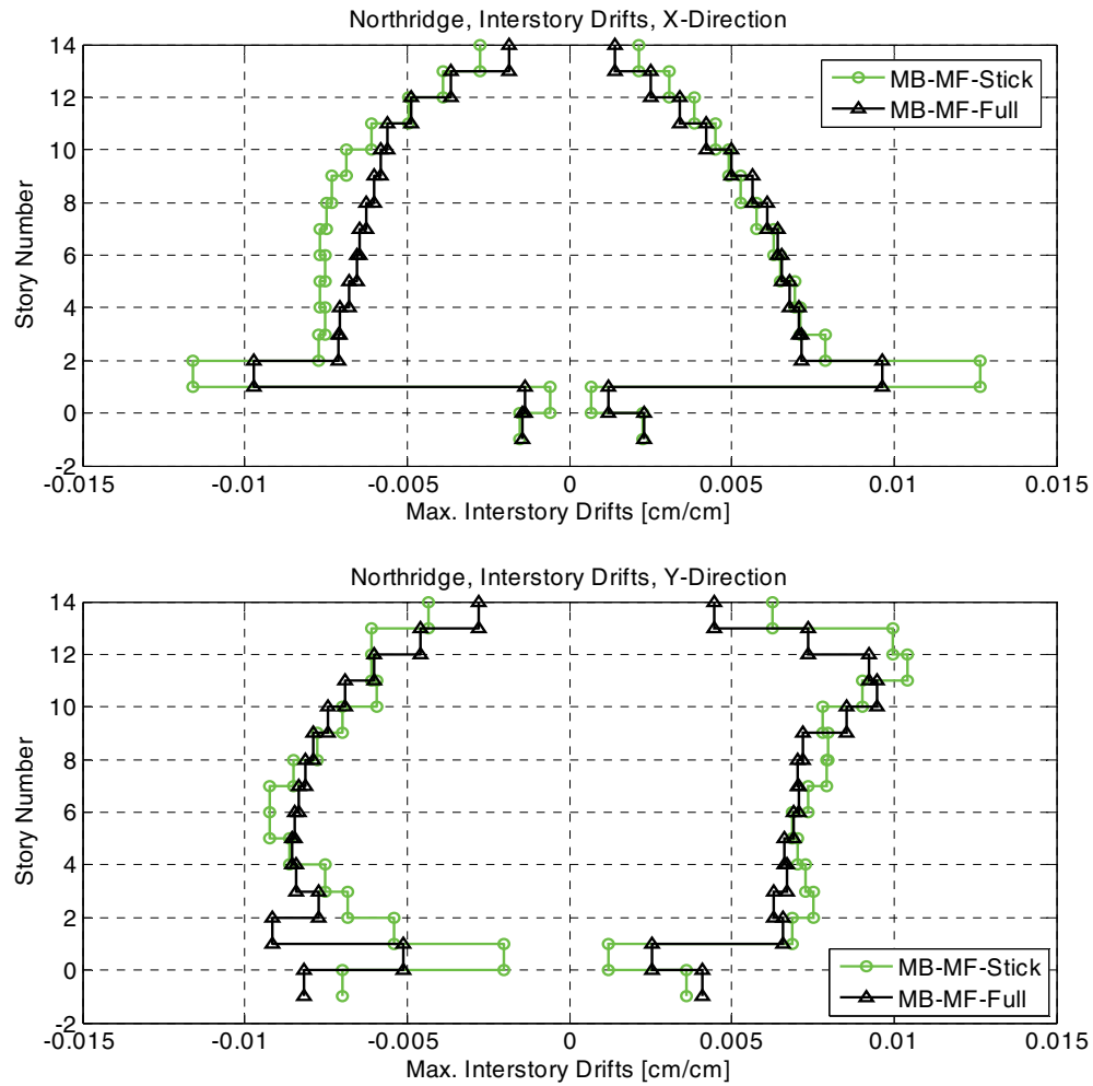
Figure B-9 Comparison of maximum story drift envelopes for the moment frame stick Model MB and the full-building Model MB.
