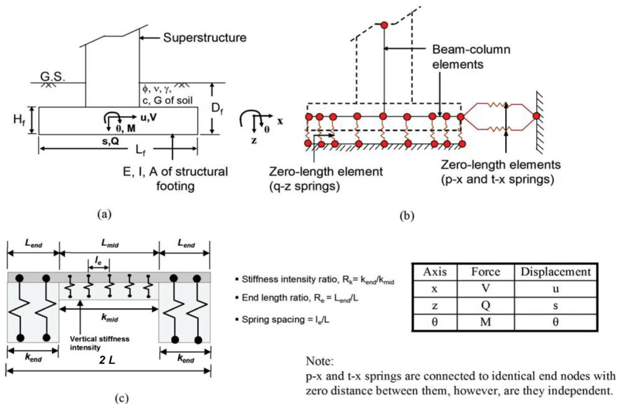
Figure 2-13 Schematic illustration of a Beam-on-Nonlinear Winkler Foundation (BNWF) model: (a) hypothesized foundation-superstructure system; (b) idealized model; and (c) variable vertical stiffness distribution (Raychowdhury and Hutchinson, 2009, with permission).
