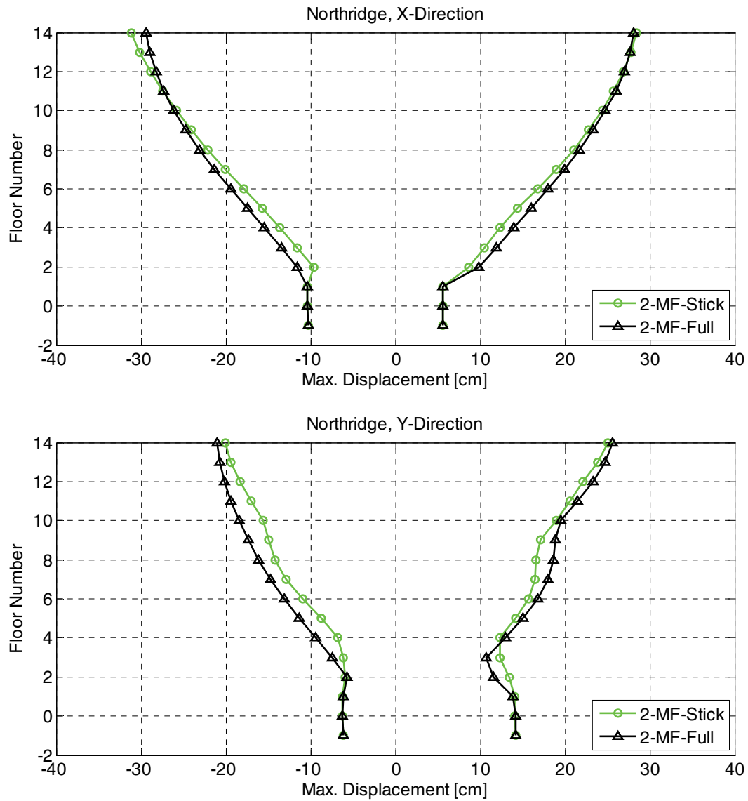
Figure B-16 Comparison of maximum displacement envelopes for the moment frame stick Model 2 and the full-building Model 2.
