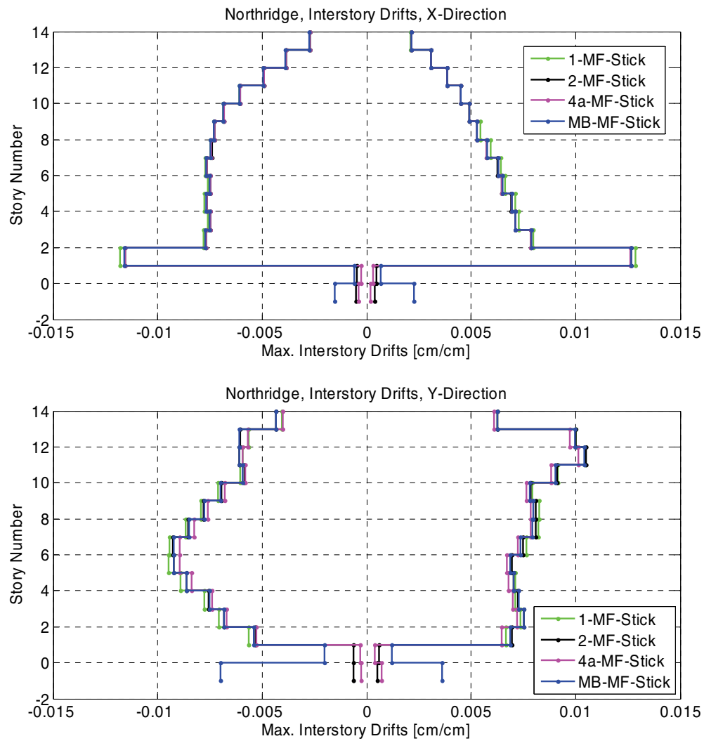
Figure B-25 Comparison of maximum story drift envelopes for the moment frame stick Models 1, 2, 4a, and MB.
