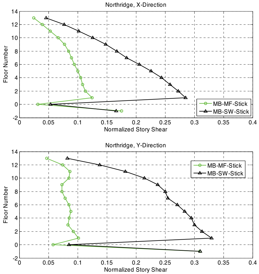
Figure B-46 Comparison of normalized story shear envelopes for the moment frame stick Model MB and the shear wall stick Model MB.
