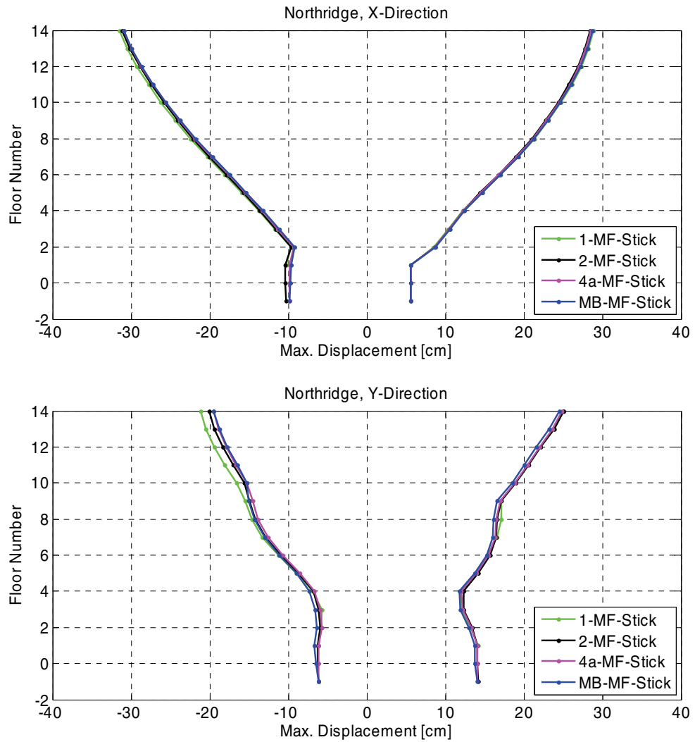
Figure B-24 Comparison of maximum displacement envelopes for the moment frame stick Models 1, 2, 4a, and MB.
