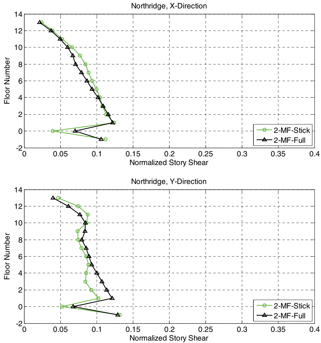
Figure B-18 Comparison of normalized story shear envelopes for the moment frame stick Model 2 and the full-building Model 2.
