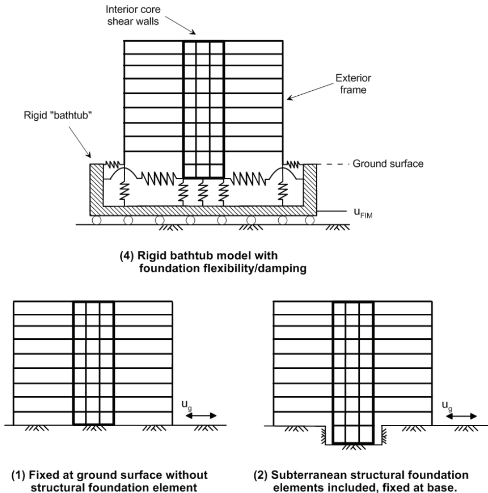
Figure 7-30 Schematic illustration of Model 4 (bathtub); Model 2 (fixed at foundation level); and Model 1 (fixed at ground surface) for the Walnut Creek building.
