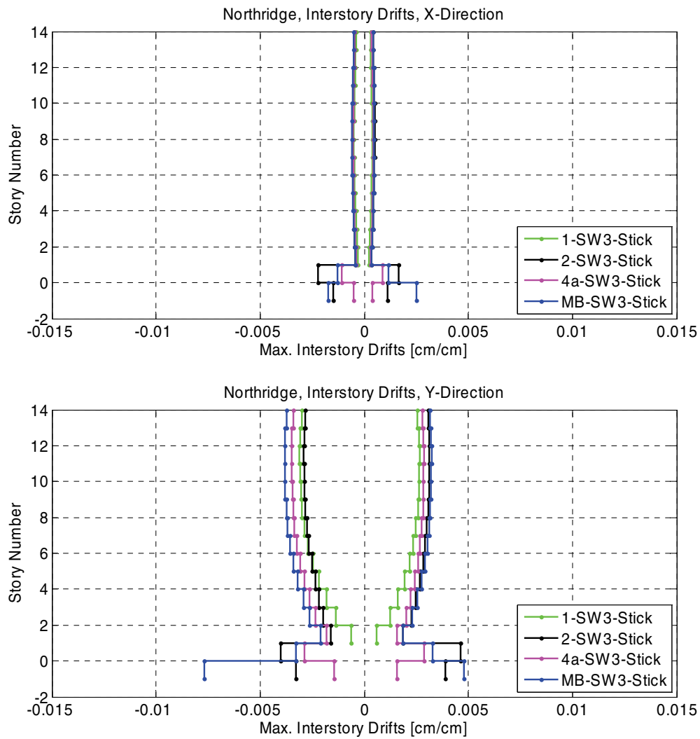
Figure B-41 Comparison of maximum story drift envelopes for the SW3 stick Models 1, 2, 4a, and MB.
