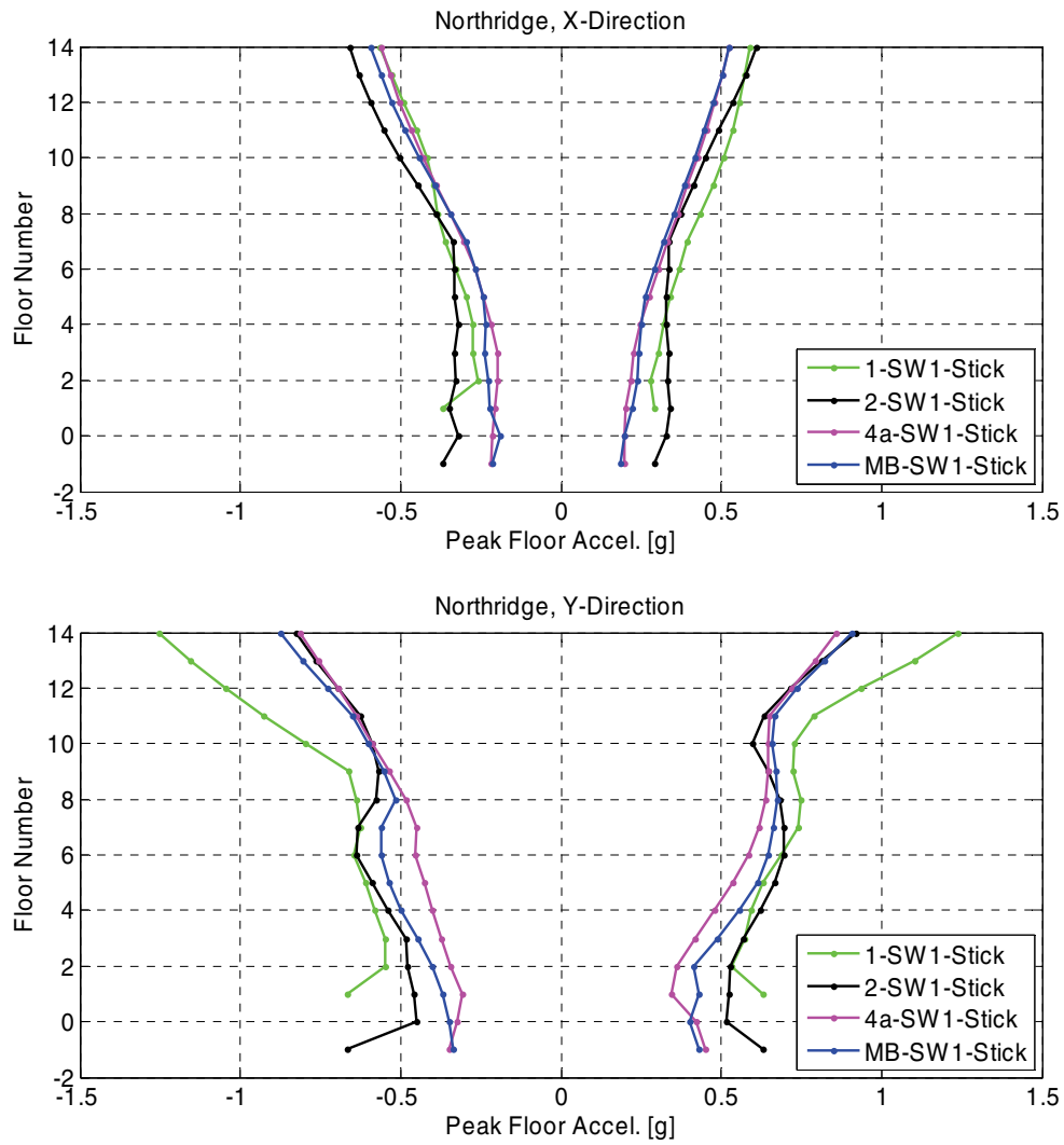
Figure B-35 Comparison of peak floor acceleration envelopes for the SW1 stick Models 1, 2, 4a, and MB.
