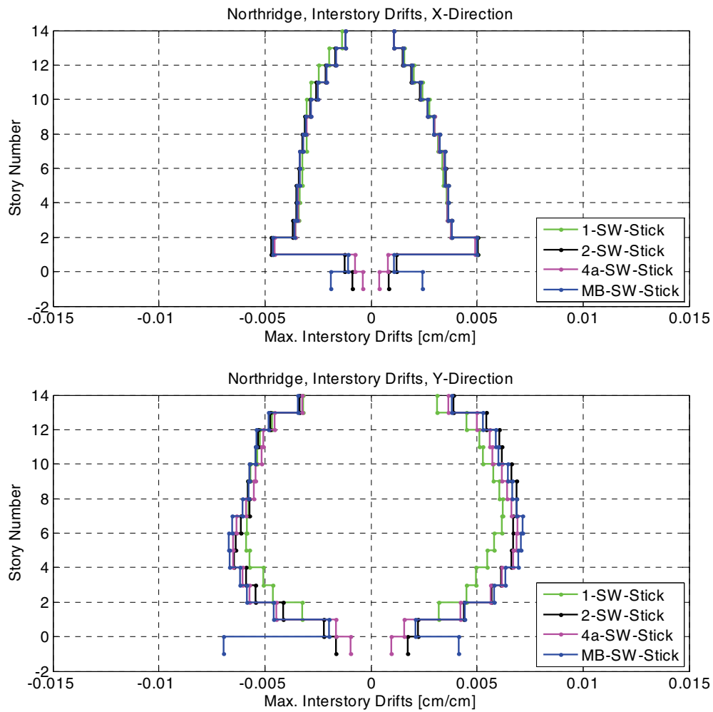
Figure B-29 Comparison of maximum story drift envelopes for the SW stick Models 1, 2, 4a, and MB.
