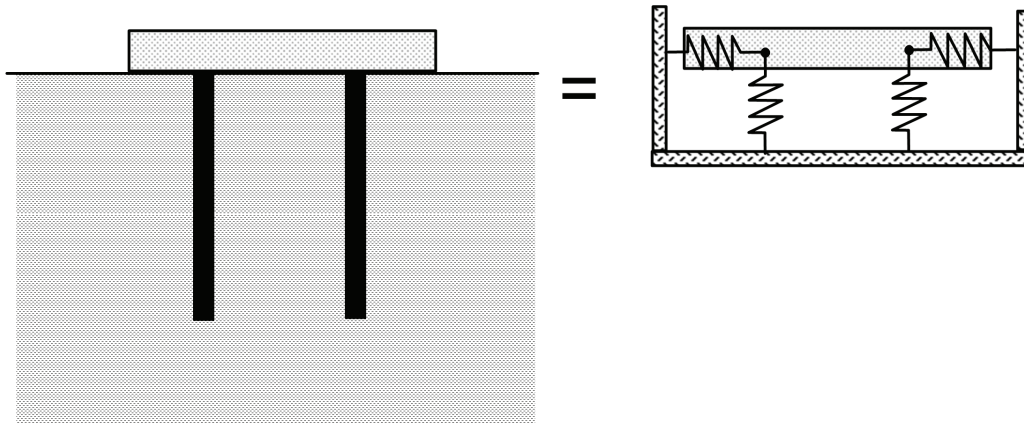
Figure 2-9 Schematic illustration showing replacement of piles with equivalent springs for translational and vertical (rotational) impedance.
